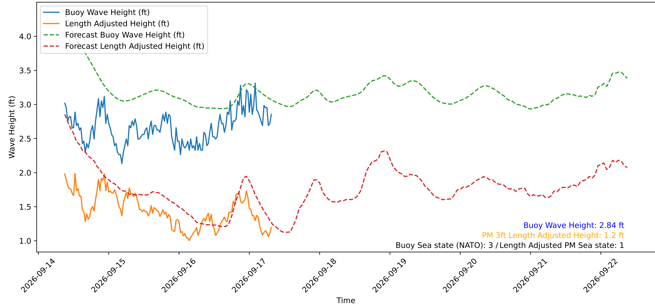
Wave Heights over Time for Green Beach at 2026-09-17 08:31:12
