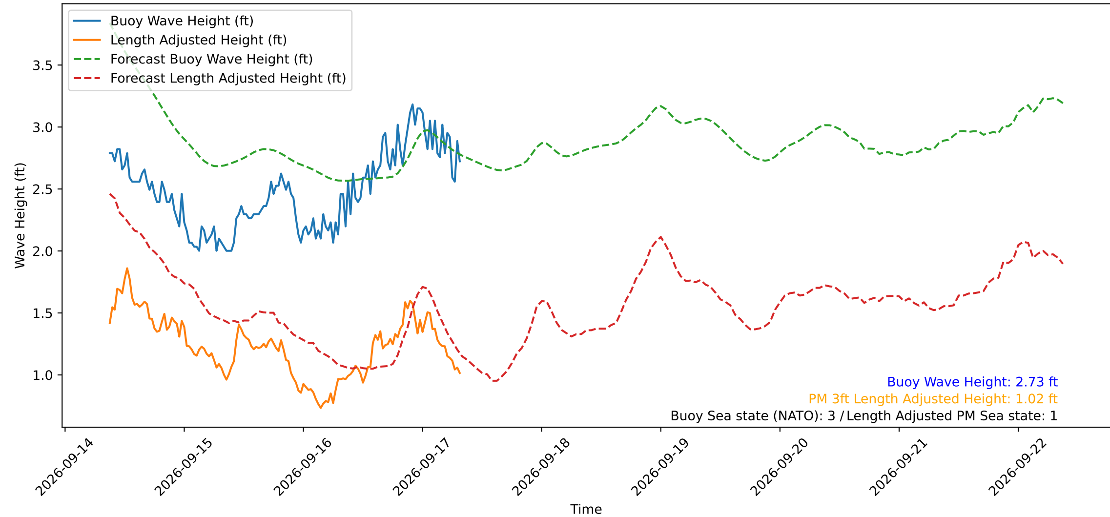
Wave Heights over Time for Red Beach at 2026-09-17 08:30:49
