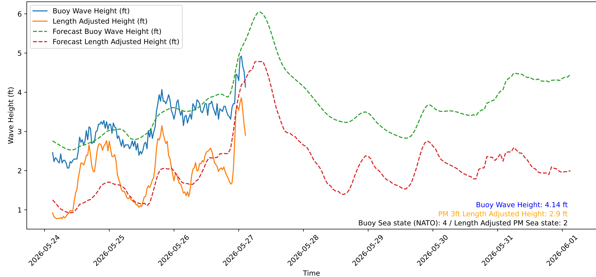
Wave Heights over Time for Green Beach at 2026-05-27 03:11:09
