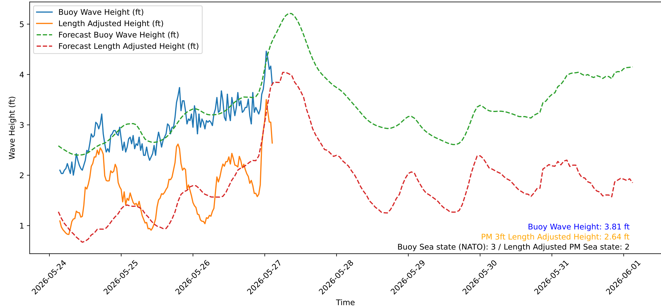
Wave Heights over Time for Red Beach at 2026-05-27 03:10:46
