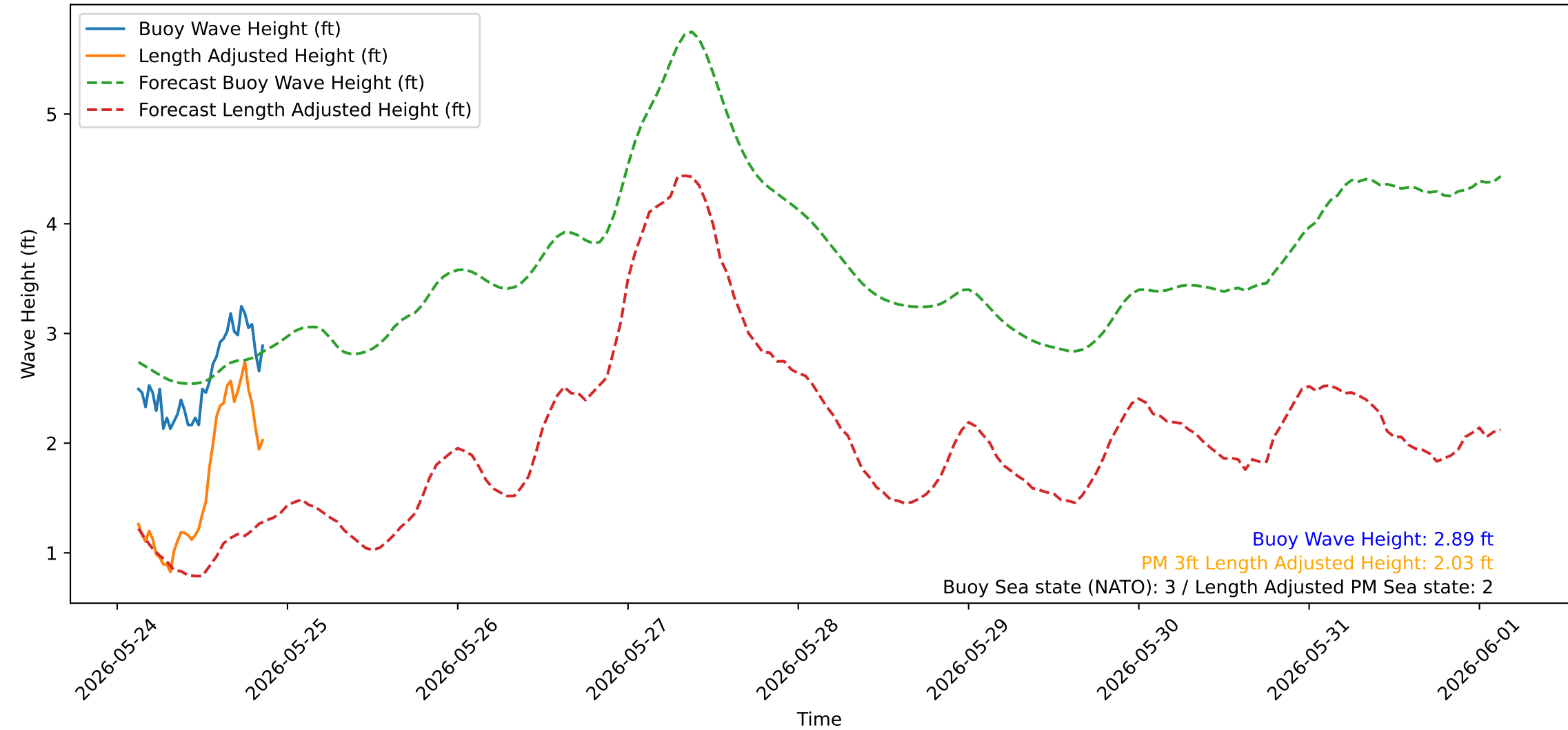
Wave Heights over Time for Oceanside Harbor at 2026-05-27 03:10:26
