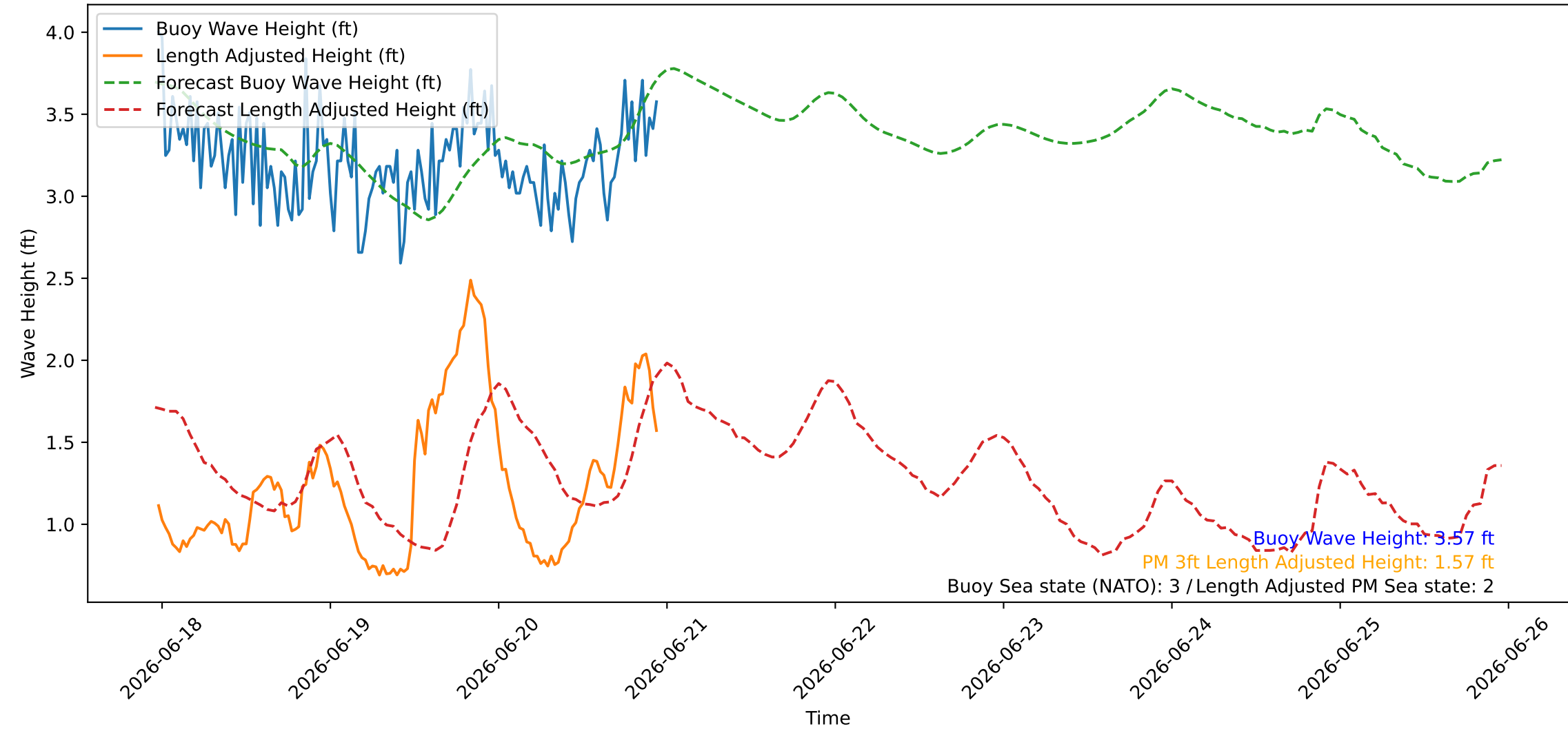
Wave Heights over Time for Red Beach at 2026-06-20 23:20:47
