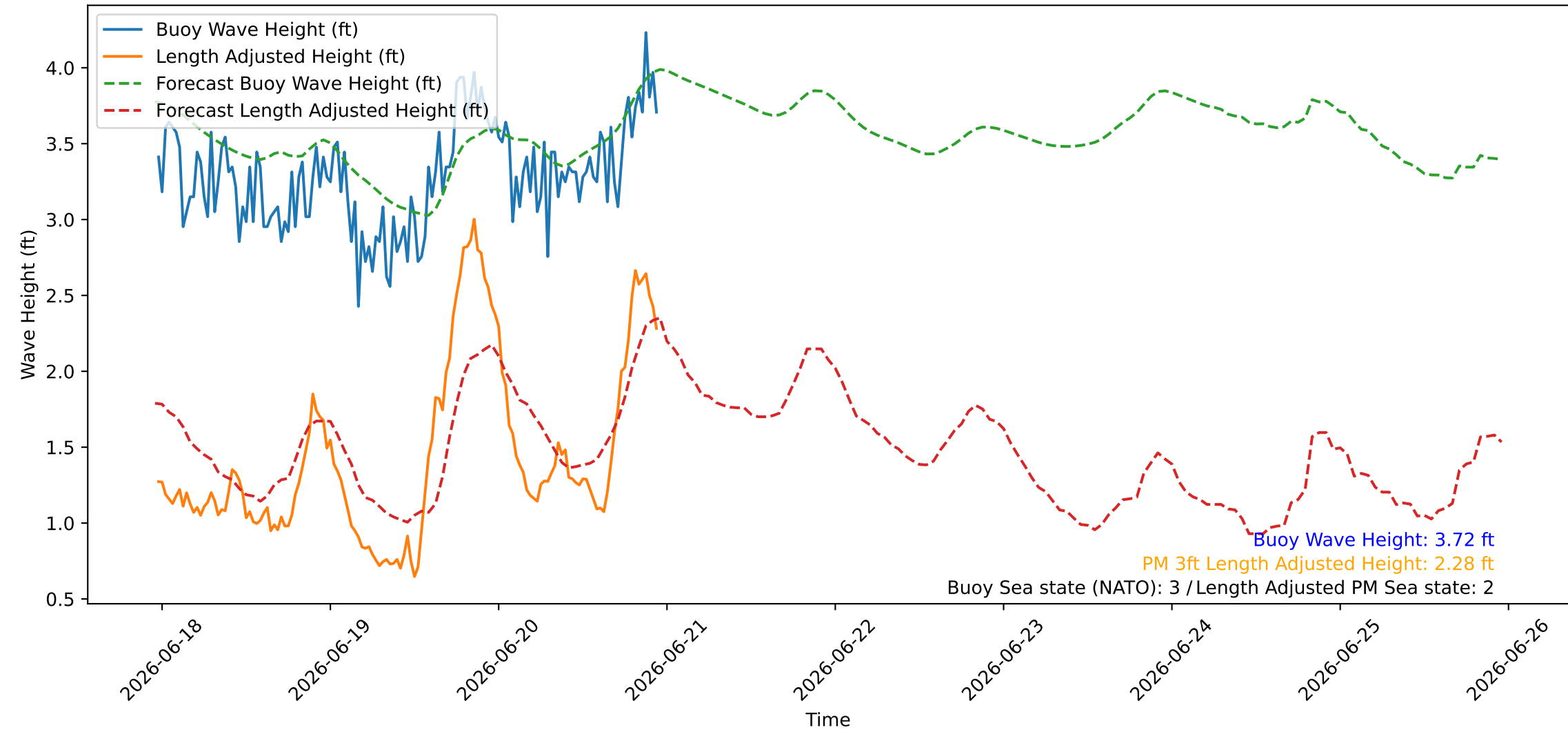
Wave Heights over Time for Green Beach at 2026-06-20 23:21:10
