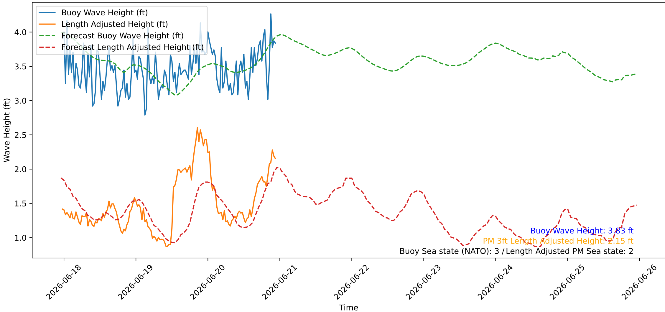
Wave Heights over Time for Oceanside Harbor at 2026-06-20 23:20:26
