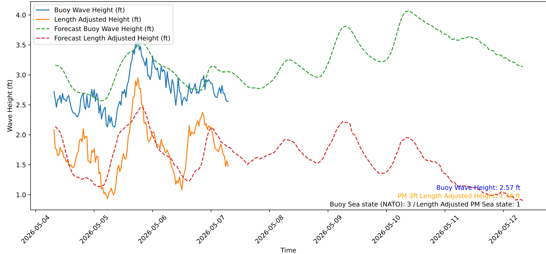
Wave Heights over Time for Green Beach at 2026-05-07 07:41:13
