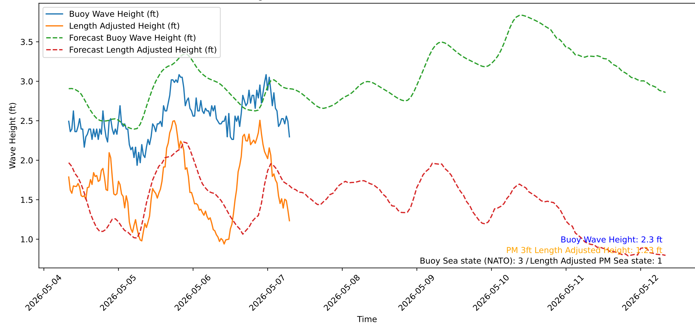
Wave Heights over Time for Red Beach at 2026-05-07 07:40:50
