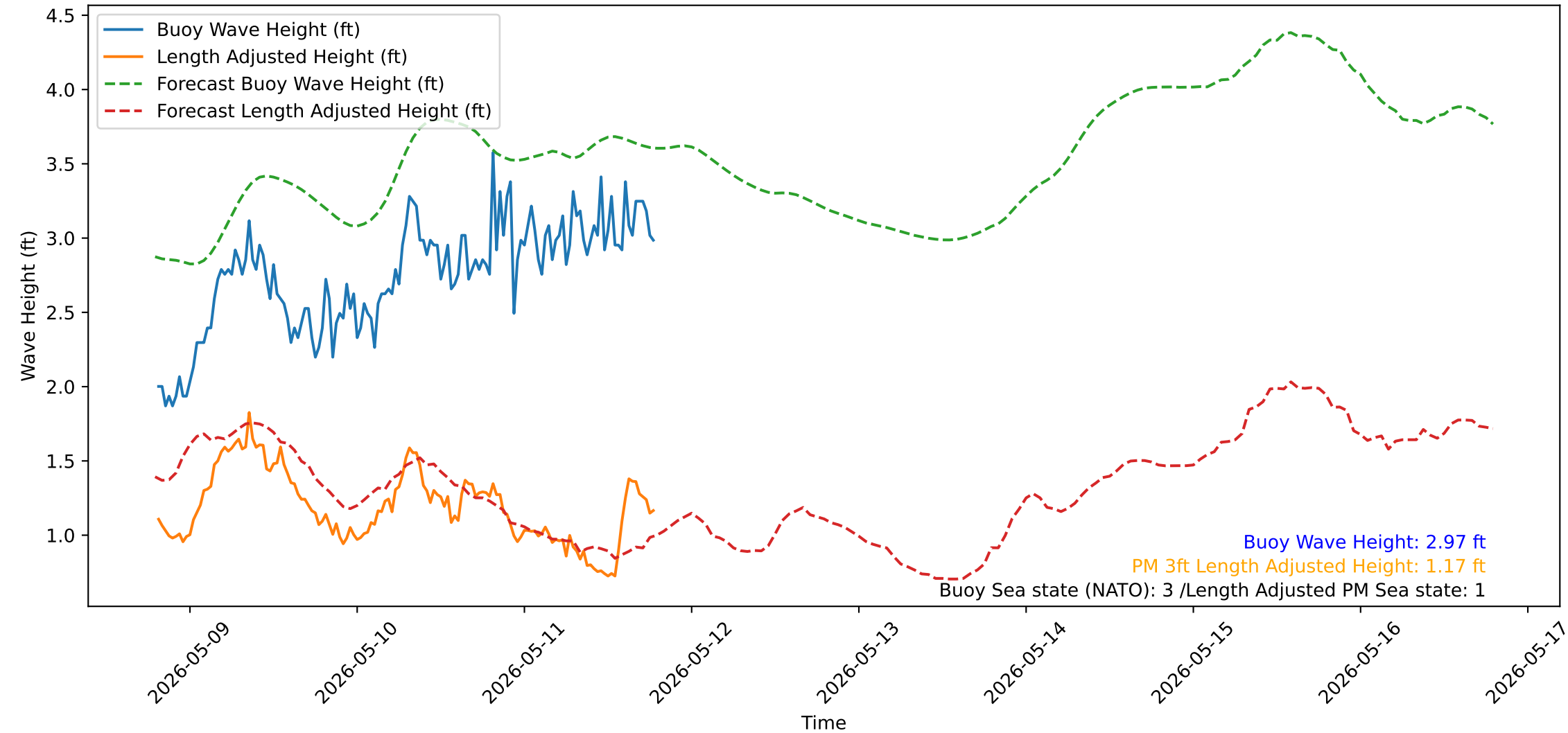
Wave Heights over Time for Oceanside Harbor at 2026-05-11 19:20:31
