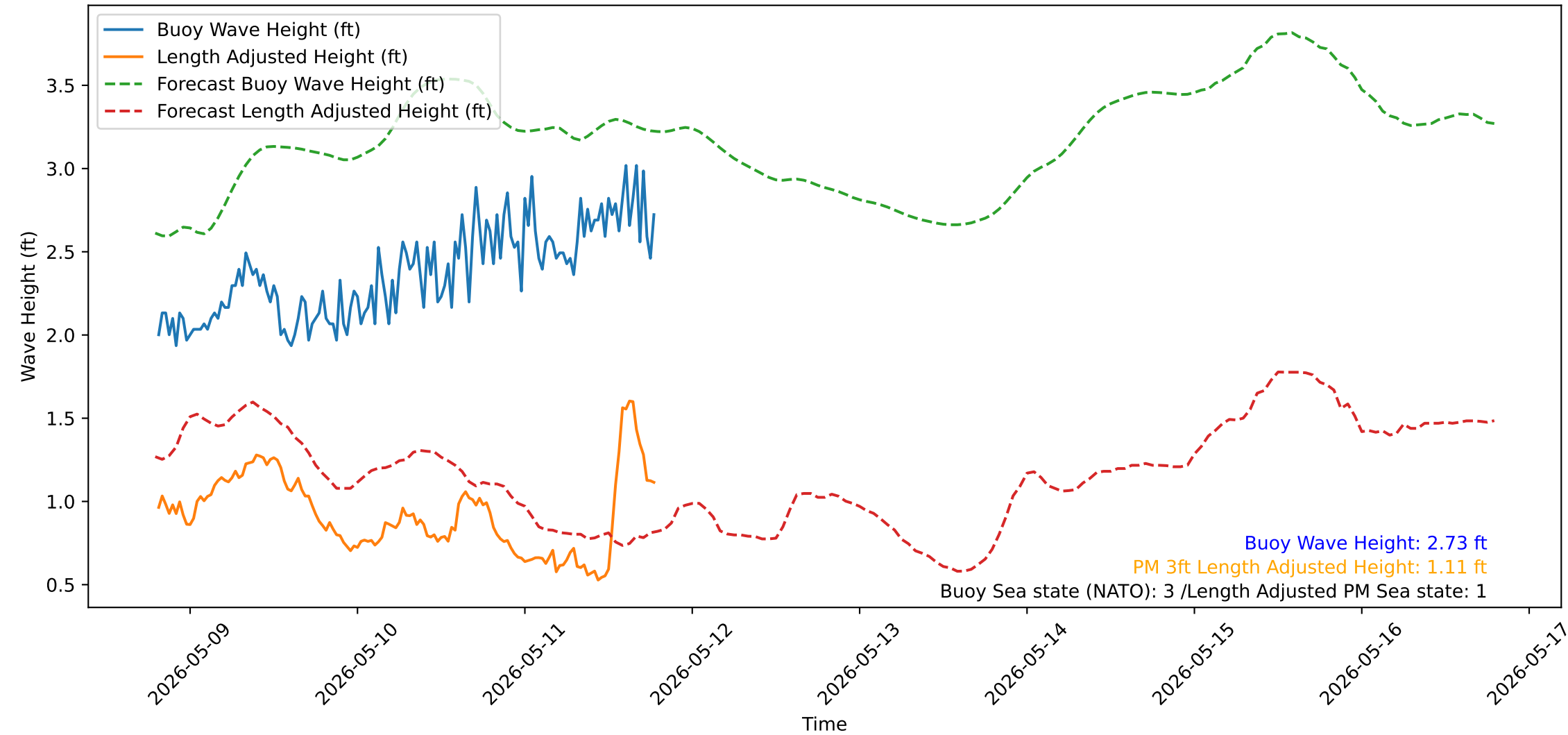
Wave Heights over Time for Red Beach at 2026-05-11 19:20:51
