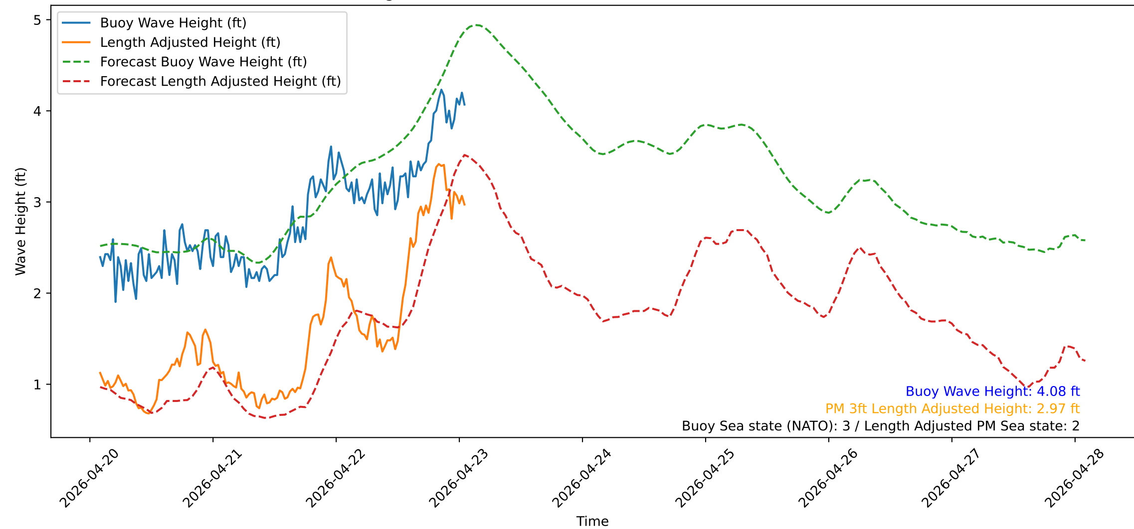
Wave Heights over Time for Oceanside Harbor at 2026-04-23 02:00:31
