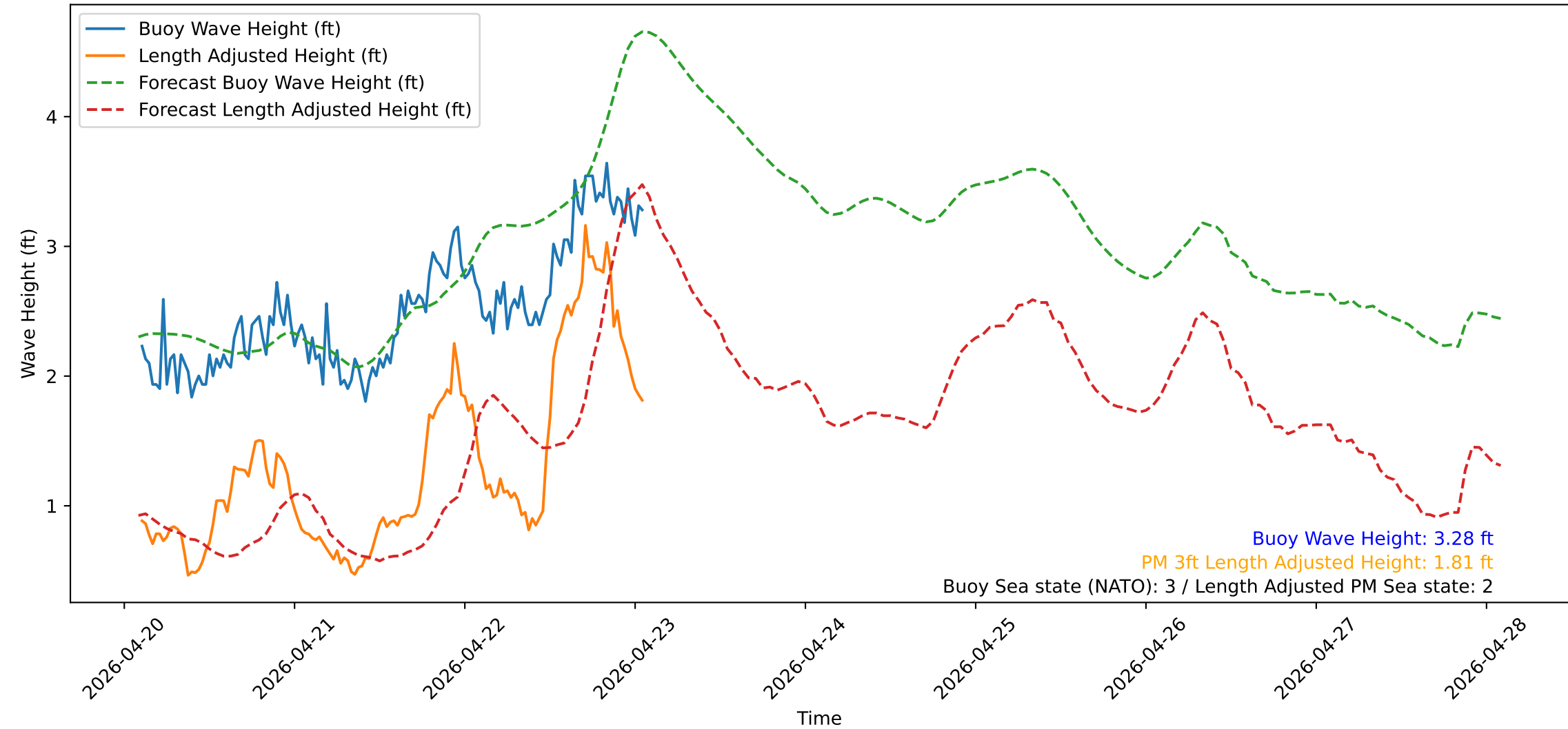
Wave Heights over Time for Red Beach at 2026-04-23 02:00:49
