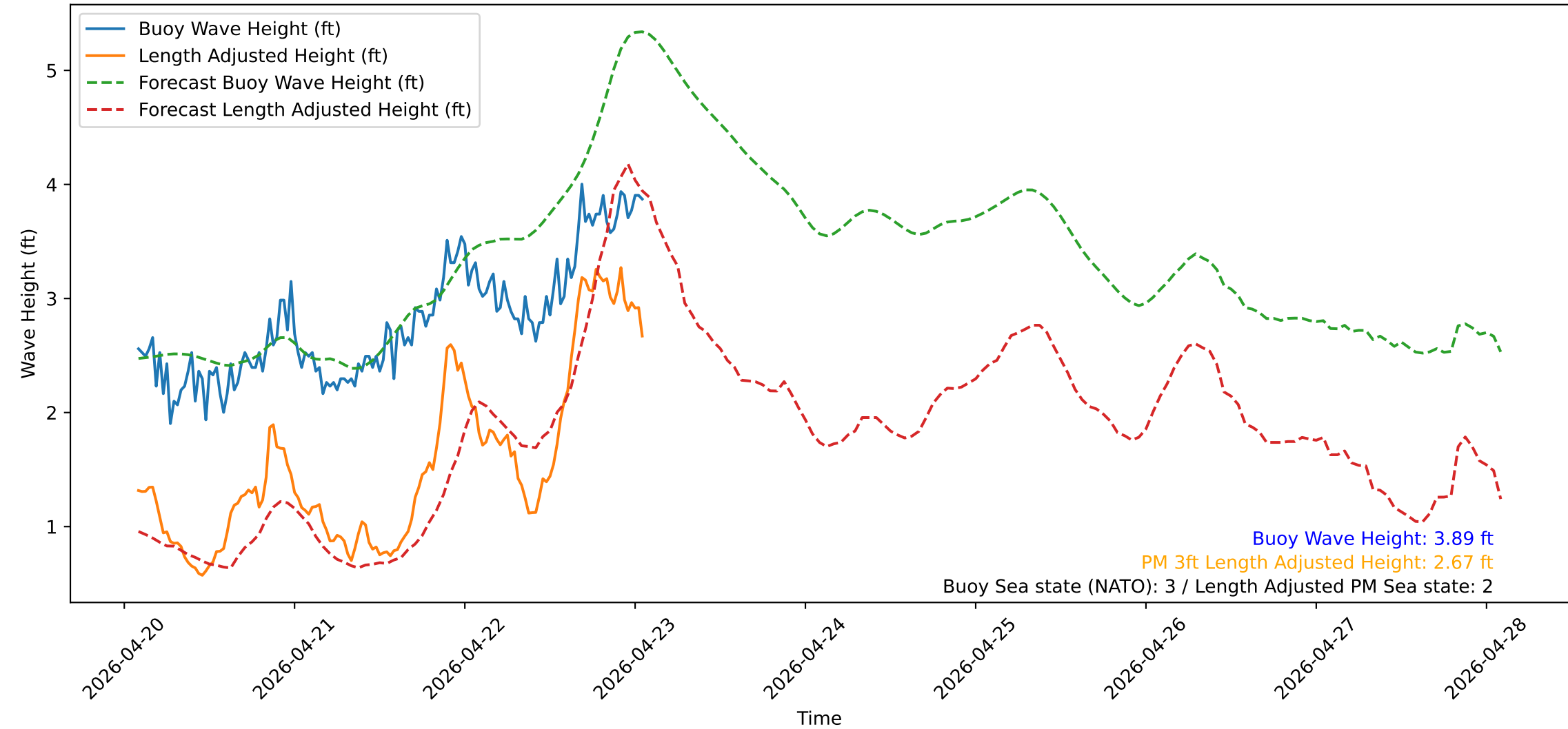
Wave Heights over Time for Green Beach at 2026-04-23 02:01:11
