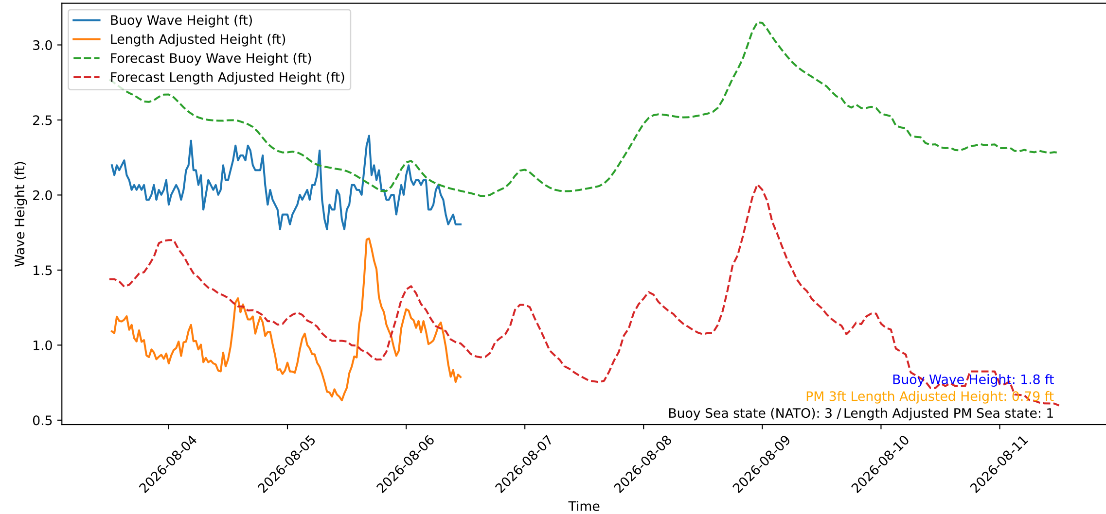
Wave Heights over Time for Red Beach at 2026-08-06 12:10:46
