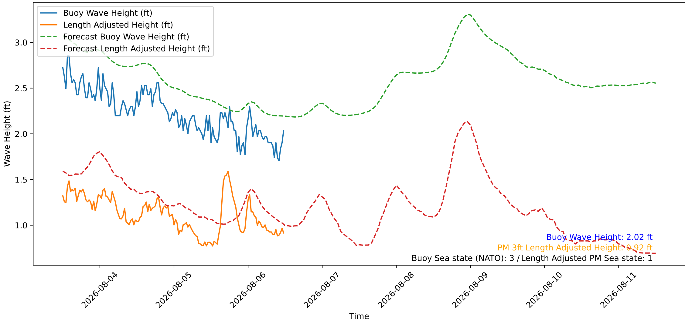
Wave Heights over Time for Oceanside Harbor at 2026-08-06 12:10:27
