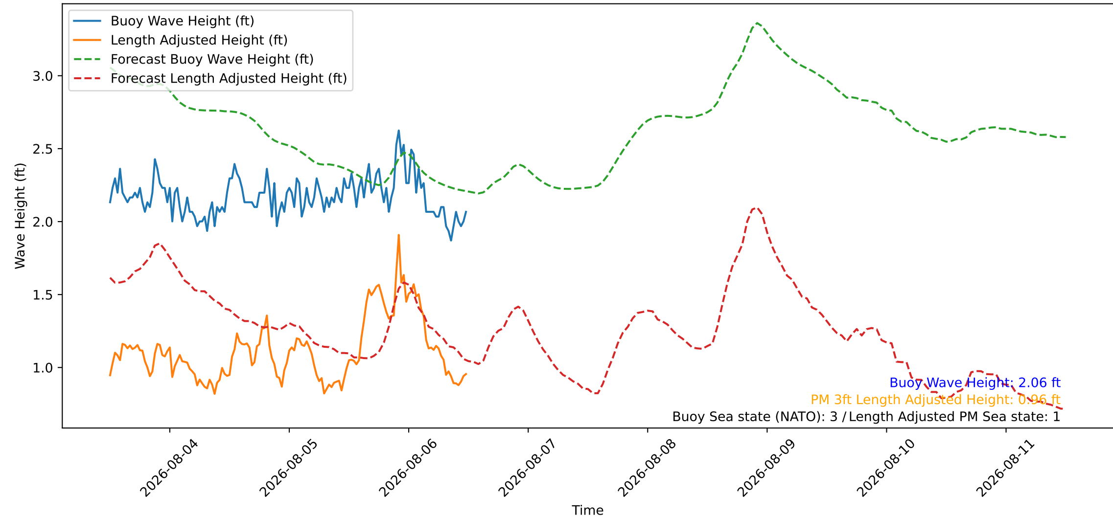
Wave Heights over Time for Green Beach at 2026-08-06 12:11:08
