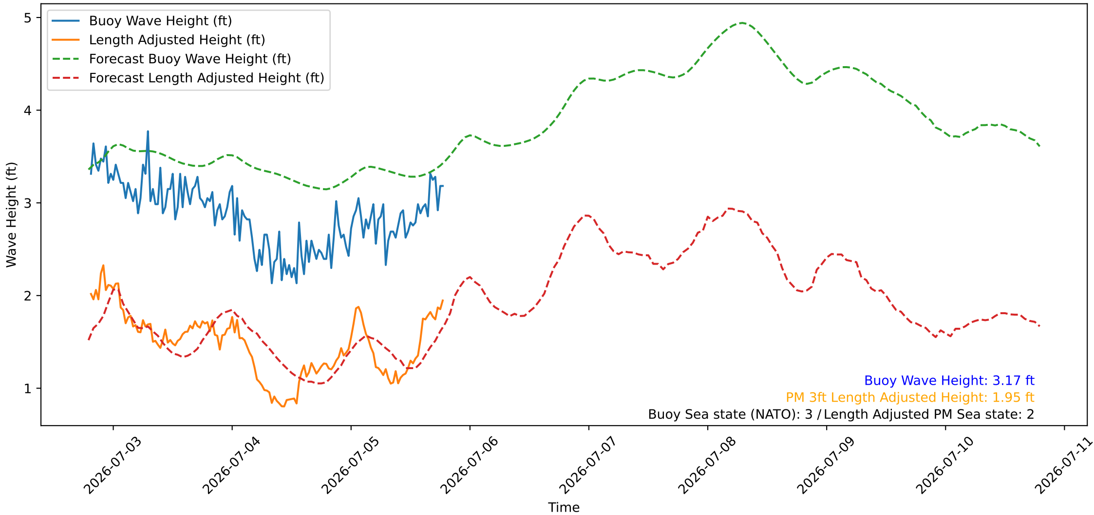
Wave Heights over Time for Oceanside Harbor at 2026-07-05 19:20:26
