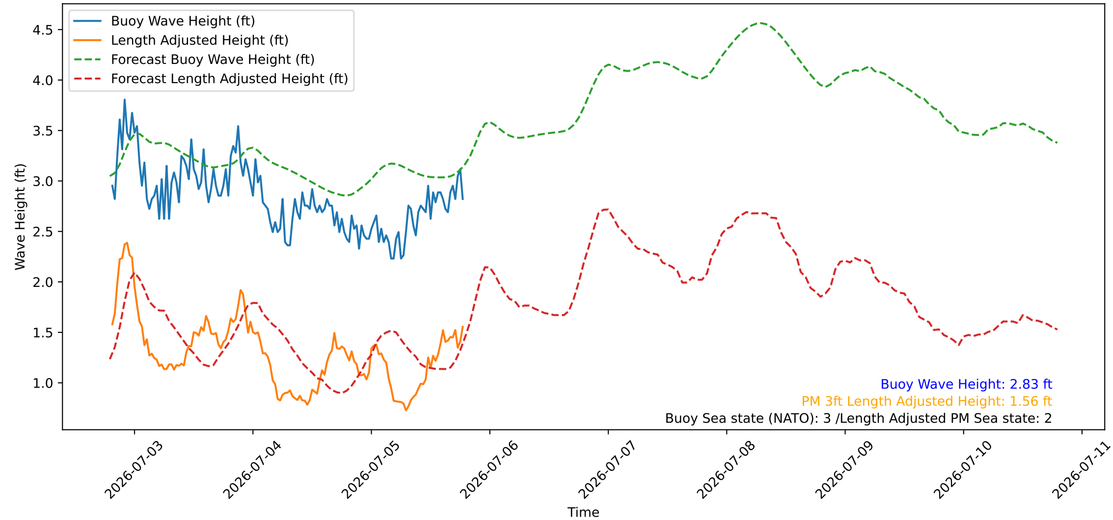
Wave Heights over Time for Red Beach at 2026-07-05 19:20:47
