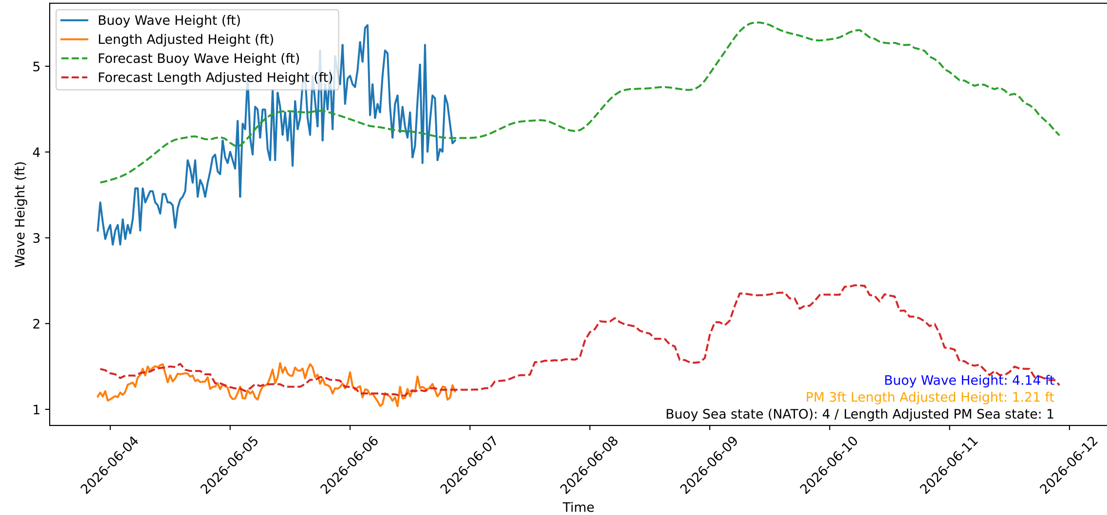
Wave Heights over Time for Oceanside Harbor at 2026-06-06 21:40:26
