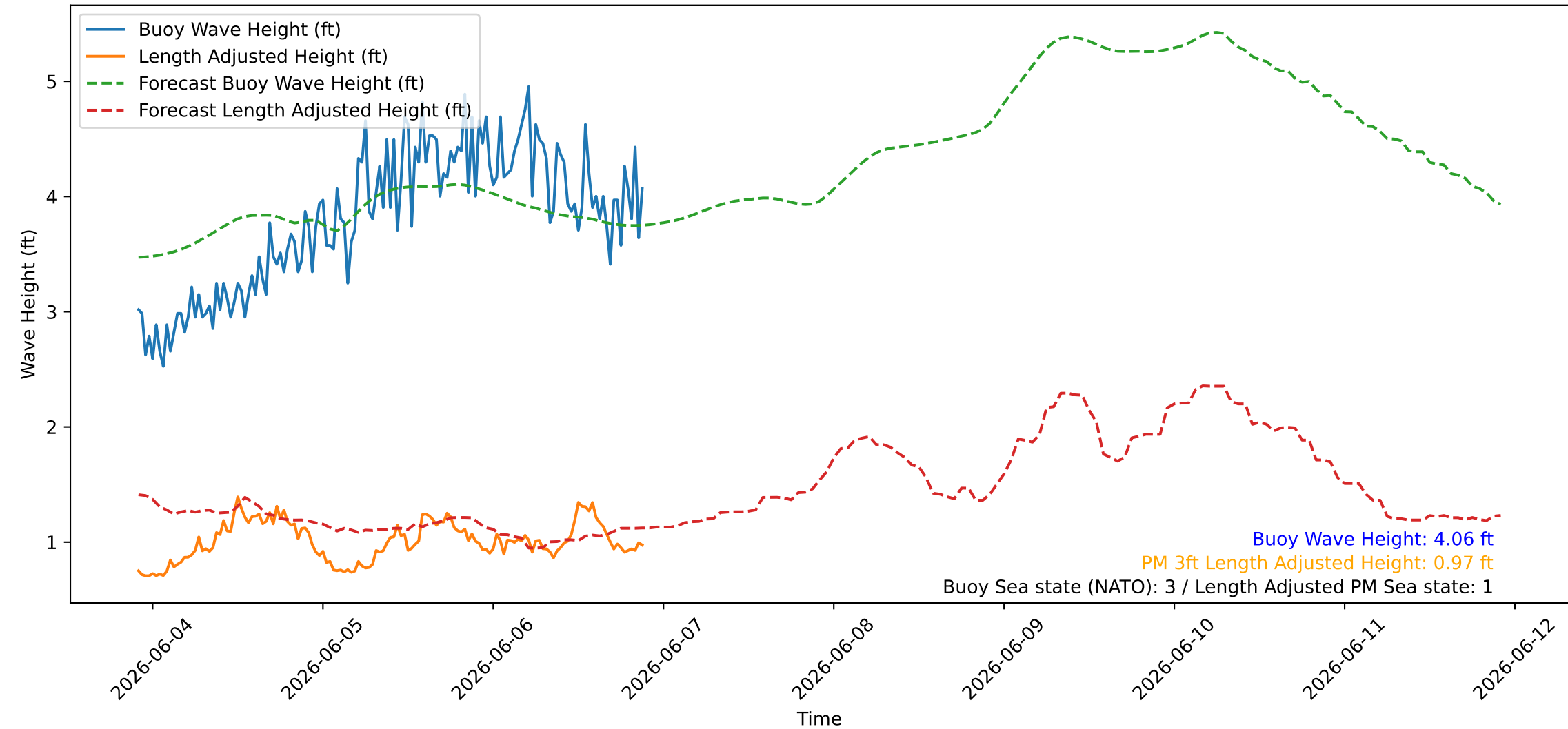
Wave Heights over Time for Red Beach at 2026-06-06 21:40:45
