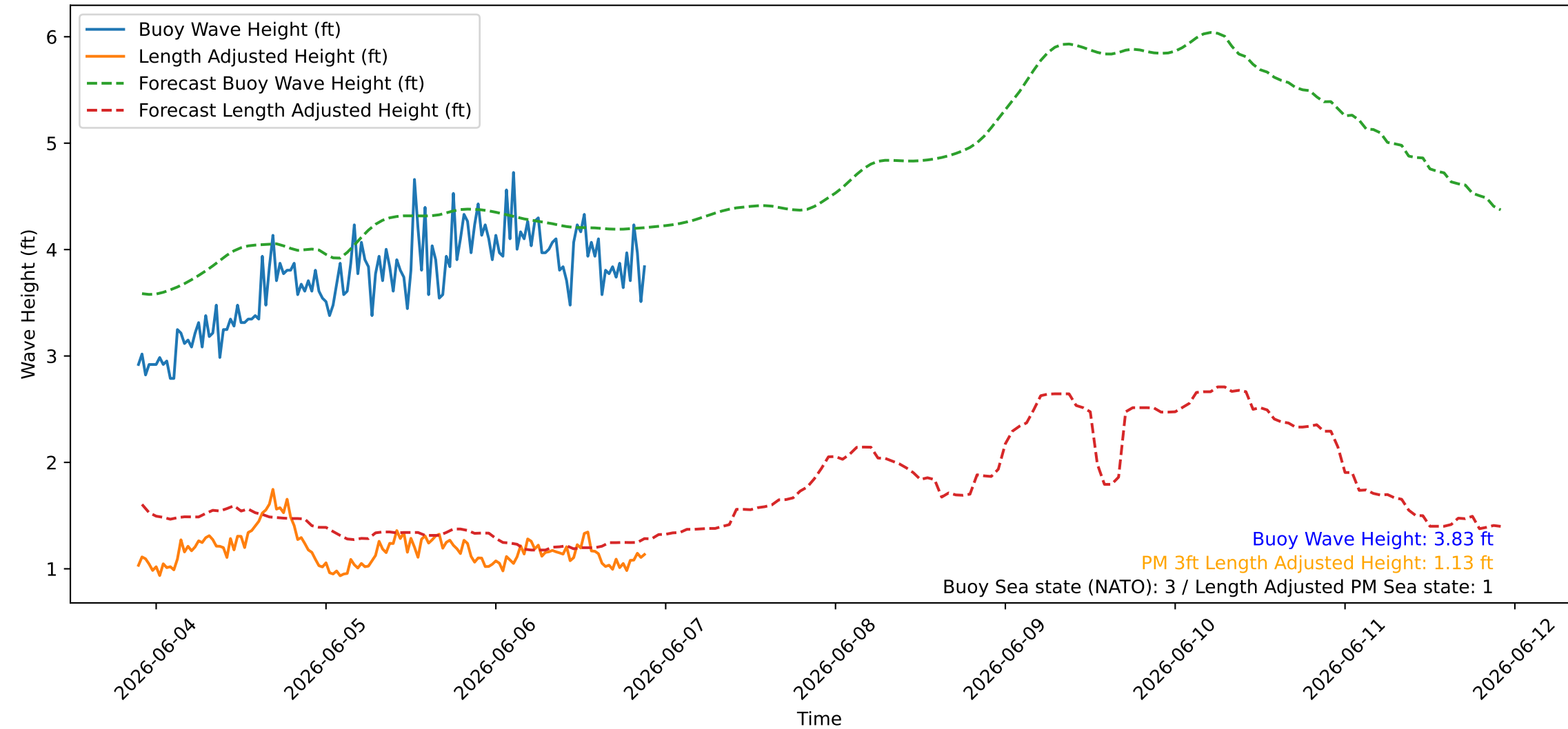
Wave Heights over Time for Green Beach at 2026-06-06 21:41:08
