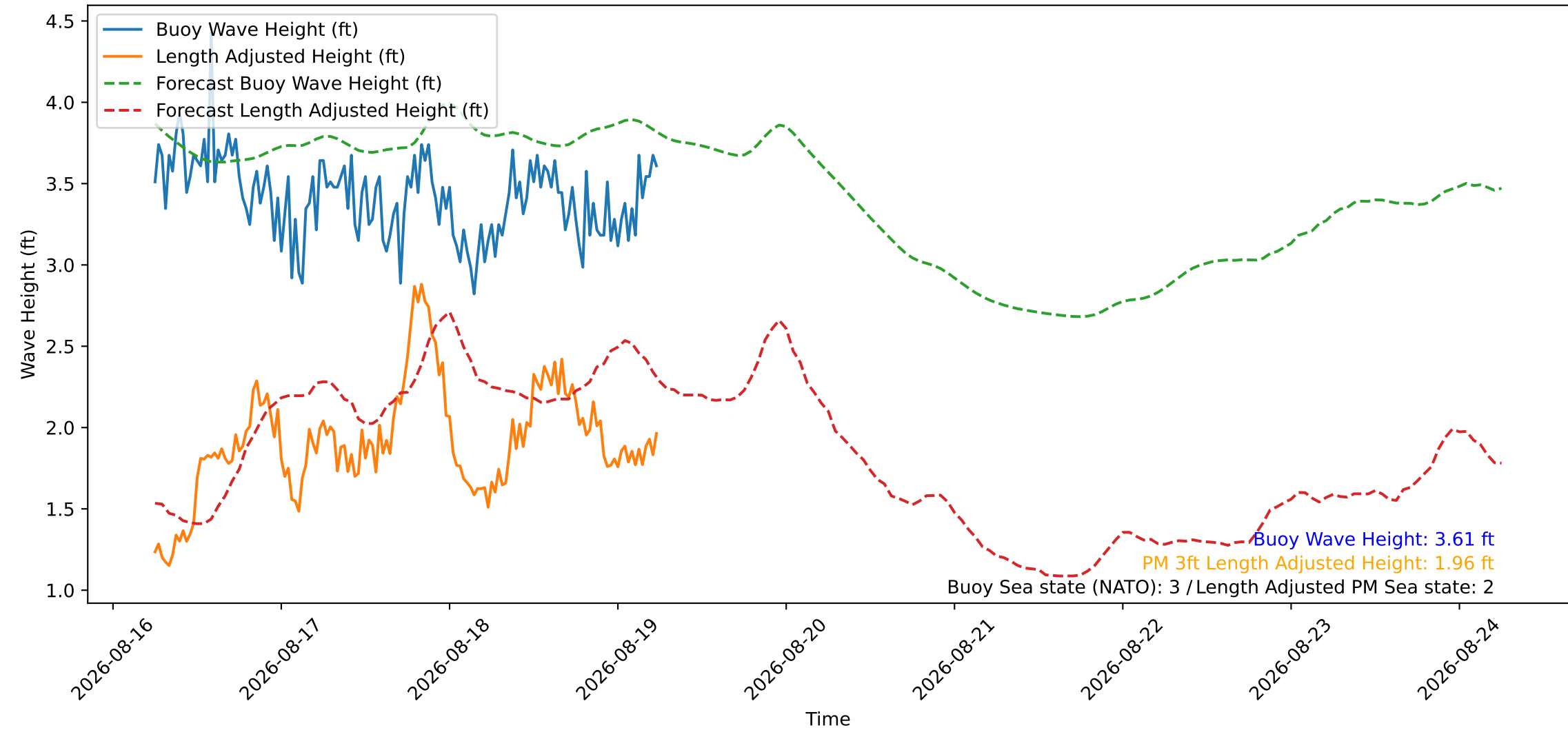
Wave Heights over Time for Oceanside Harbor at 2026-08-19 06:00:27
