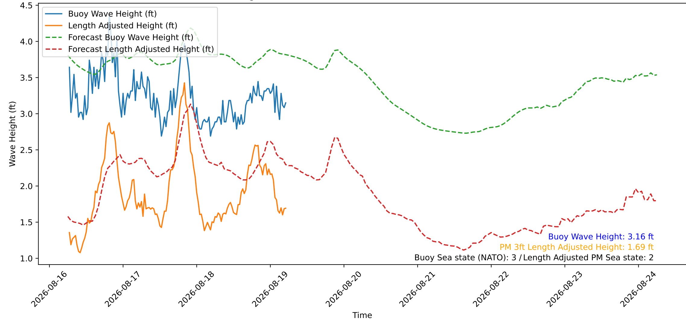
Wave Heights over Time for Green Beach at 2026-08-19 06:01:09
