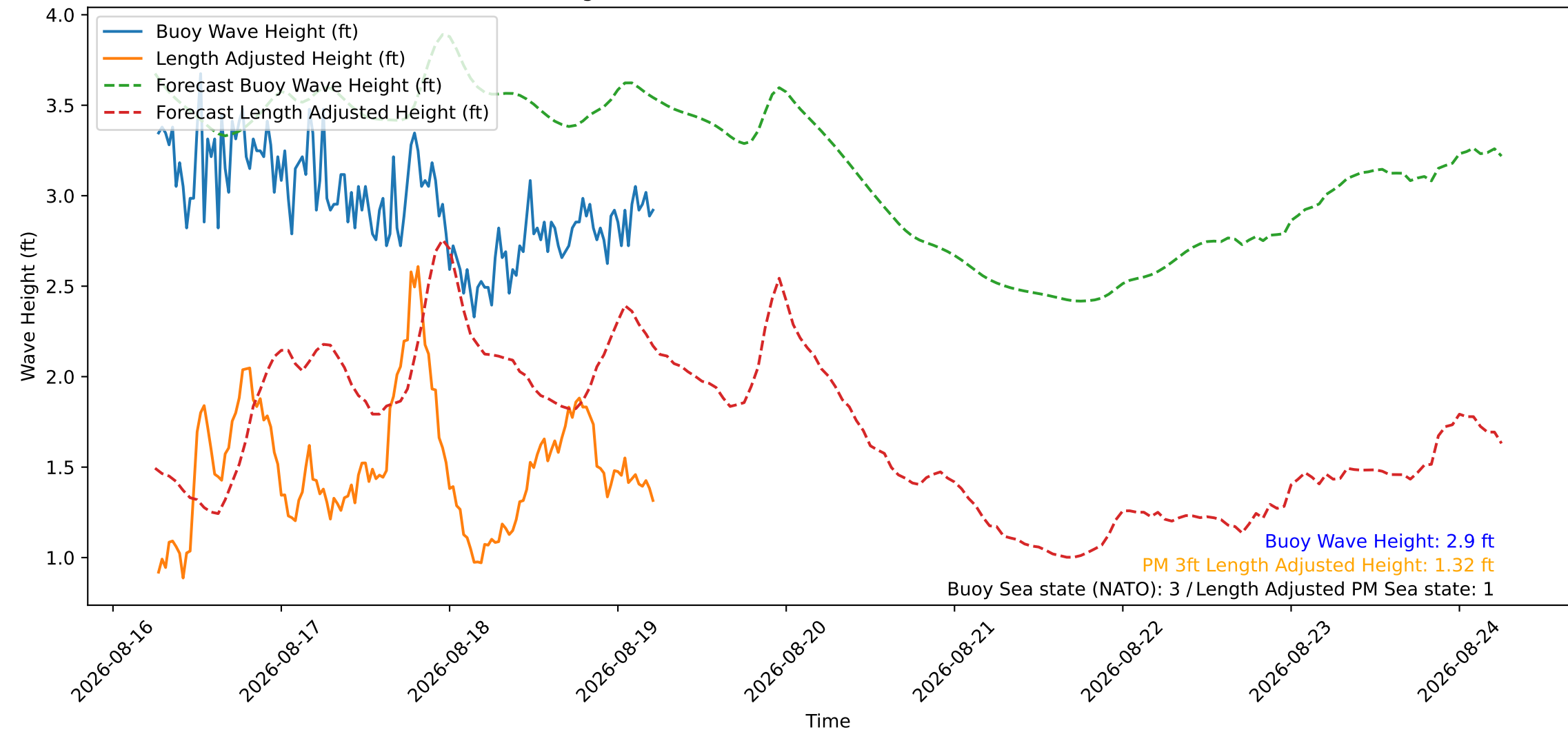
Wave Heights over Time for Red Beach at 2026-08-19 06:00:46
