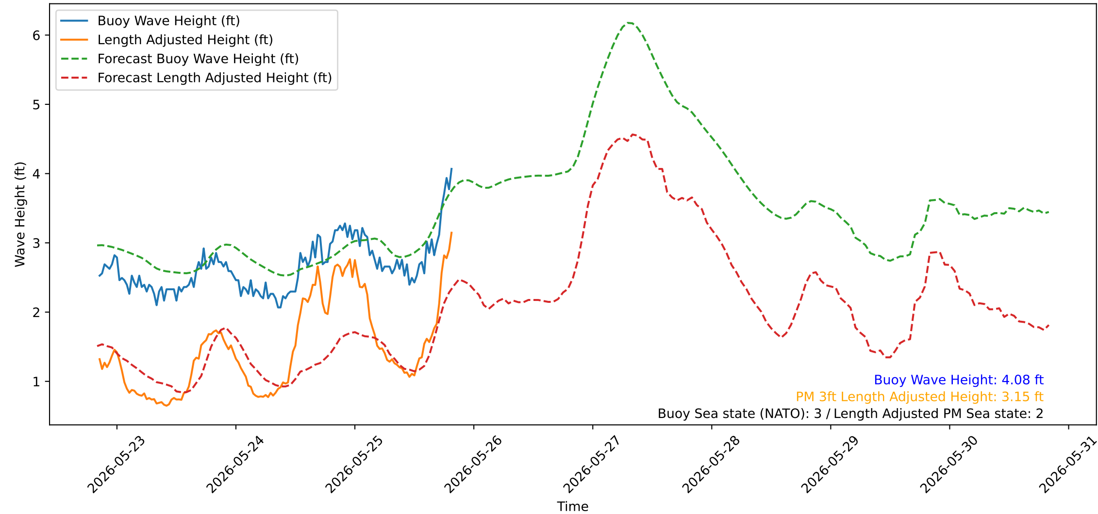
Wave Heights over Time for Green Beach at 2026-05-25 20:21:13
