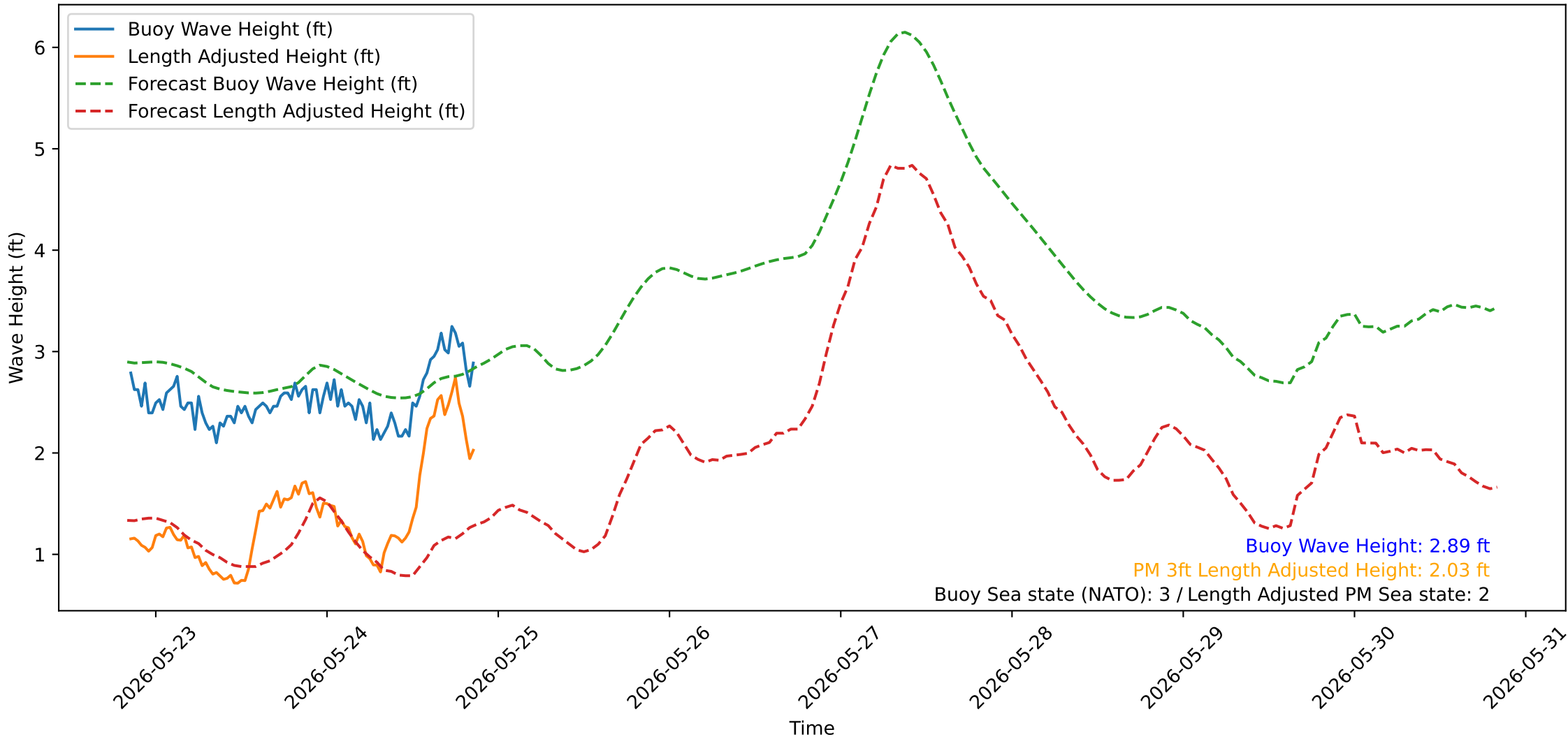
Wave Heights over Time for Oceanside Harbor at 2026-05-25 20:20:29
