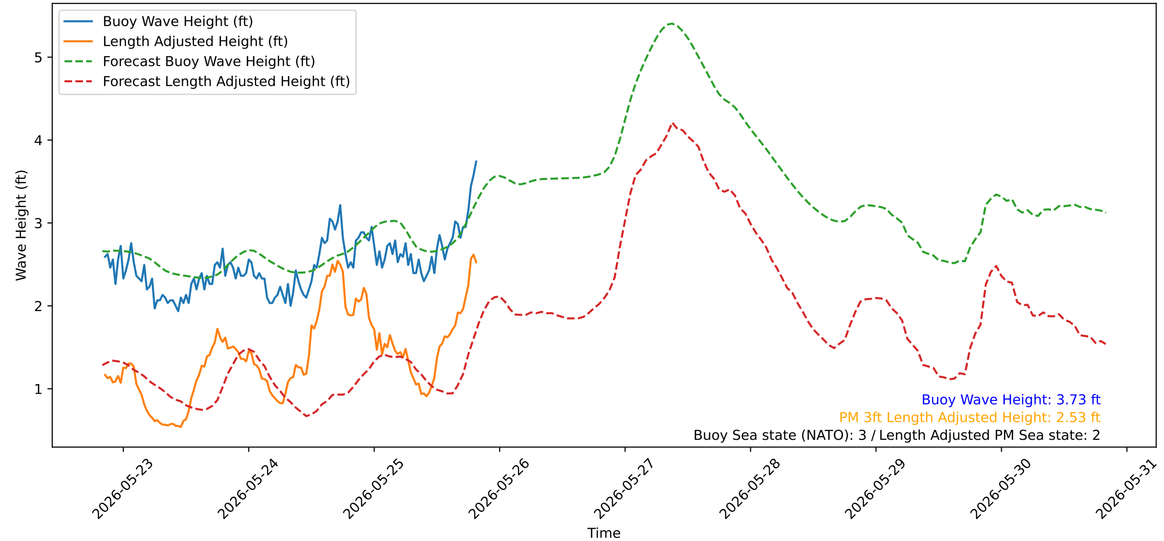
Wave Heights over Time for Red Beach at 2026-05-25 20:20:50
