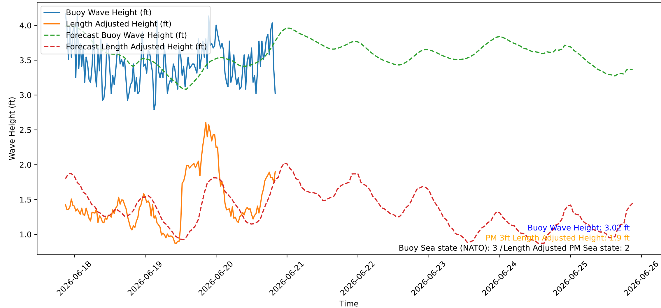
Wave Heights over Time for Oceanside Harbor at 2026-06-20 20:50:26
