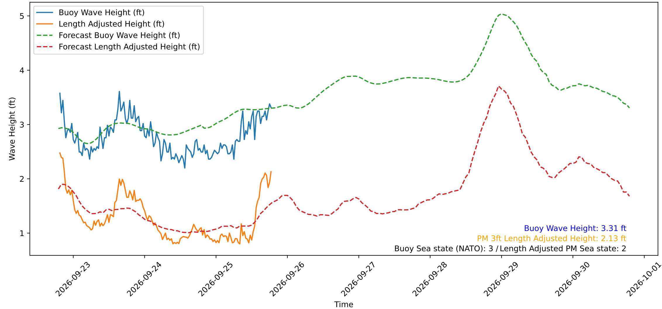
Wave Heights over Time for Oceanside Harbor at 2026-09-25 19:20:29
