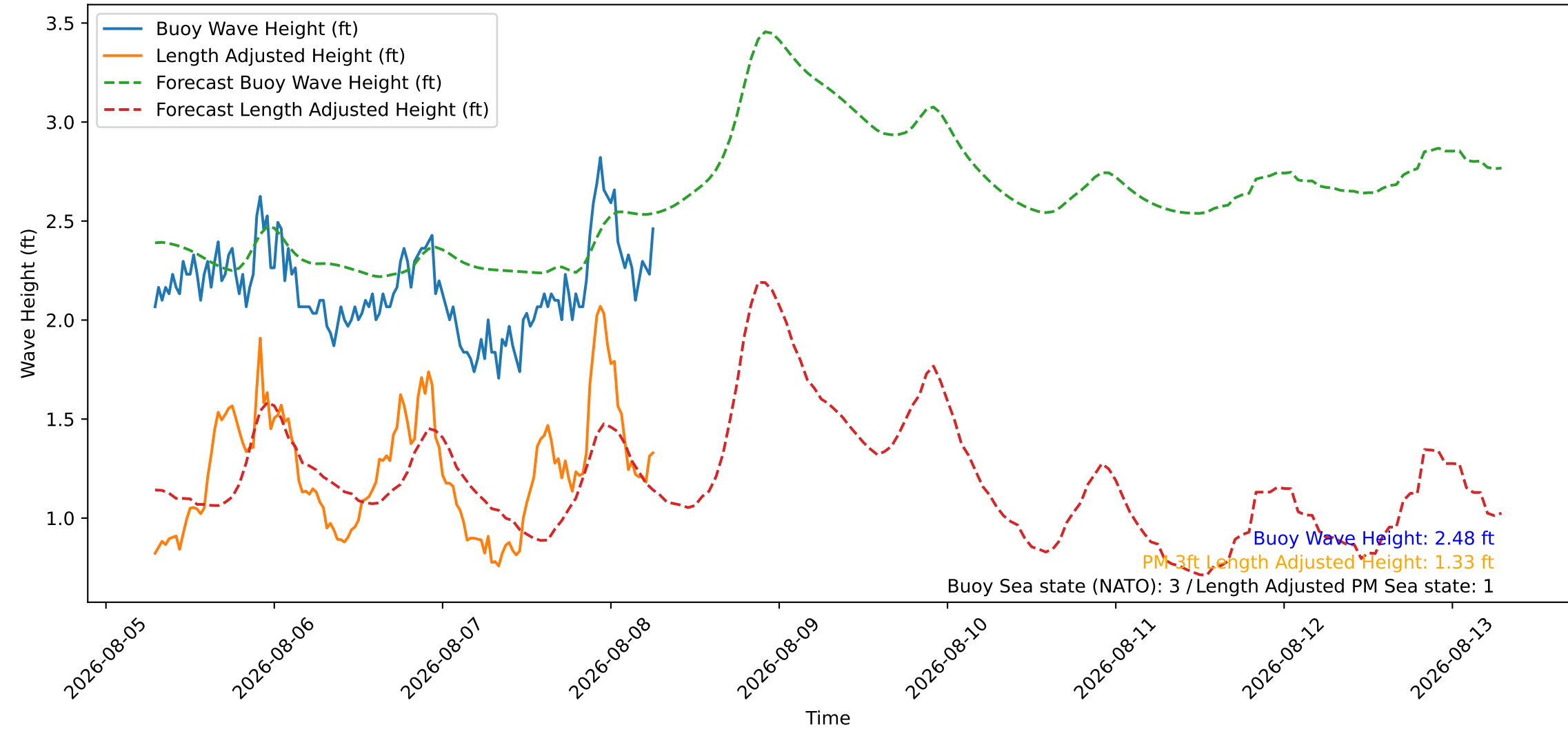
Wave Heights over Time for Green Beach at 2026-08-08 06:51:10
