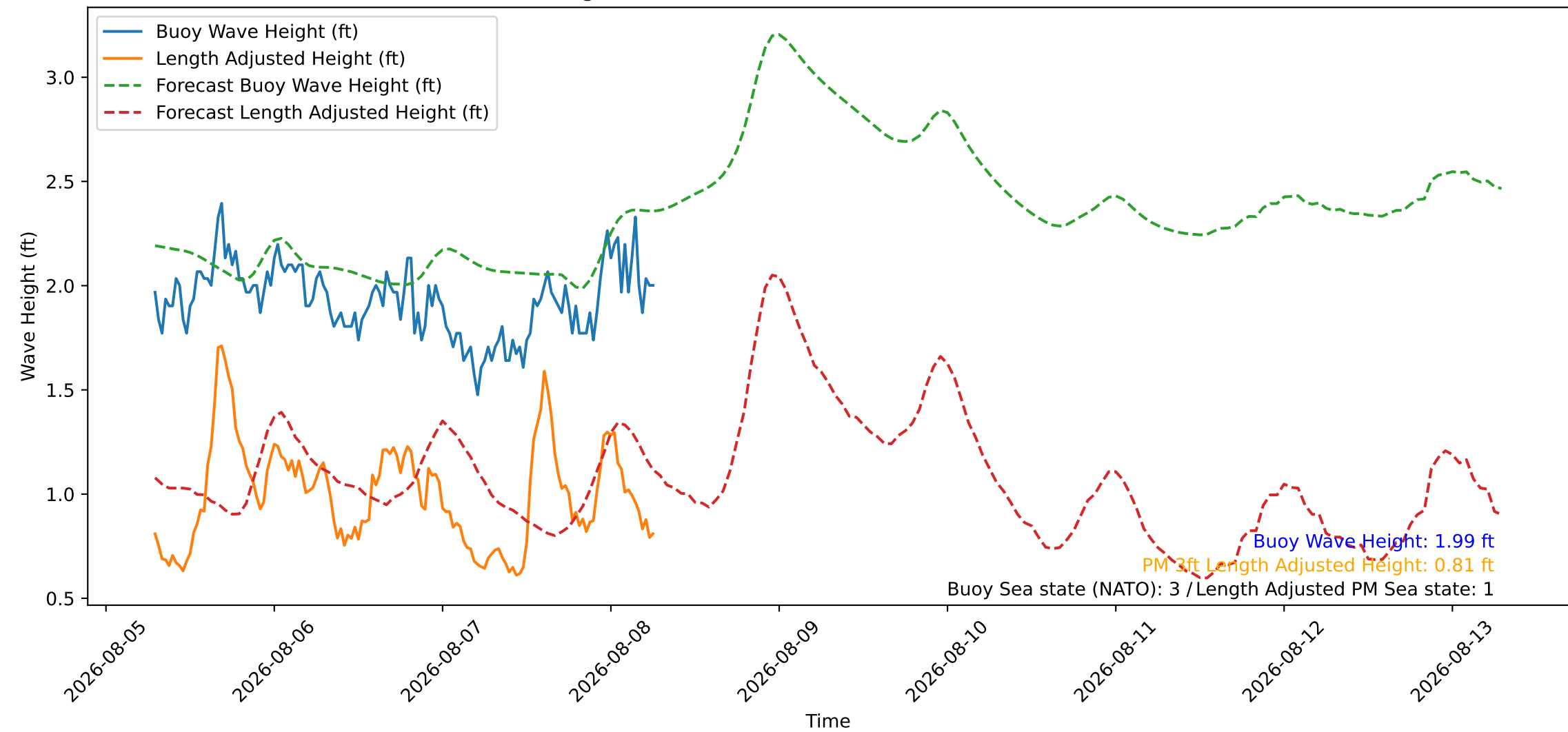
Wave Heights over Time for Red Beach at 2026-08-08 06:50:48
