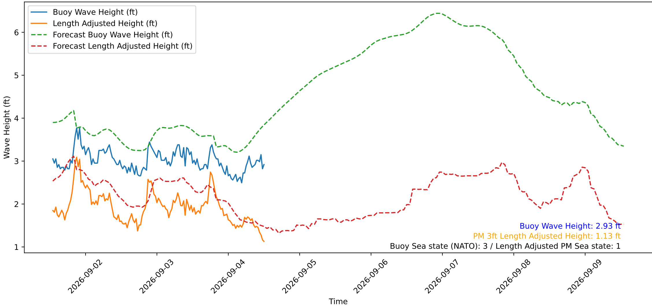
Wave Heights over Time for Green Beach at 2026-09-04 12:51:16
