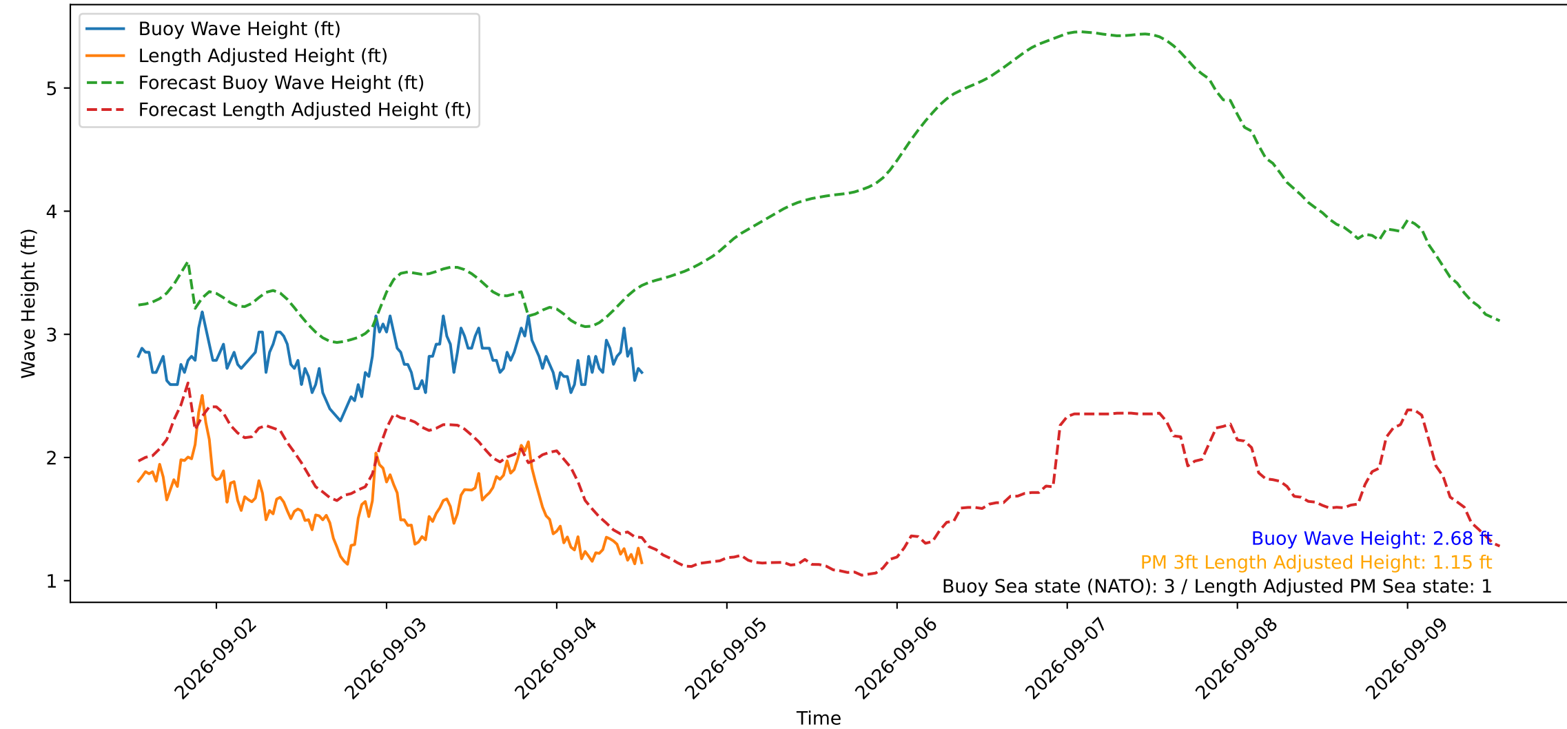
Wave Heights over Time for Red Beach at 2026-09-04 12:50:51
