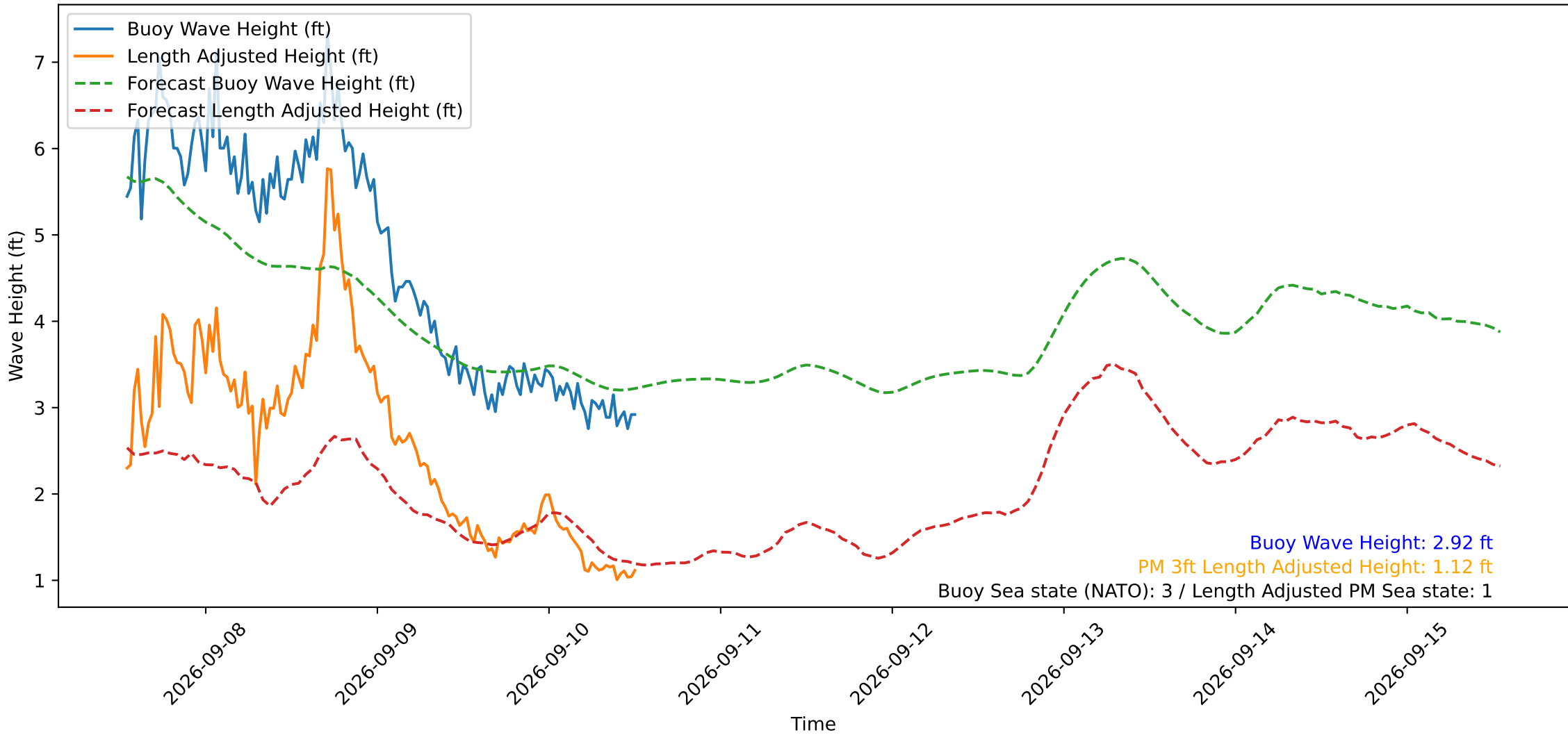
Wave Heights over Time for Oceanside Harbor at 2026-09-10 12:50:29
