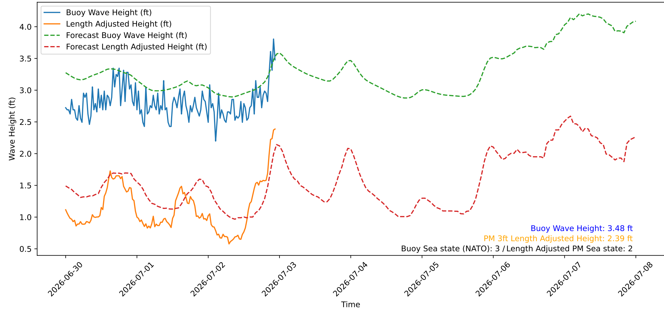
Wave Heights over Time for Red Beach at 2026-07-02 23:30:45
