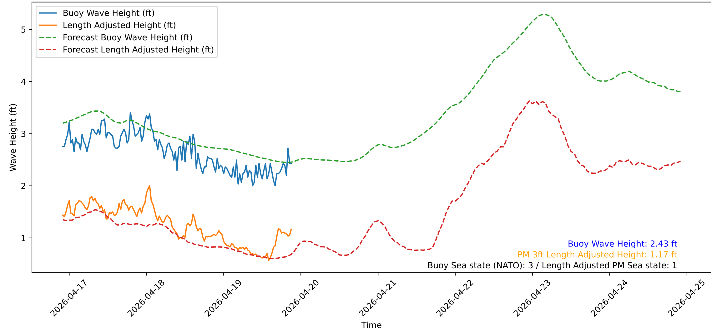
Wave Heights over Time for Oceanside Harbor at 2026-04-19 22:00:32
