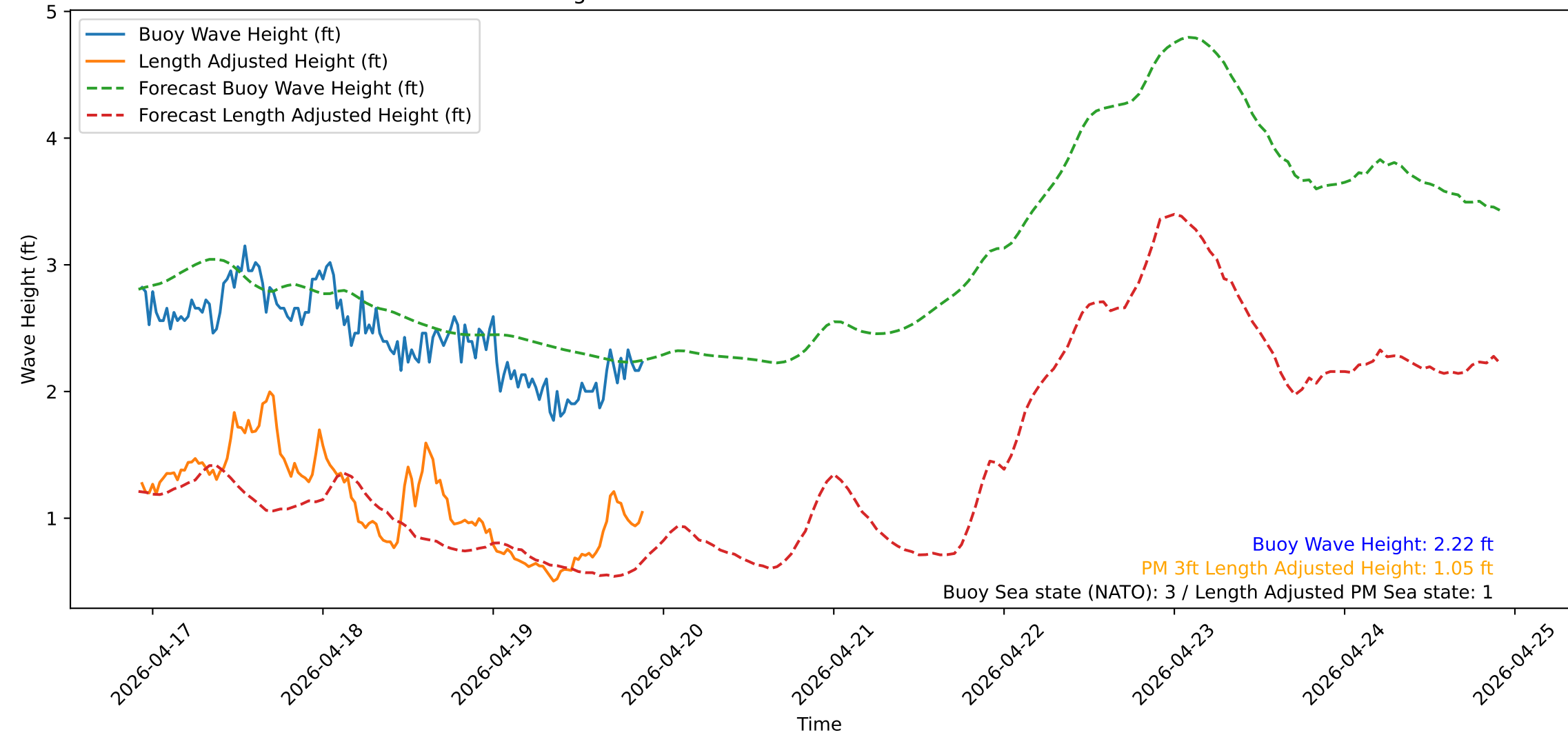
Wave Heights over Time for Red Beach at 2026-04-19 22:00:51
