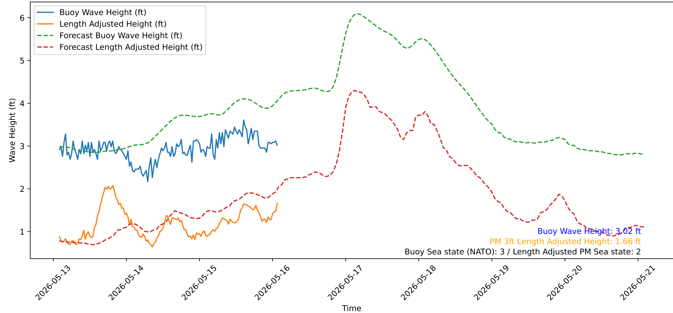
Wave Heights over Time for Oceanside Harbor at 2026-05-16 02:10:32
