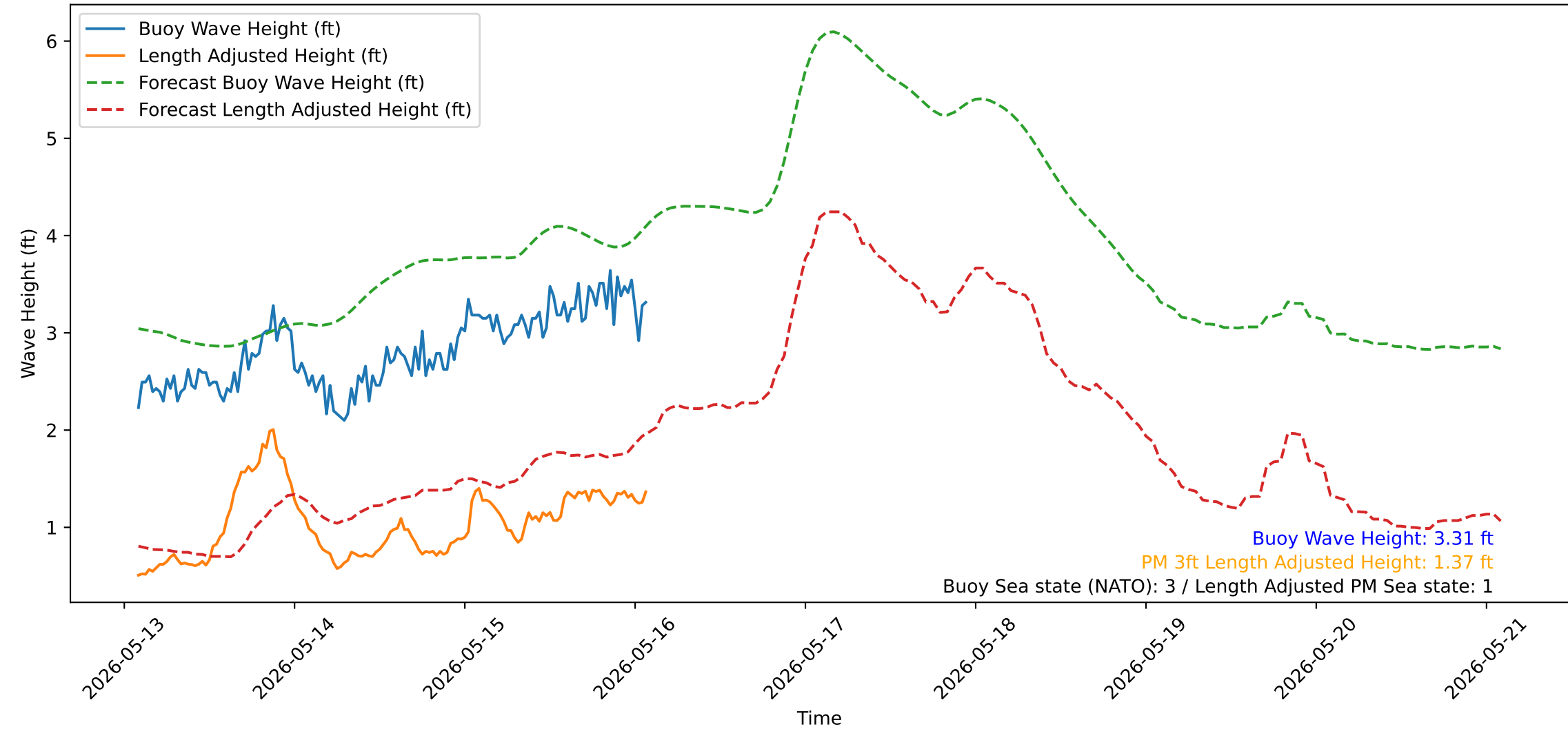
Wave Heights over Time for Green Beach at 2026-05-16 02:11:14
