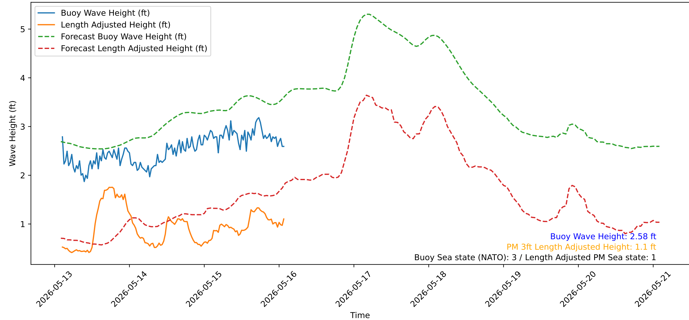
Wave Heights over Time for Red Beach at 2026-05-16 02:10:51
