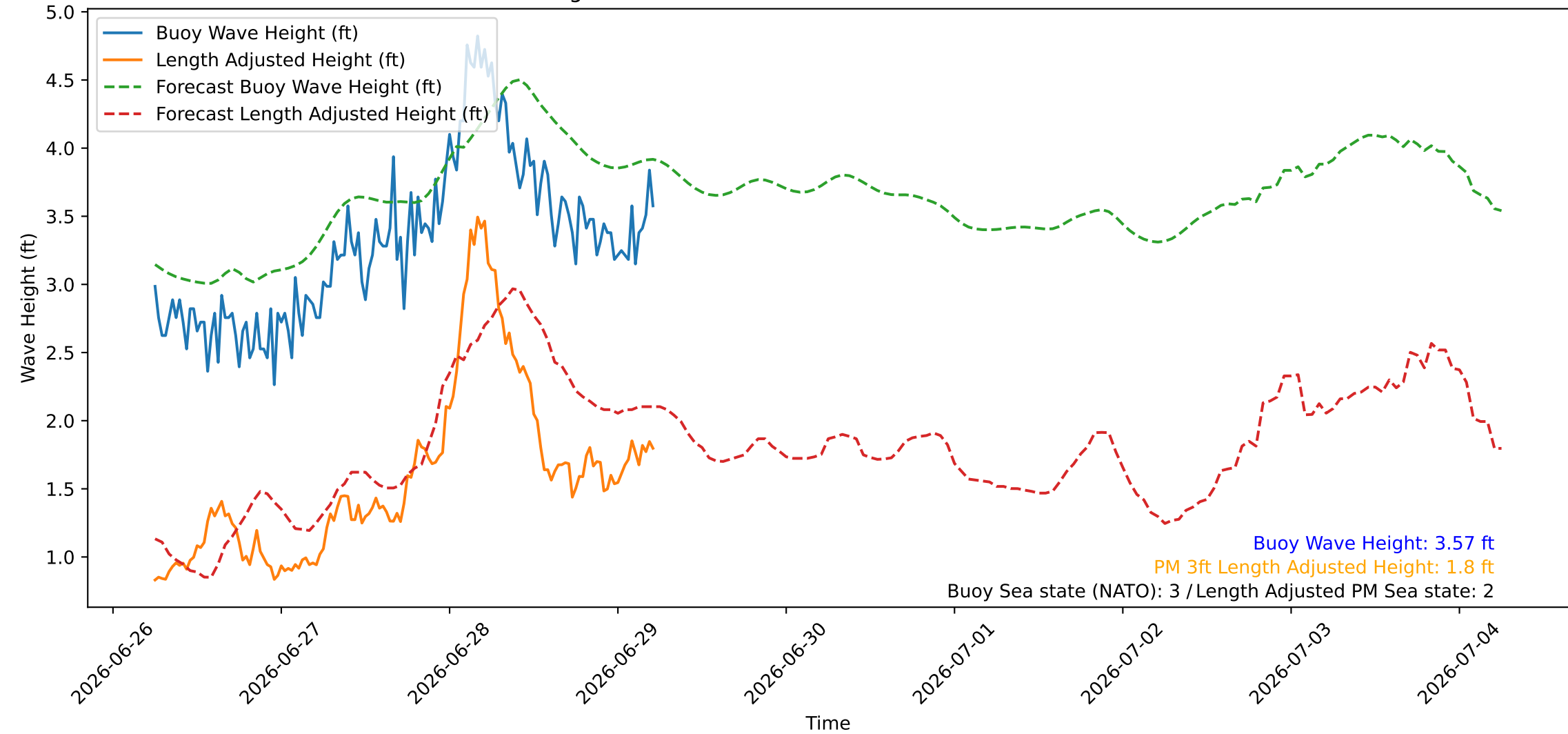
Wave Heights over Time for Green Beach at 2026-06-29 05:51:09
