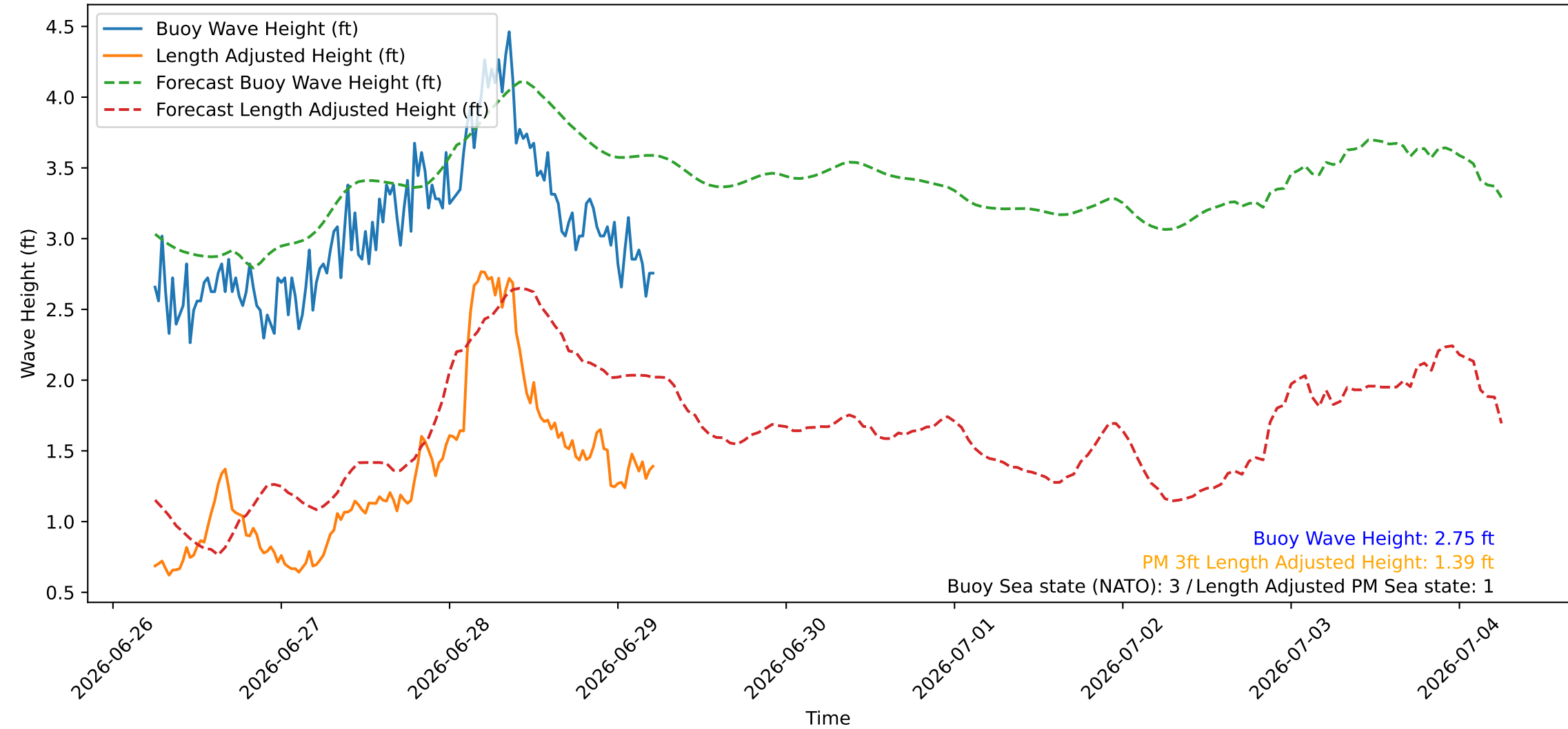
Wave Heights over Time for Red Beach at 2026-06-29 05:50:47
