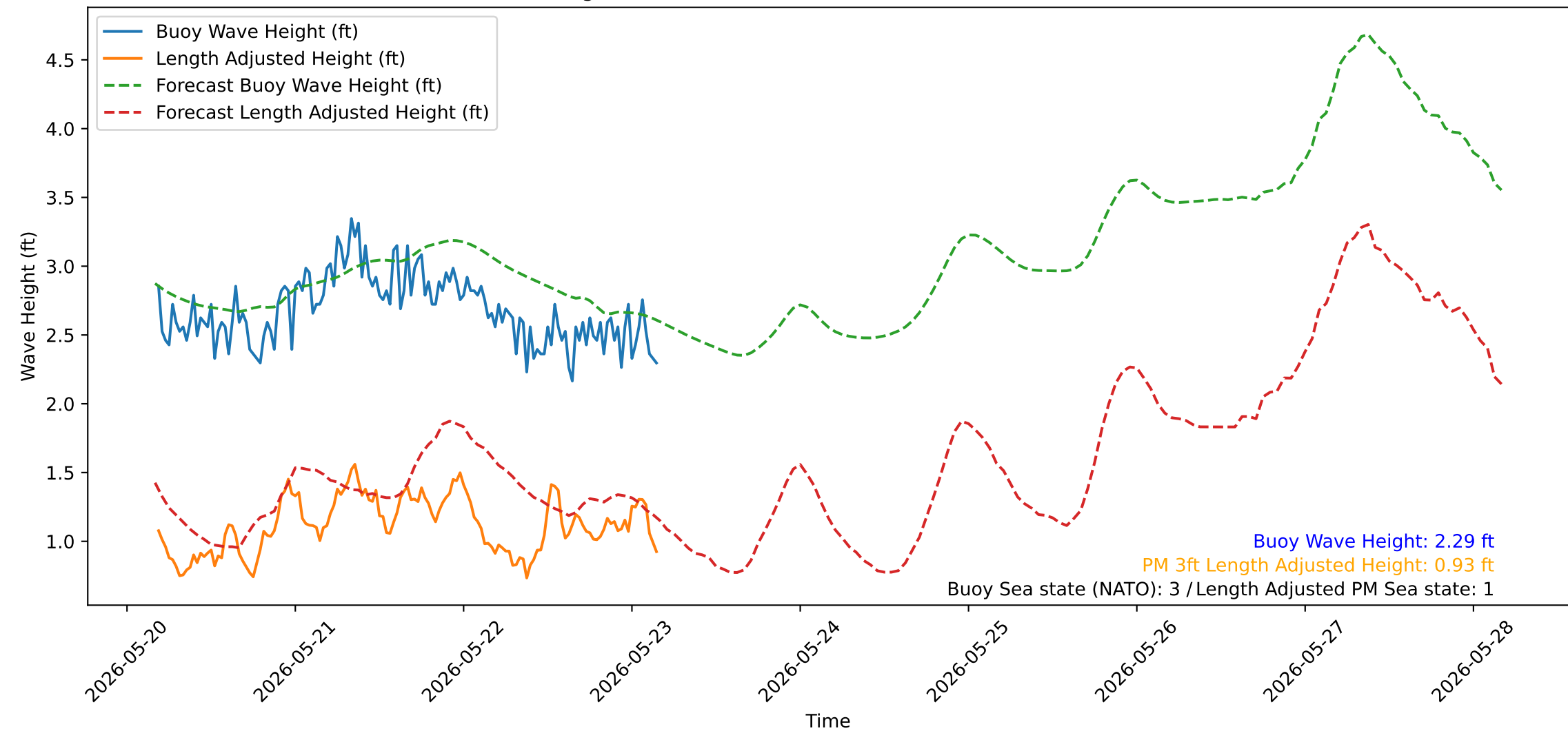
Wave Heights over Time for Red Beach at 2026-05-23 04:20:52
