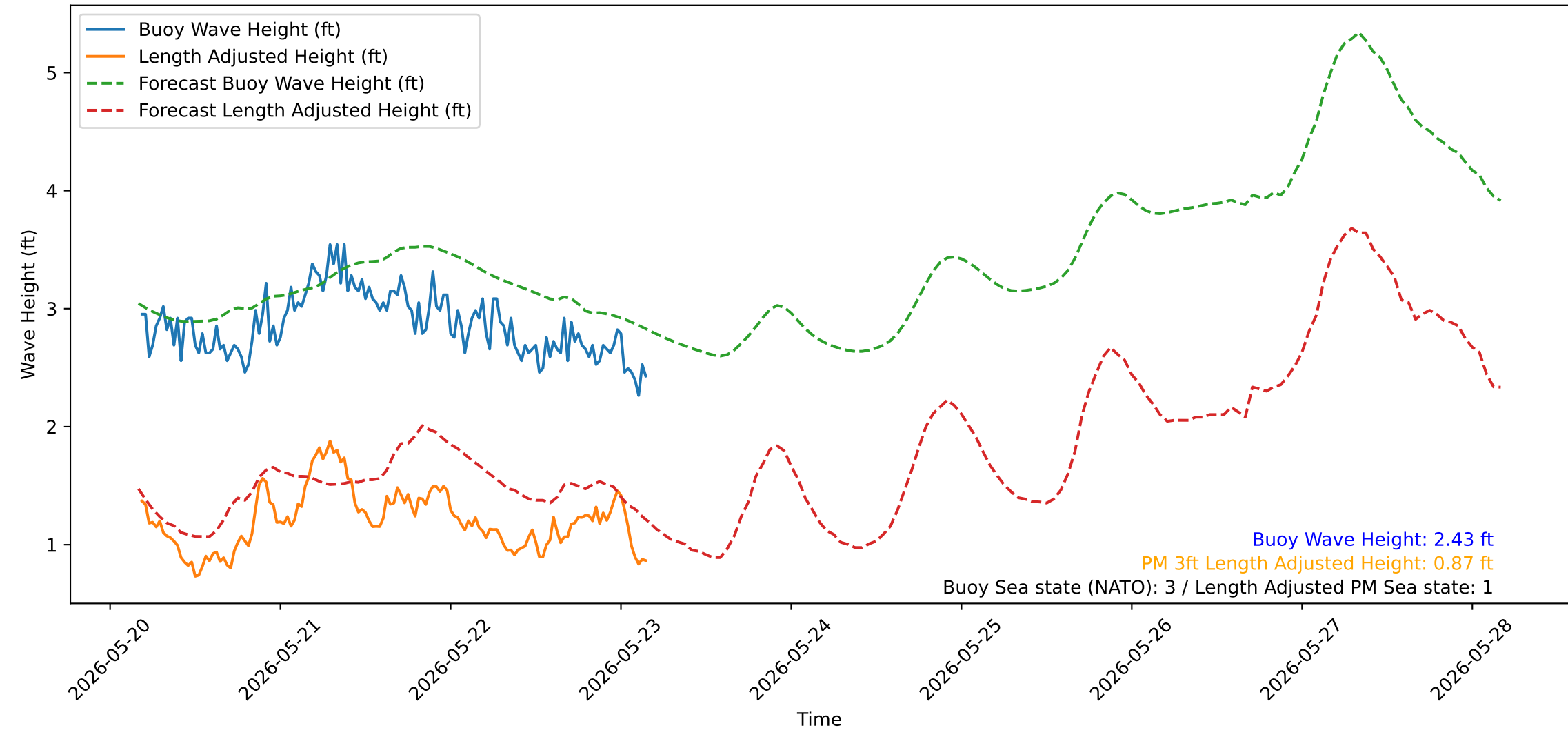
Wave Heights over Time for Green Beach at 2026-05-23 04:21:15
