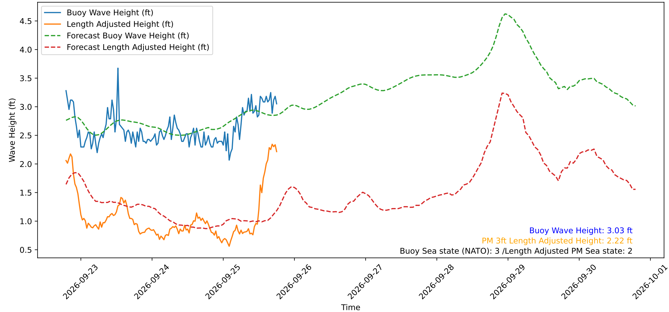
Wave Heights over Time for Red Beach at 2026-09-25 18:40:49
