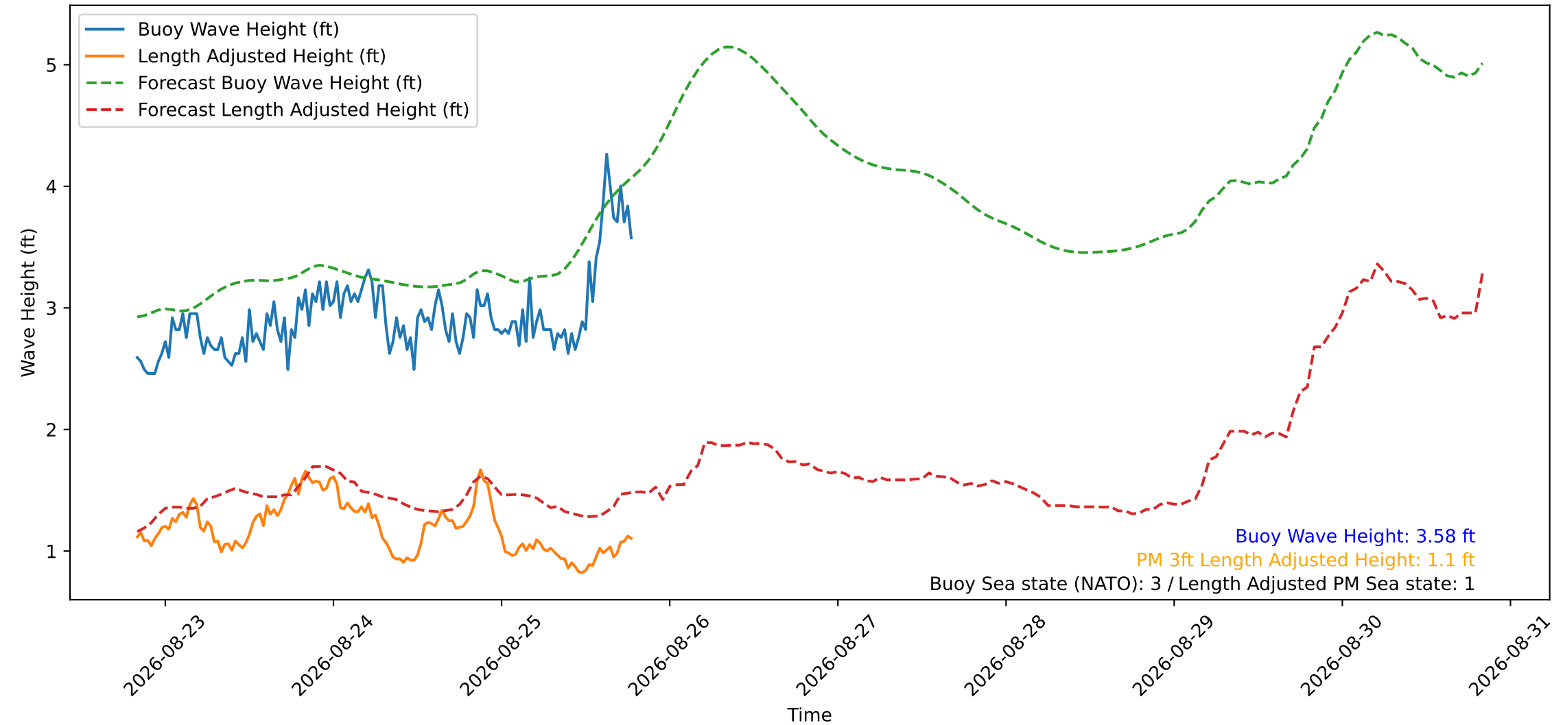
Wave Heights over Time for Green Beach at 2026-08-25 19:31:12
