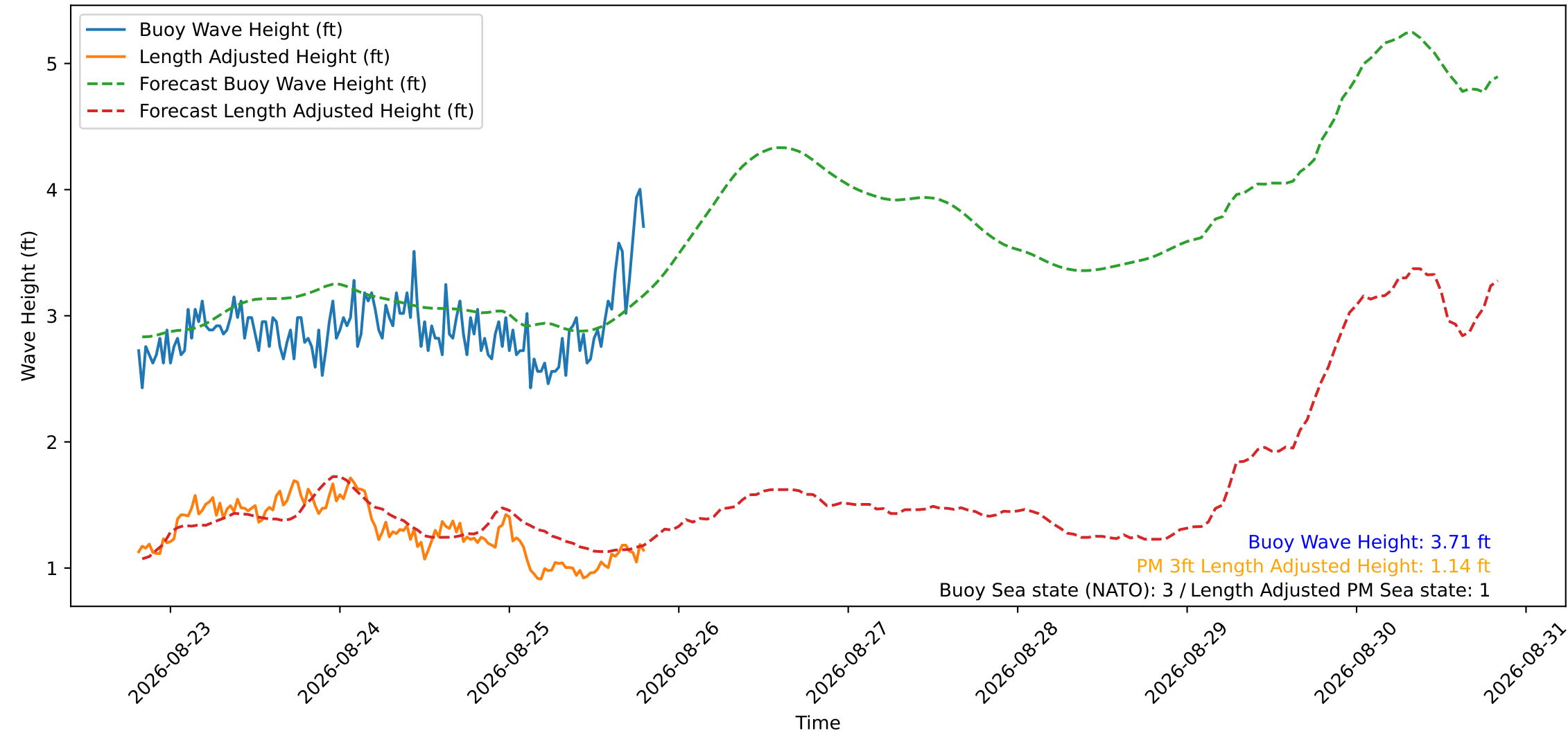
Wave Heights over Time for Oceanside Harbor at 2026-08-25 19:30:30
