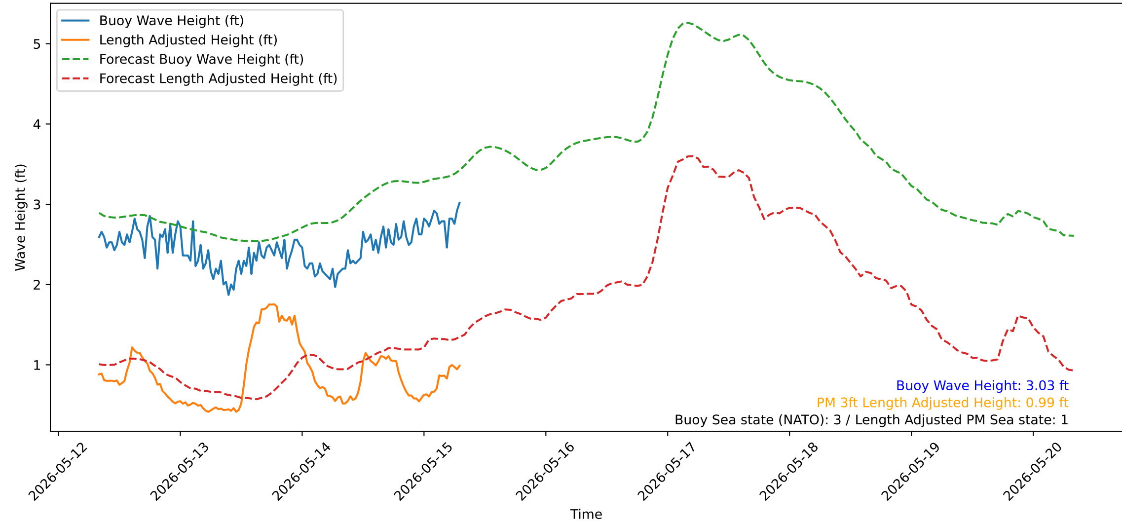
Wave Heights over Time for Red Beach at 2026-05-15 07:40:51
