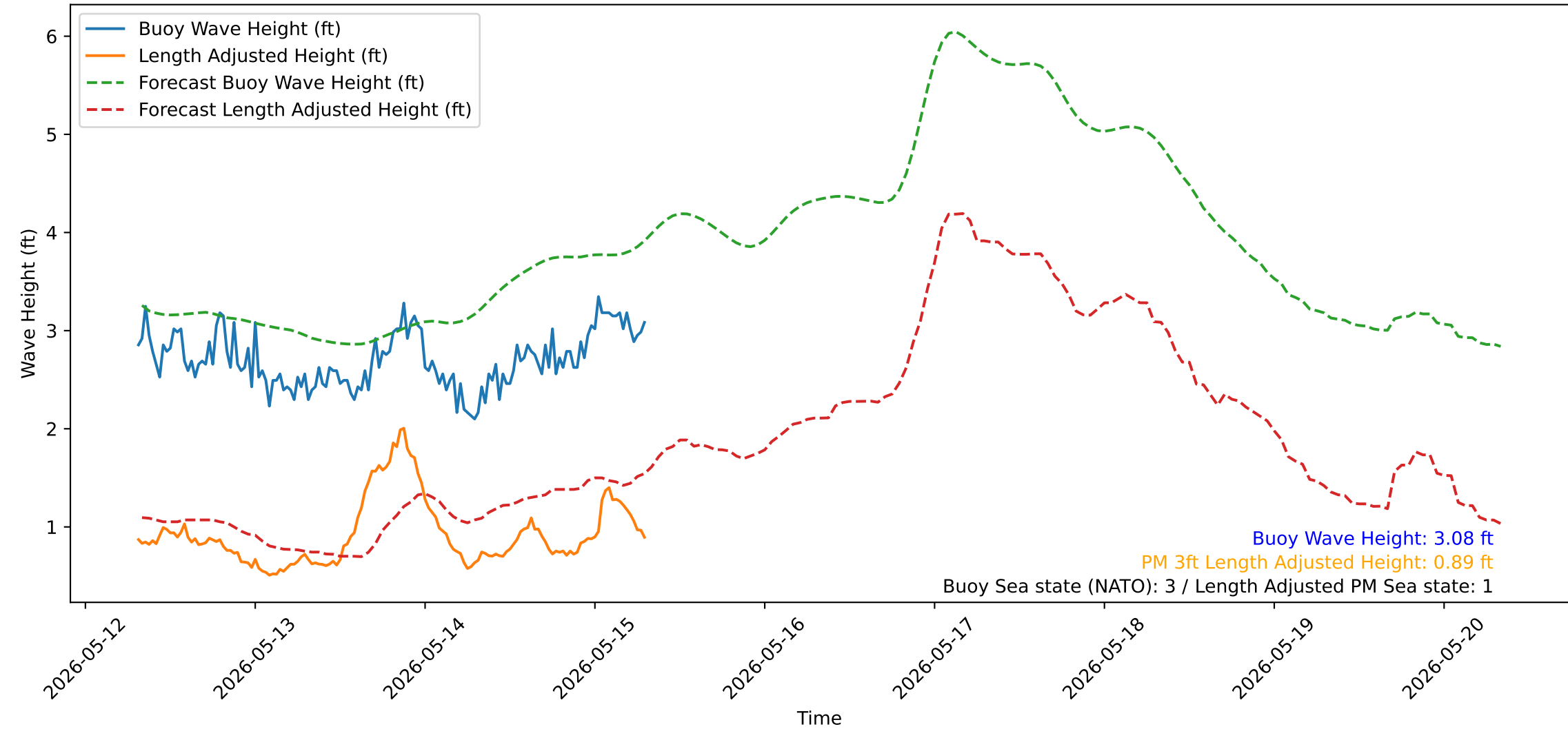
Wave Heights over Time for Green Beach at 2026-05-15 07:41:14
