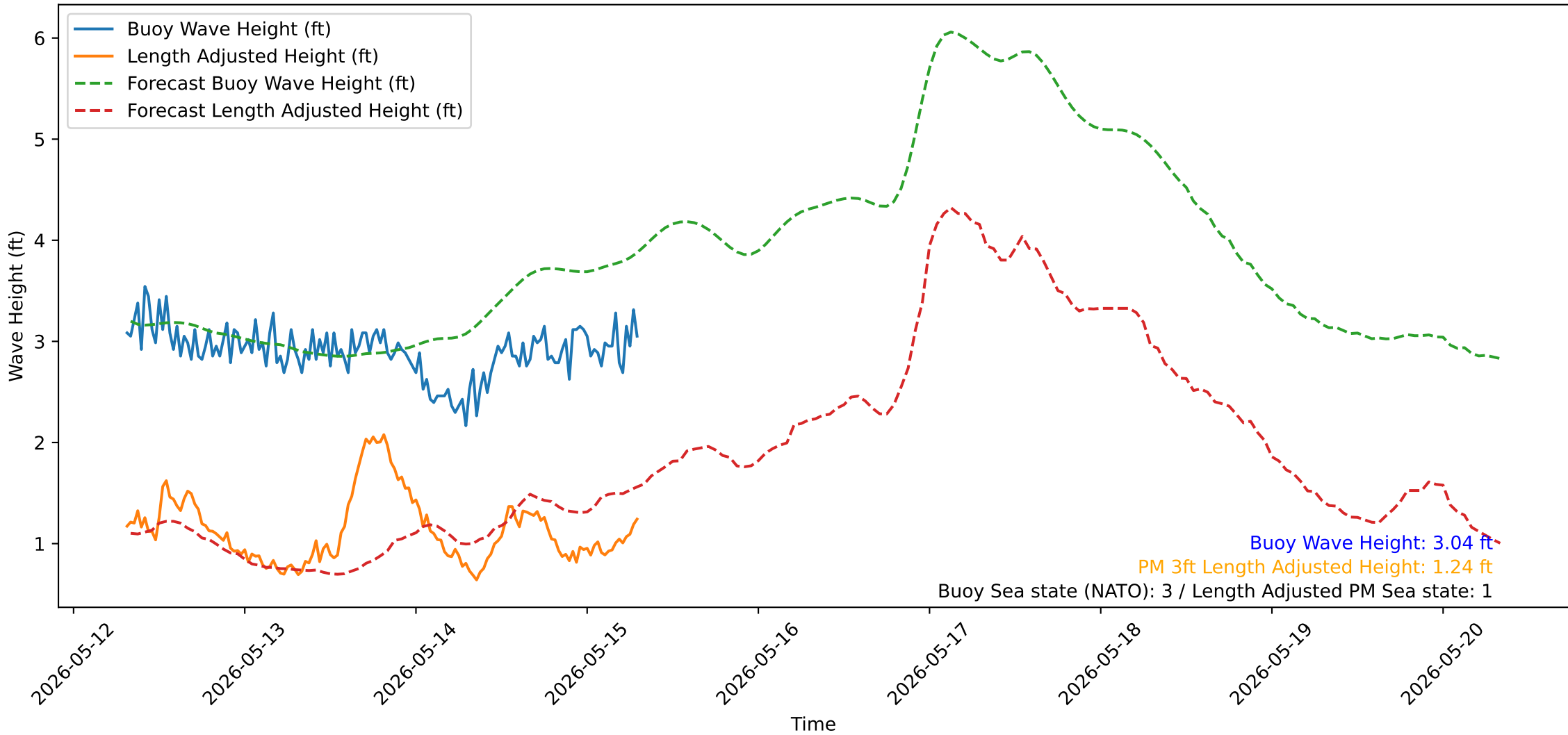
Wave Heights over Time for Oceanside Harbor at 2026-05-15 07:40:32
