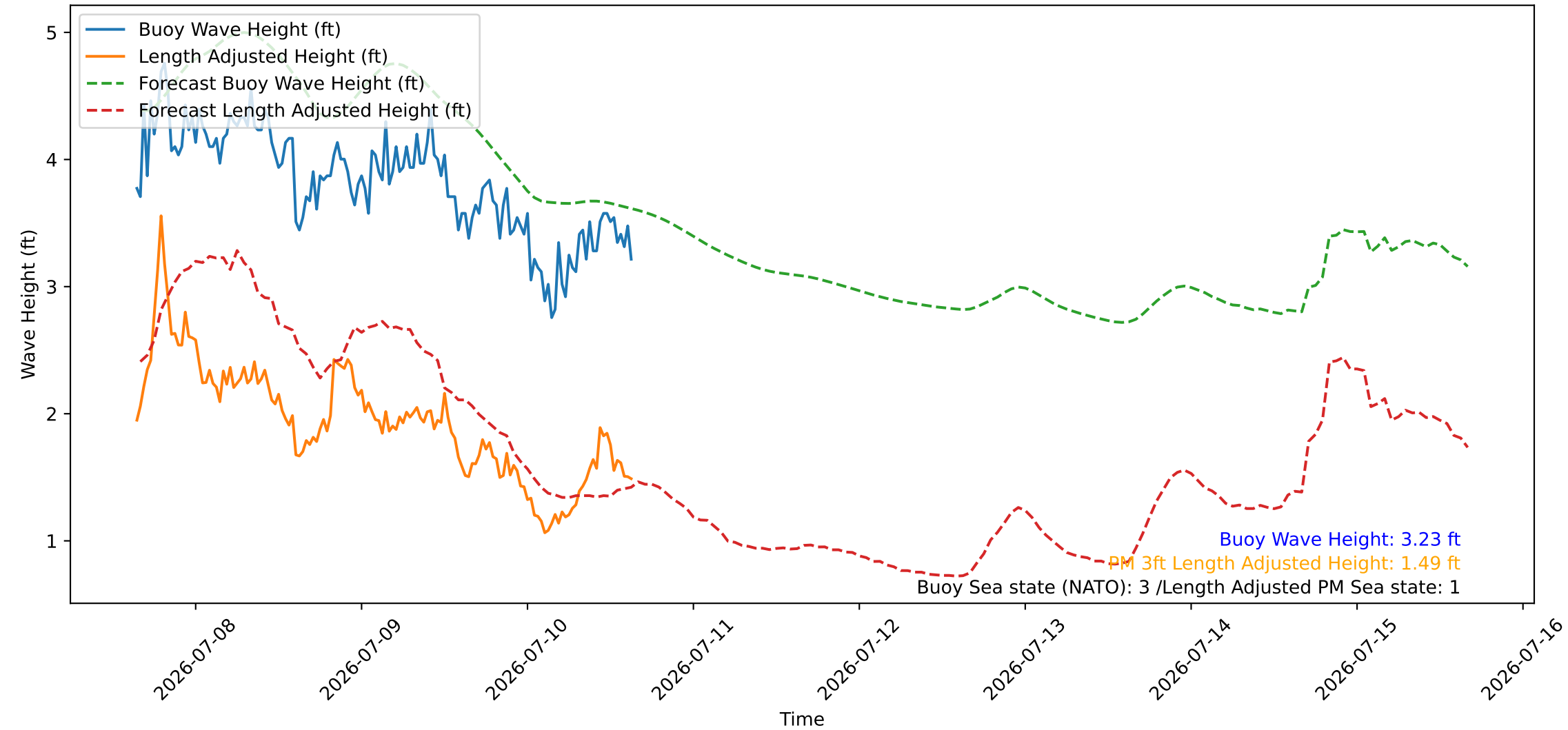
Wave Heights over Time for Green Beach at 2026-07-10 15:41:07
