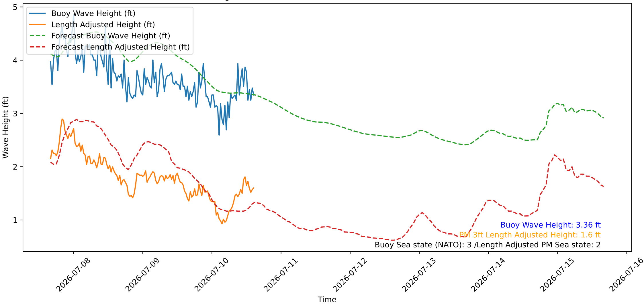
Wave Heights over Time for Red Beach at 2026-07-10 15:40:45
