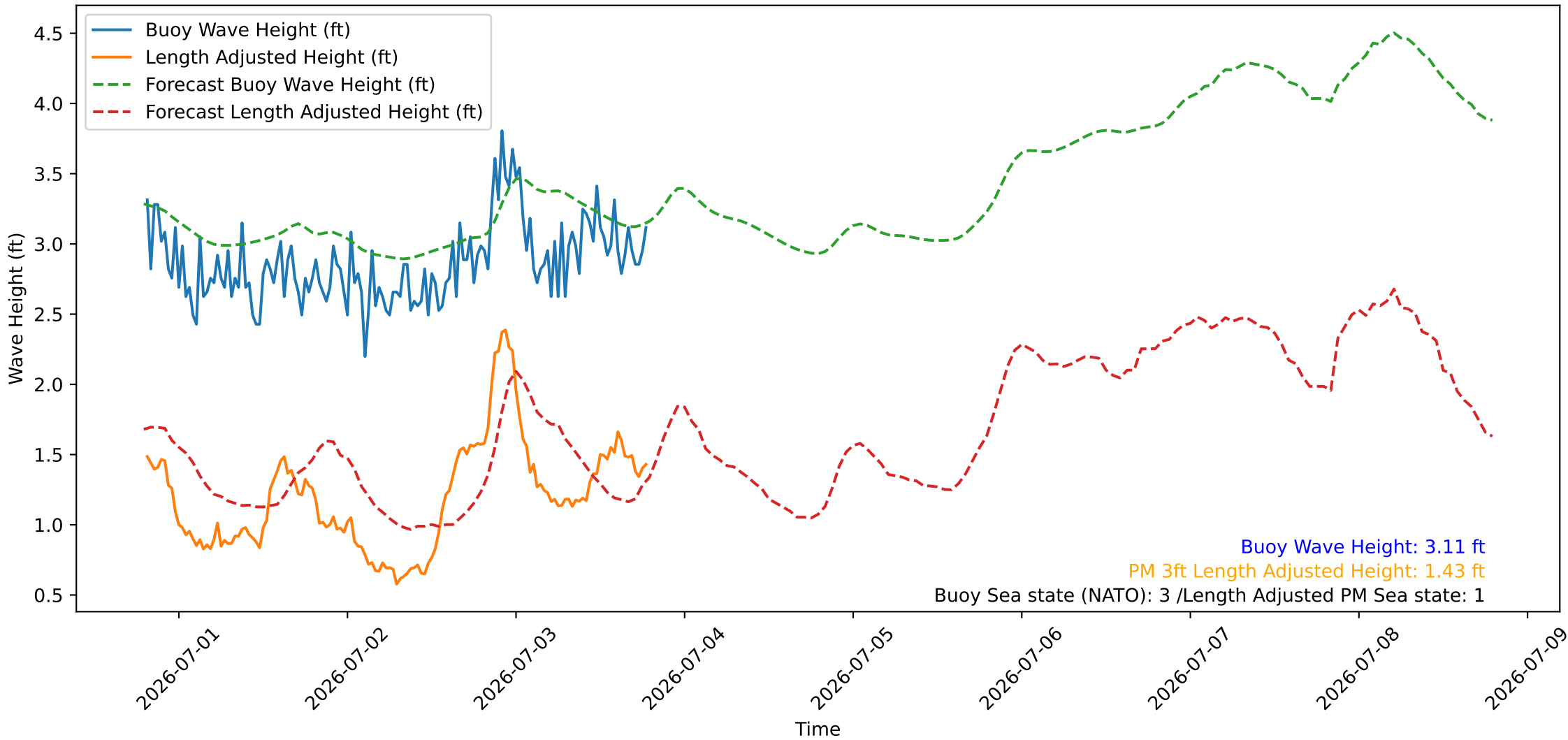
Wave Heights over Time for Red Beach at 2026-07-03 19:20:47
