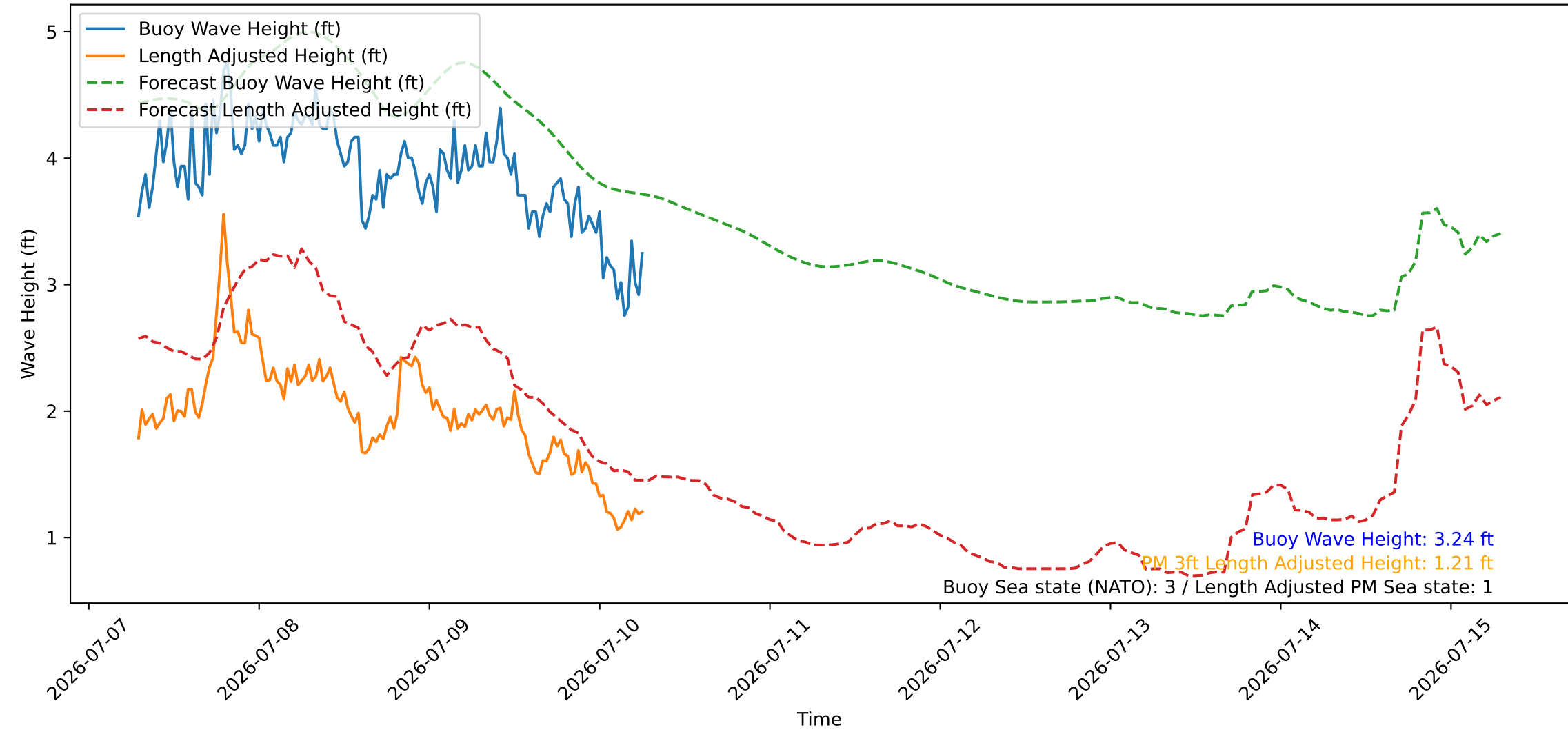
Wave Heights over Time for Green Beach at 2026-07-10 07:01:08
