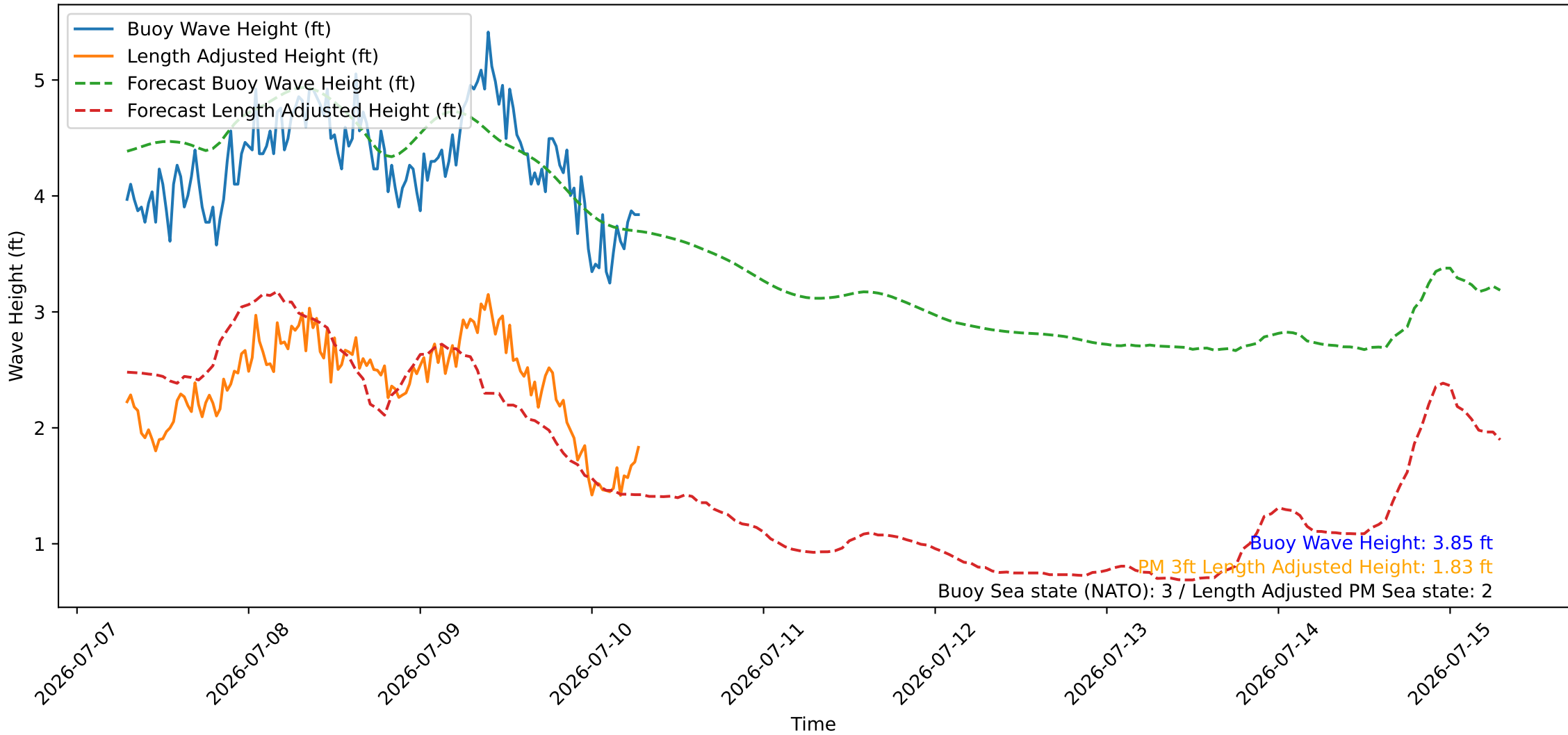
Wave Heights over Time for Oceanside Harbor at 2026-07-10 07:00:27
