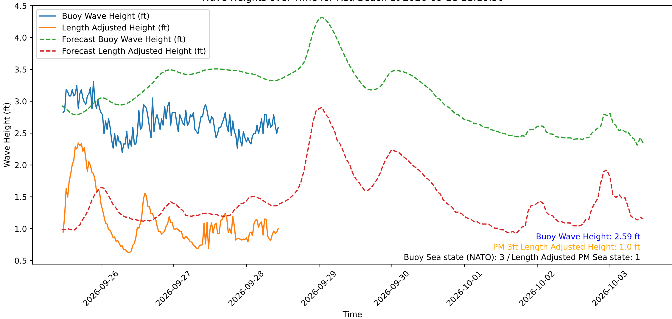
Wave Heights over Time for Red Beach at 2026-09-28 11:10:50
