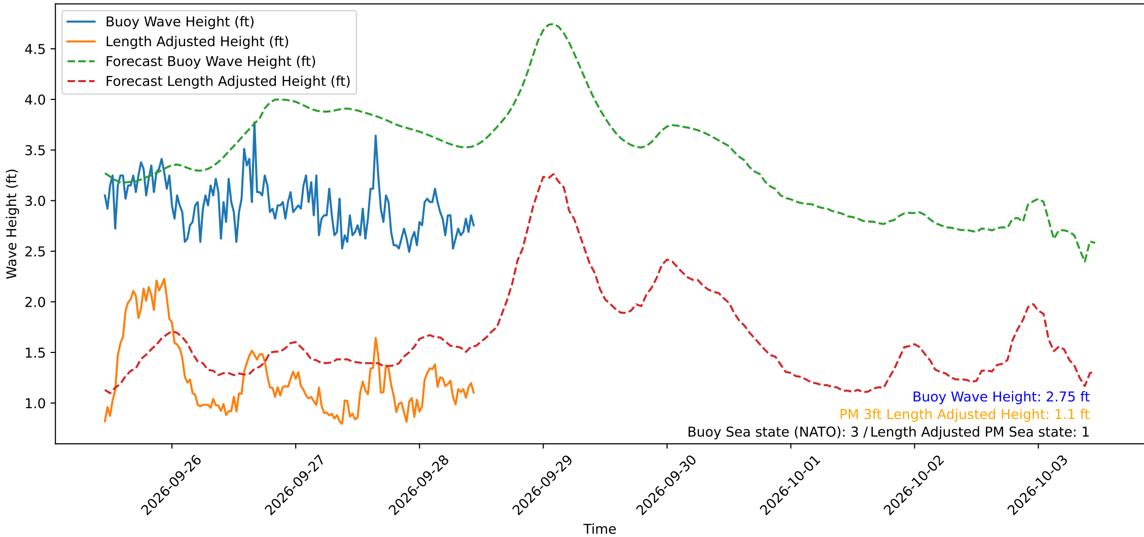
Wave Heights over Time for Oceanside Harbor at 2026-09-28 11:10:30
