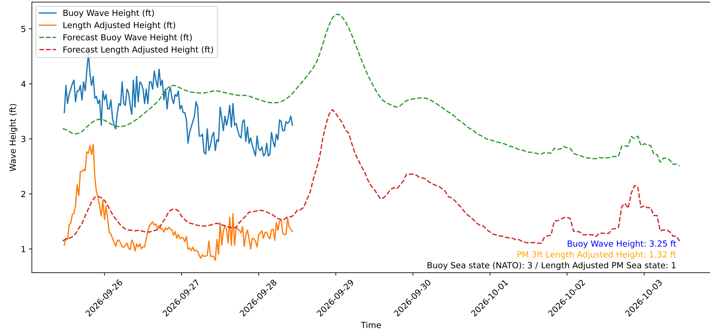
Wave Heights over Time for Green Beach at 2026-09-28 11:11:13
