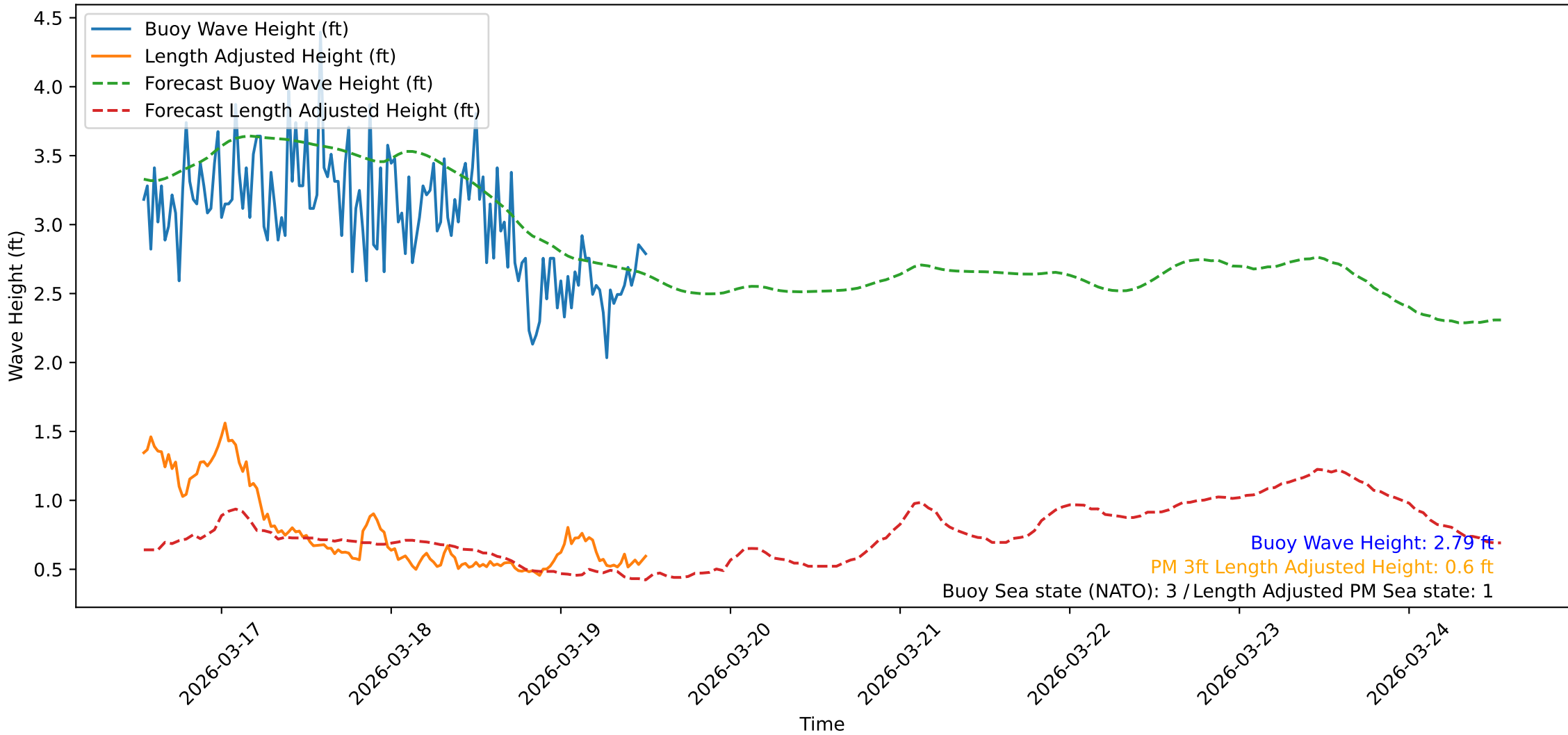
Wave Heights over Time for Oceanside Harbor at 2026-03-19 12:50:30
