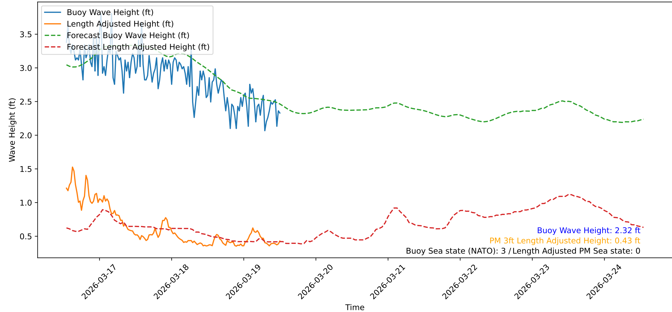
Wave Heights over Time for Red Beach at 2026-03-19 12:50:47
