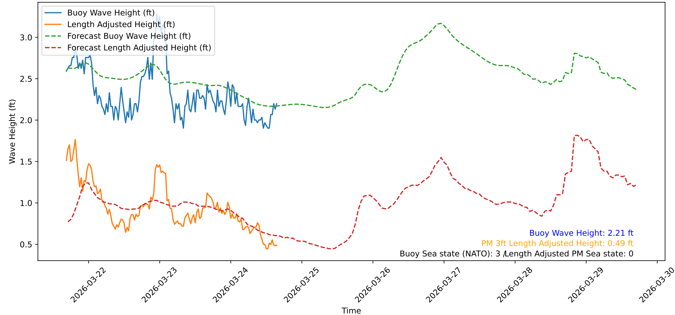
Wave Heights over Time for Green Beach at 2026-03-24 16:31:11
