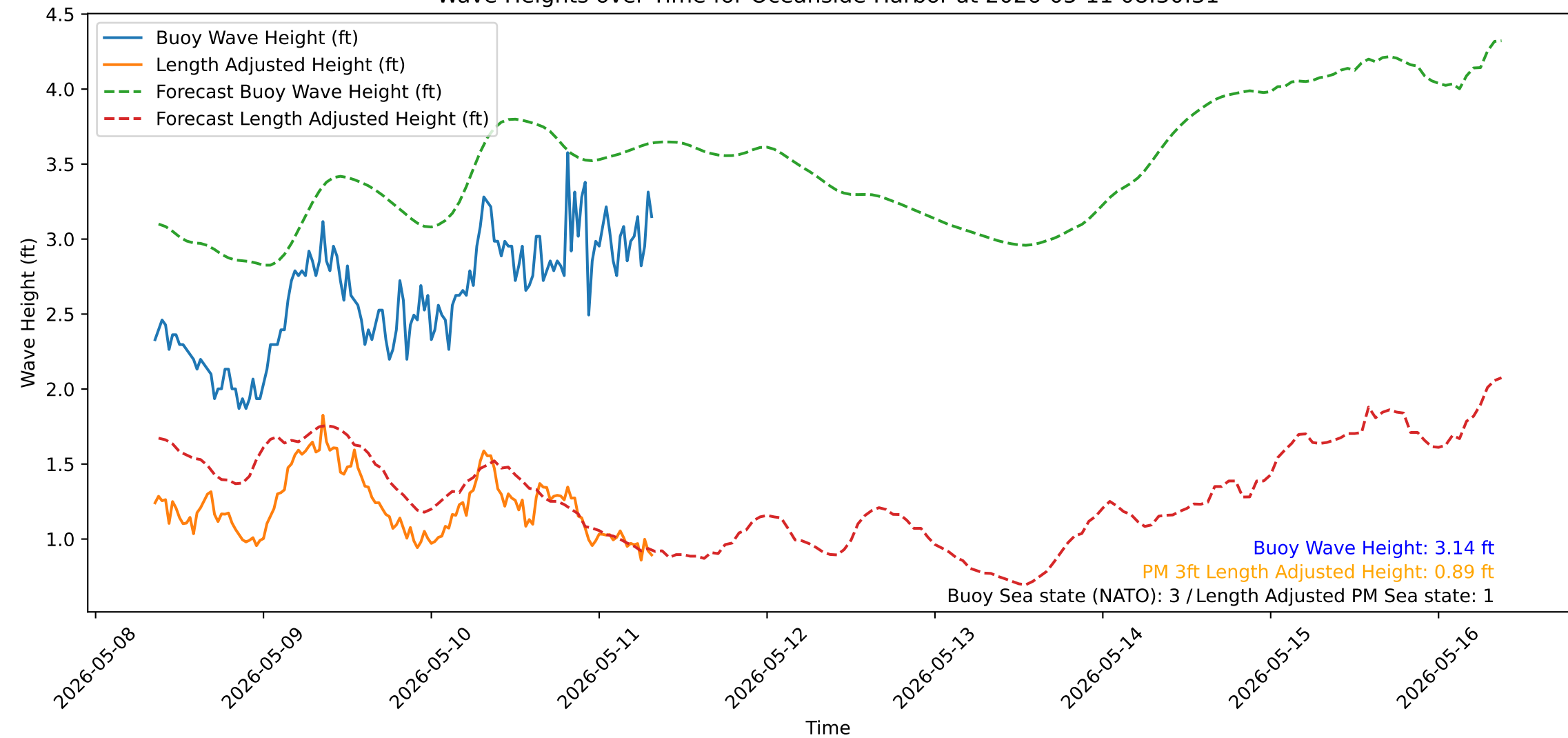
Wave Heights over Time for Oceanside Harbor at 2026-05-11 08:30:31
