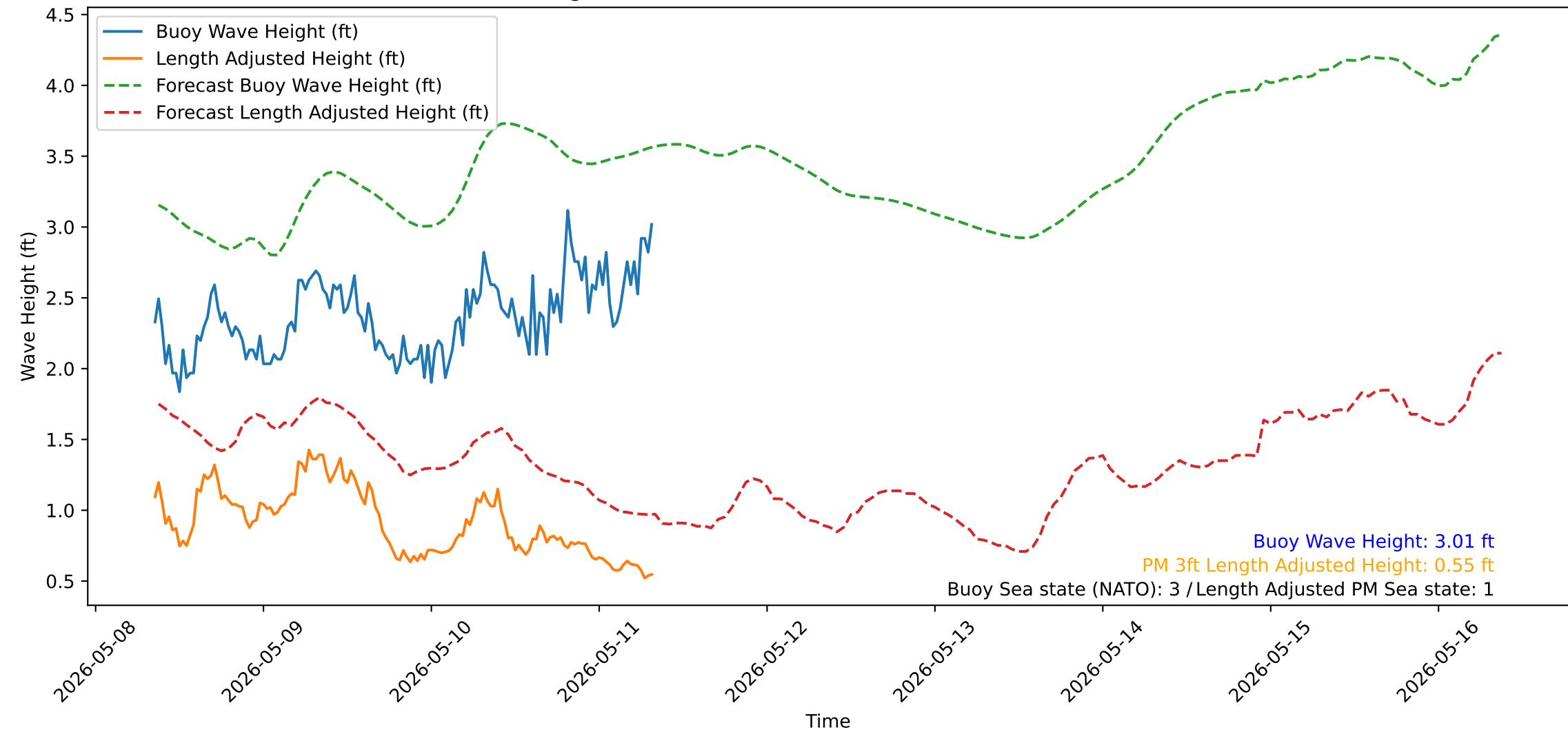
Wave Heights over Time for Green Beach at 2026-05-11 08:31:13
