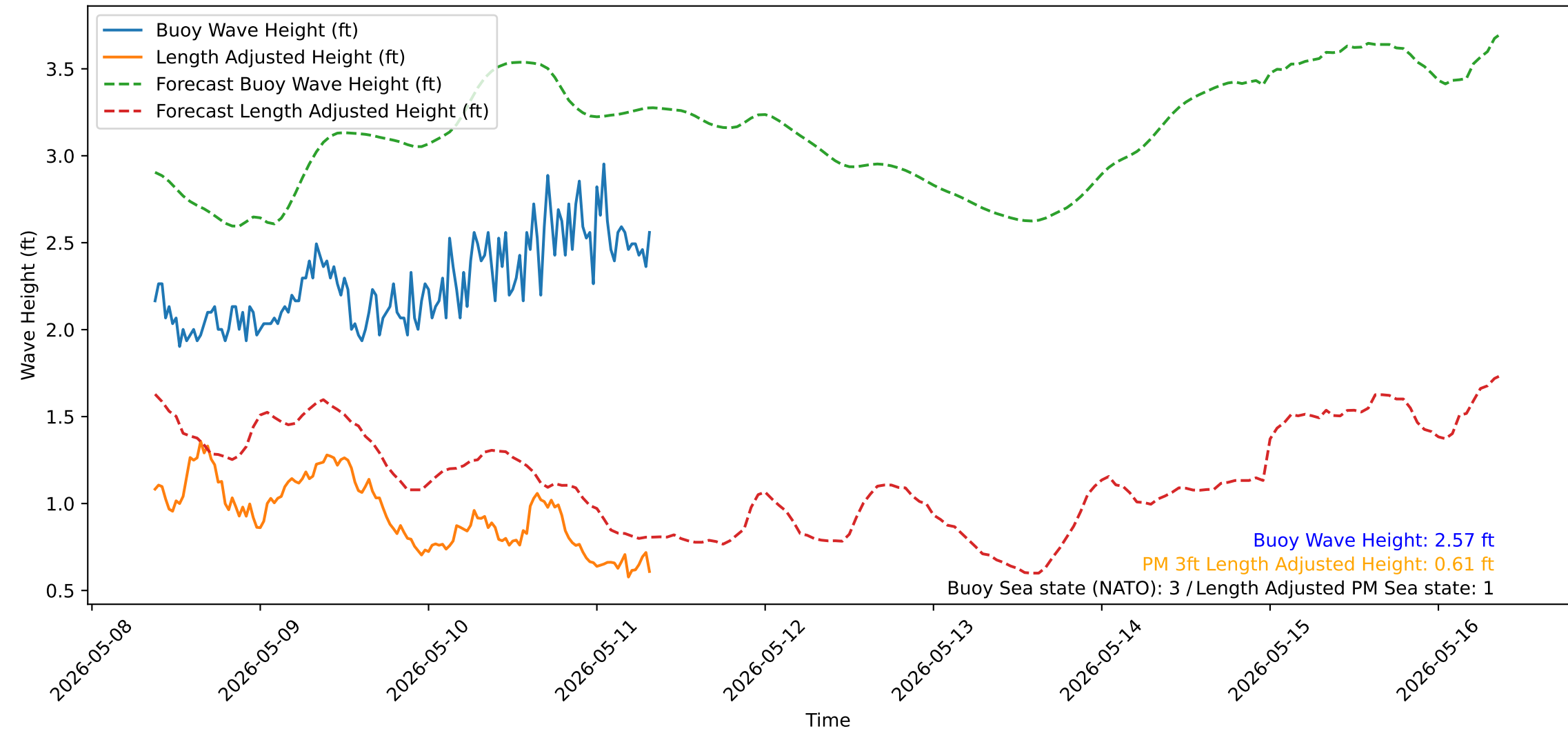
Wave Heights over Time for Red Beach at 2026-05-11 08:30:51
