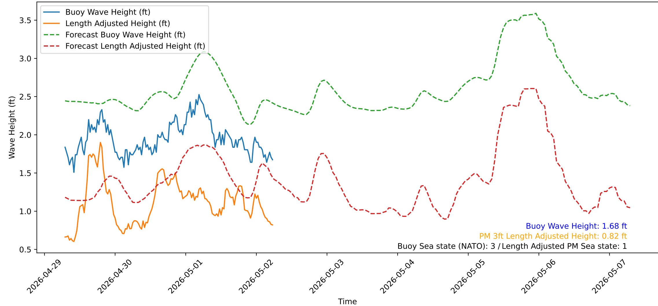
Wave Heights over Time for Red Beach at 2026-05-02 06:30:50
