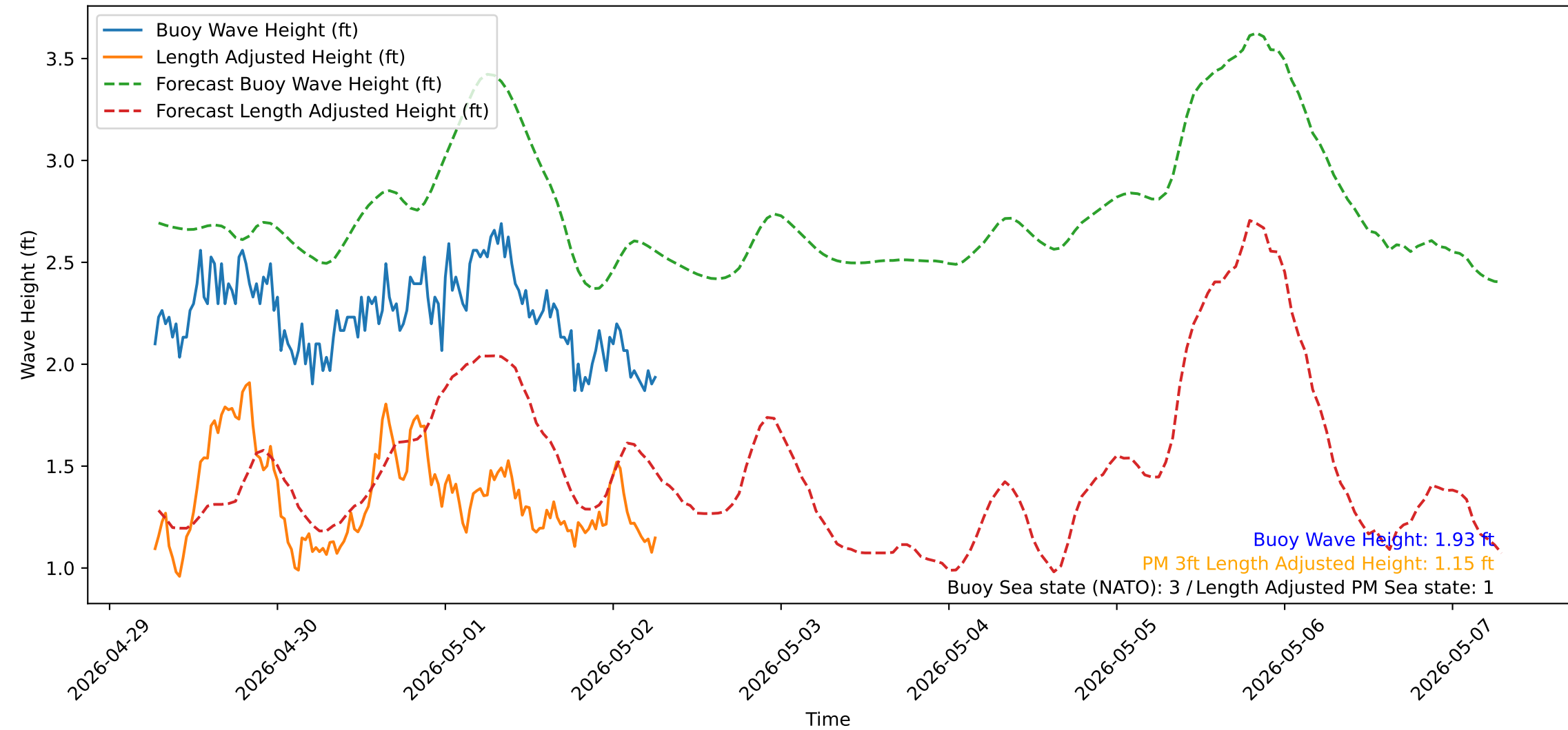
Wave Heights over Time for Oceanside Harbor at 2026-05-02 06:30:31
