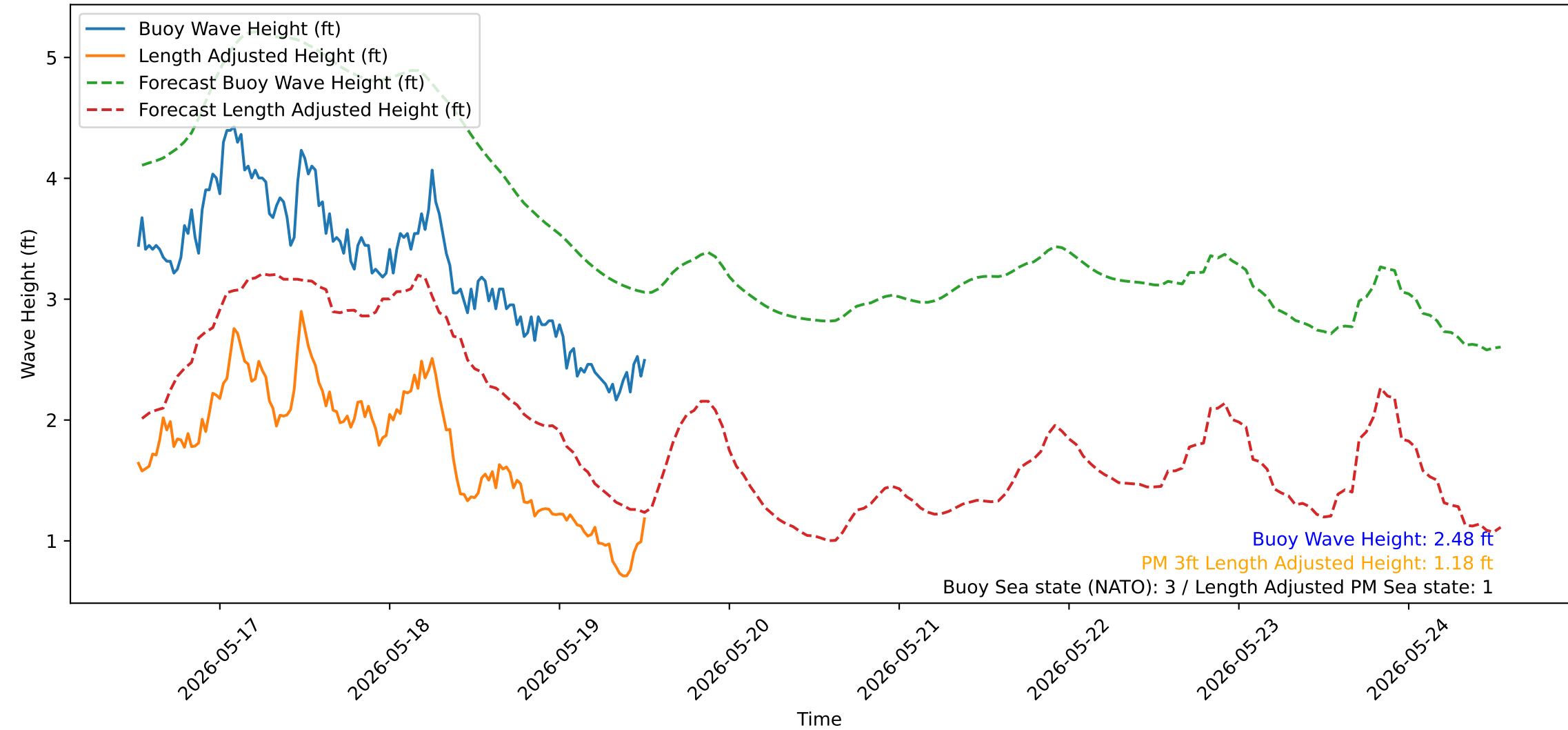
Wave Heights over Time for Green Beach at 2026-05-19 12:41:13
