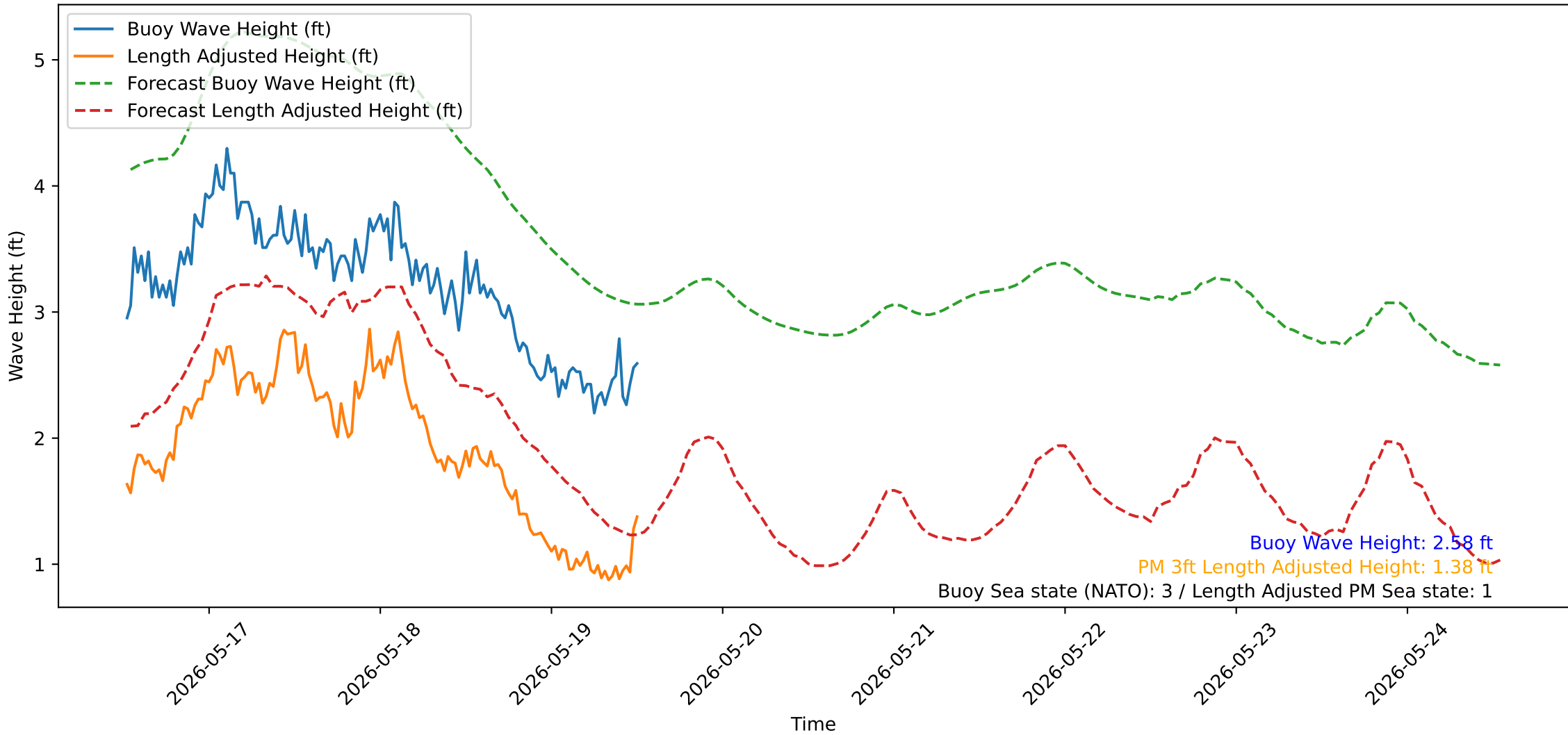
Wave Heights over Time for Oceanside Harbor at 2026-05-19 12:40:31
