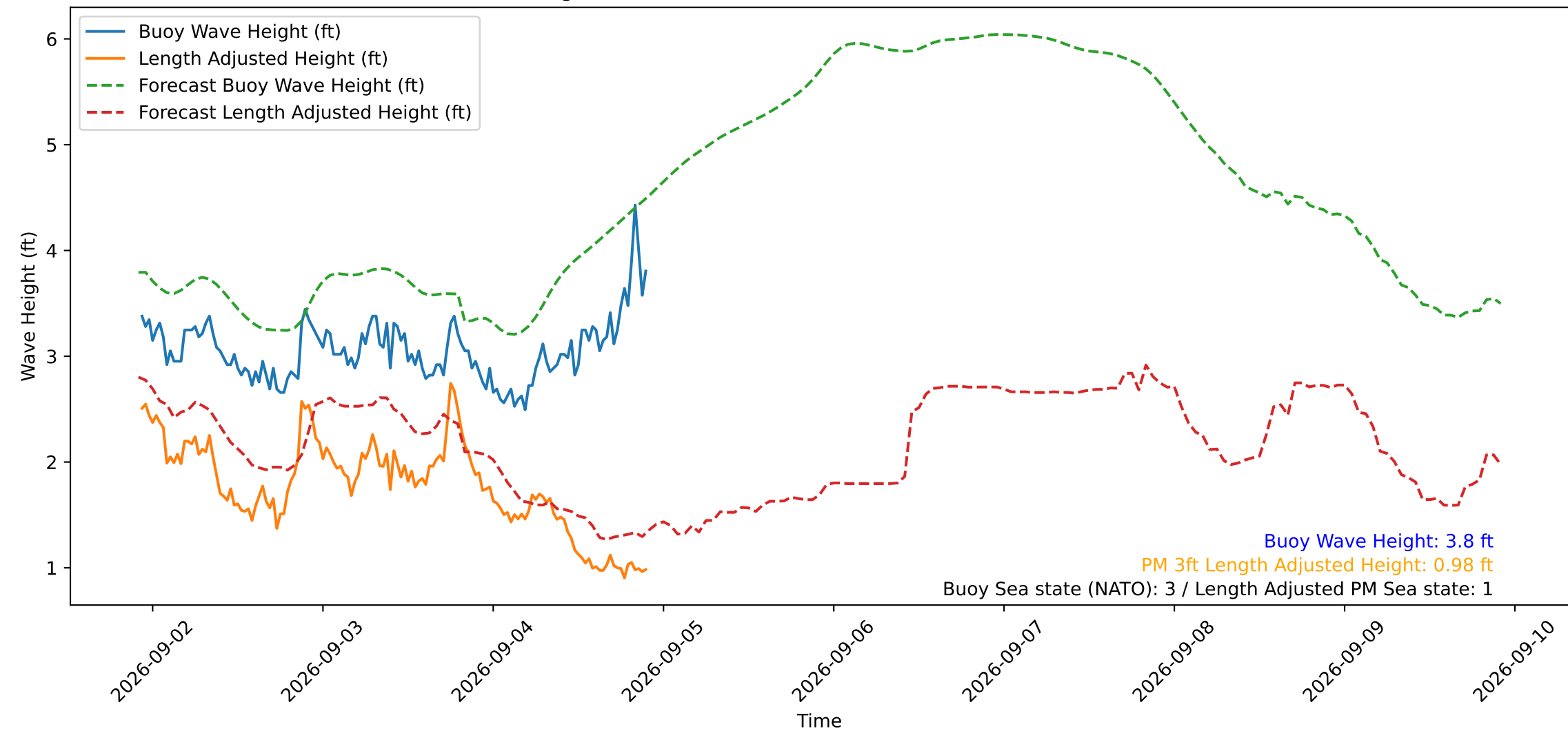
Wave Heights over Time for Green Beach at 2026-09-04 22:21:15
