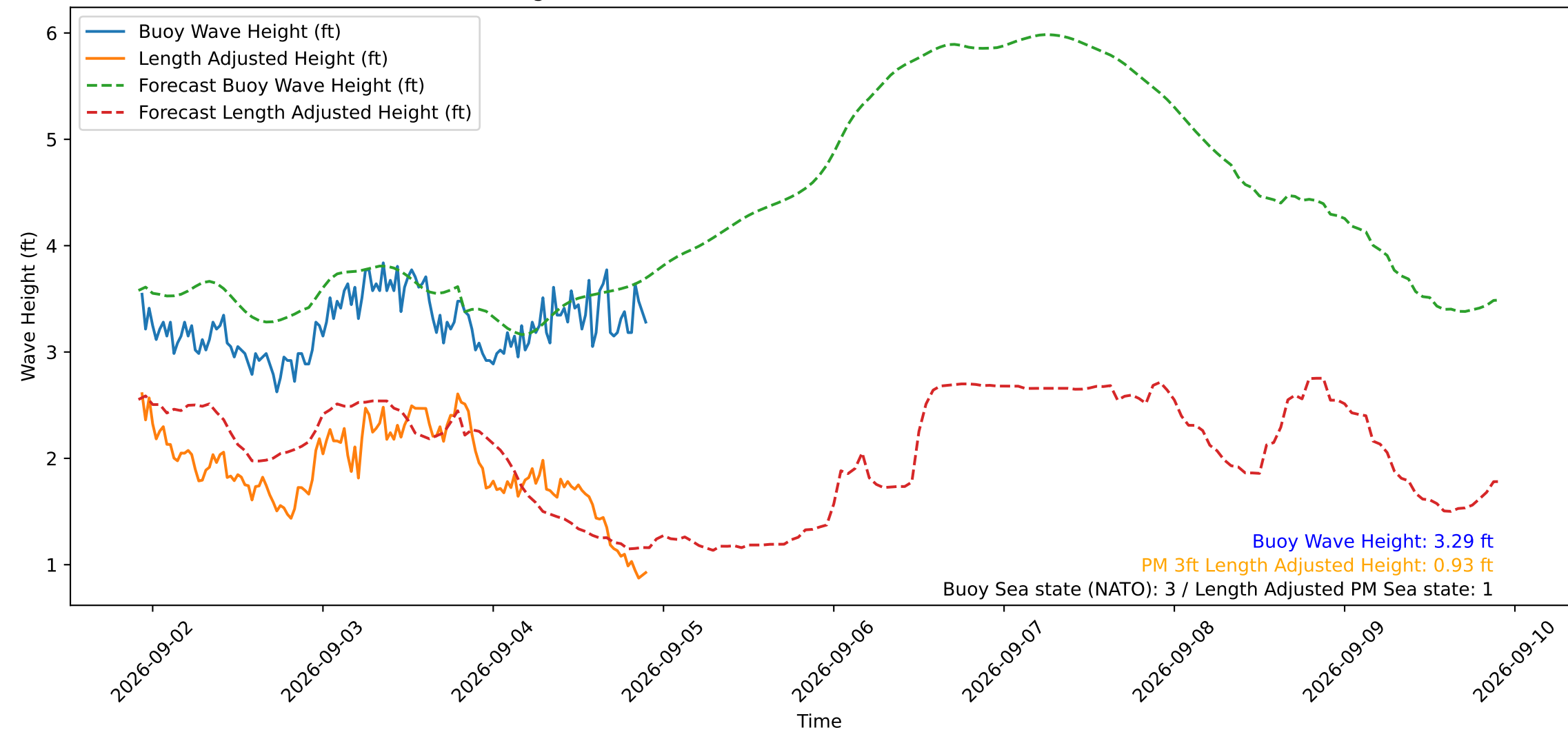
Wave Heights over Time for Oceanside Harbor at 2026-09-04 22:20:30
