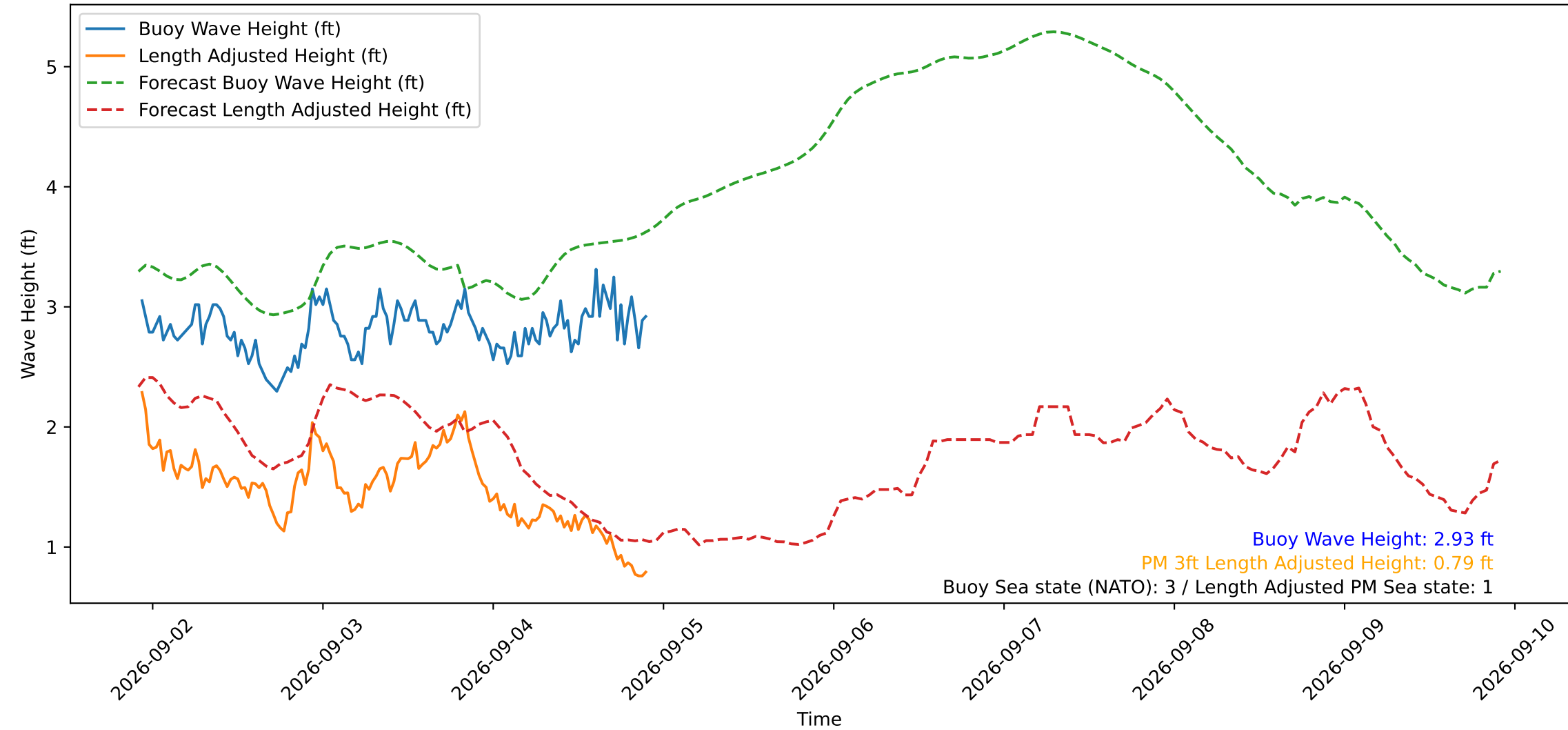
Wave Heights over Time for Red Beach at 2026-09-04 22:20:51
