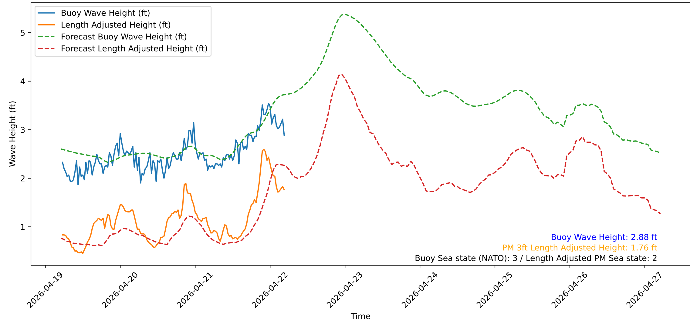
Wave Heights over Time for Green Beach at 2026-04-22 05:21:13
