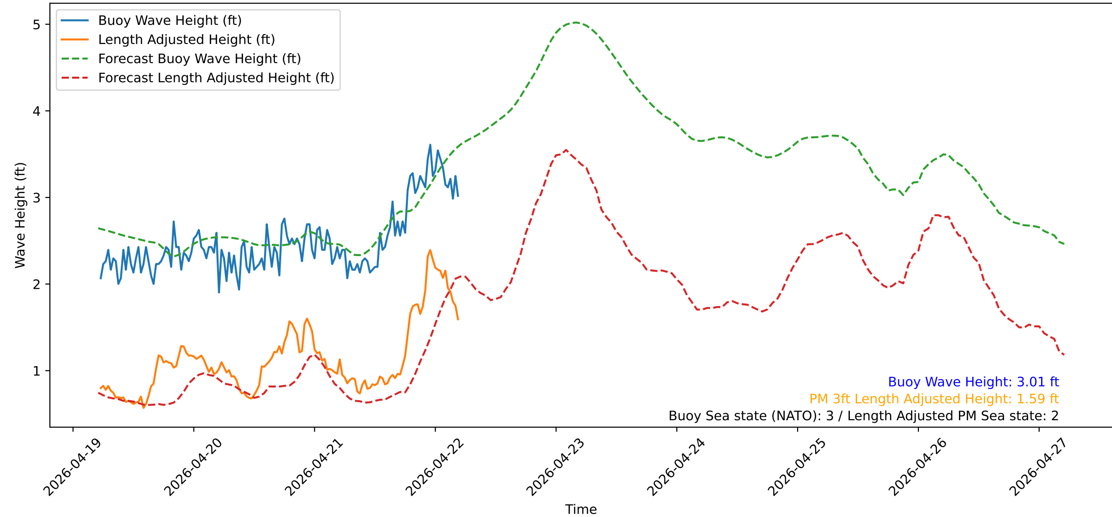
Wave Heights over Time for Oceanside Harbor at 2026-04-22 05:20:31
