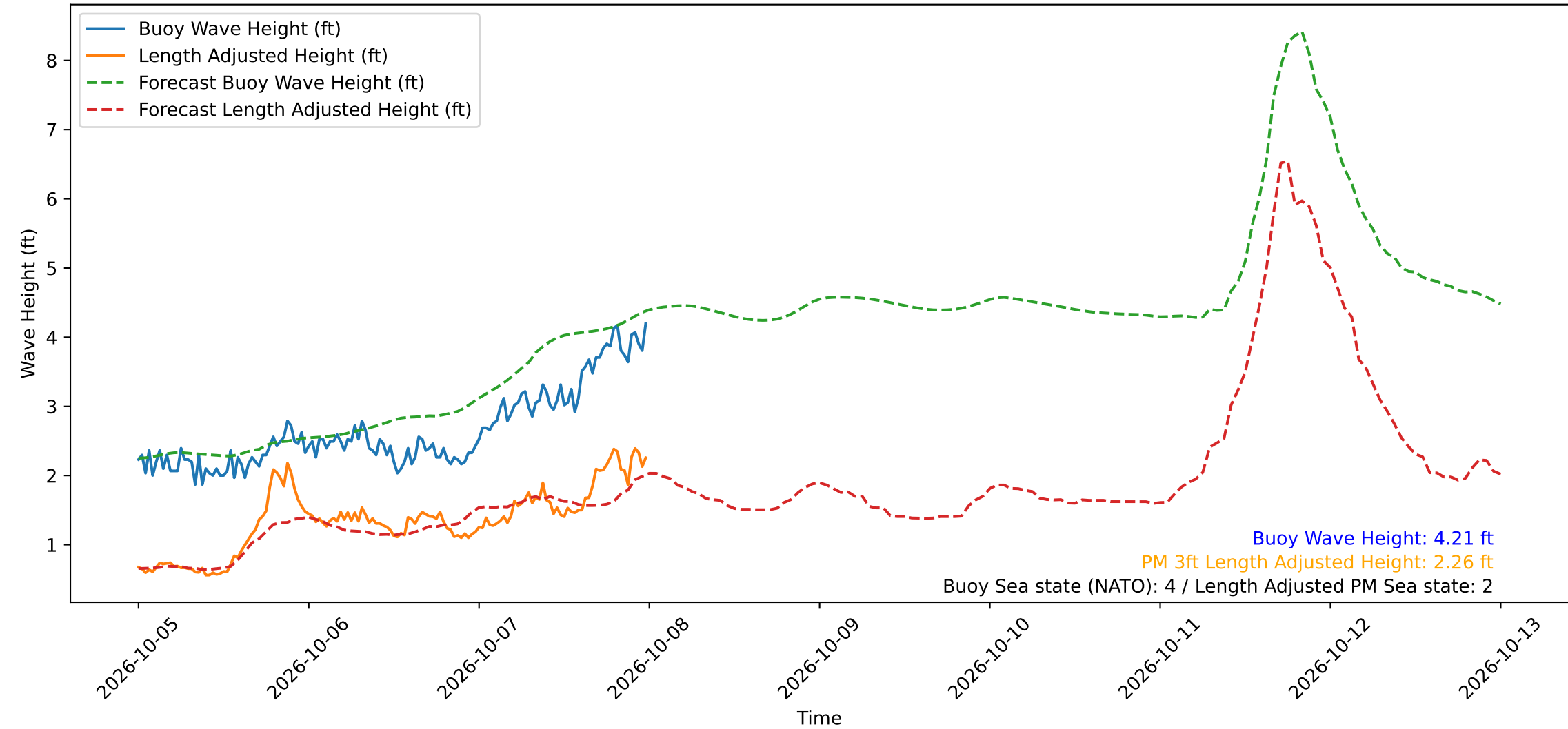
Wave Heights over Time for Oceanside Harbor at 2026-10-08 00:10:29
