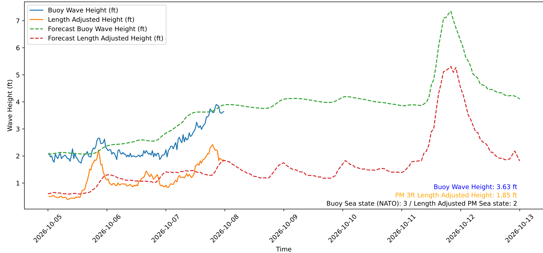
Wave Heights over Time for Red Beach at 2026-10-08 00:10:49
