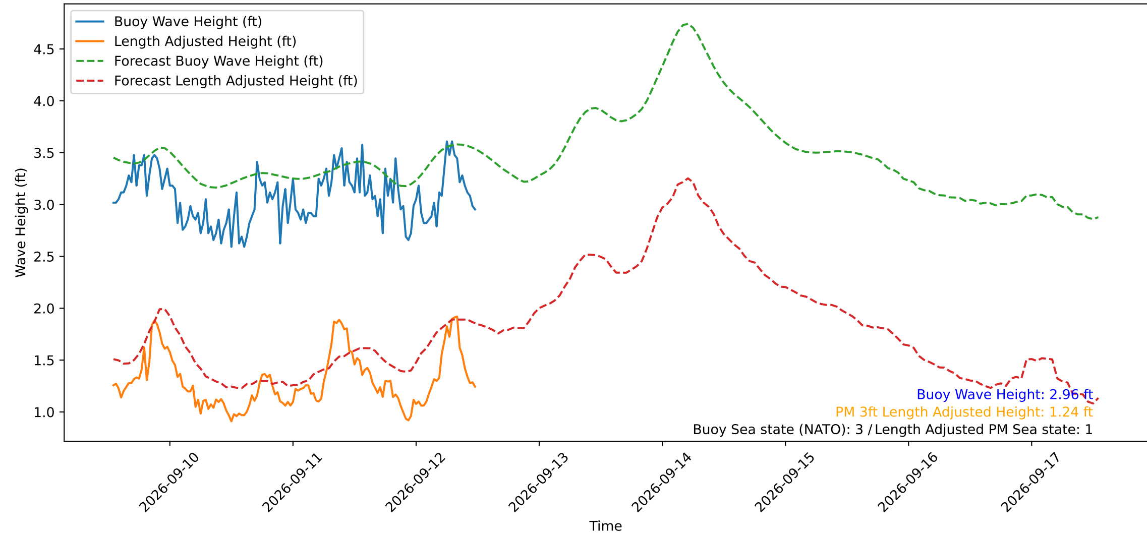
Wave Heights over Time for Green Beach at 2026-09-12 12:31:12
