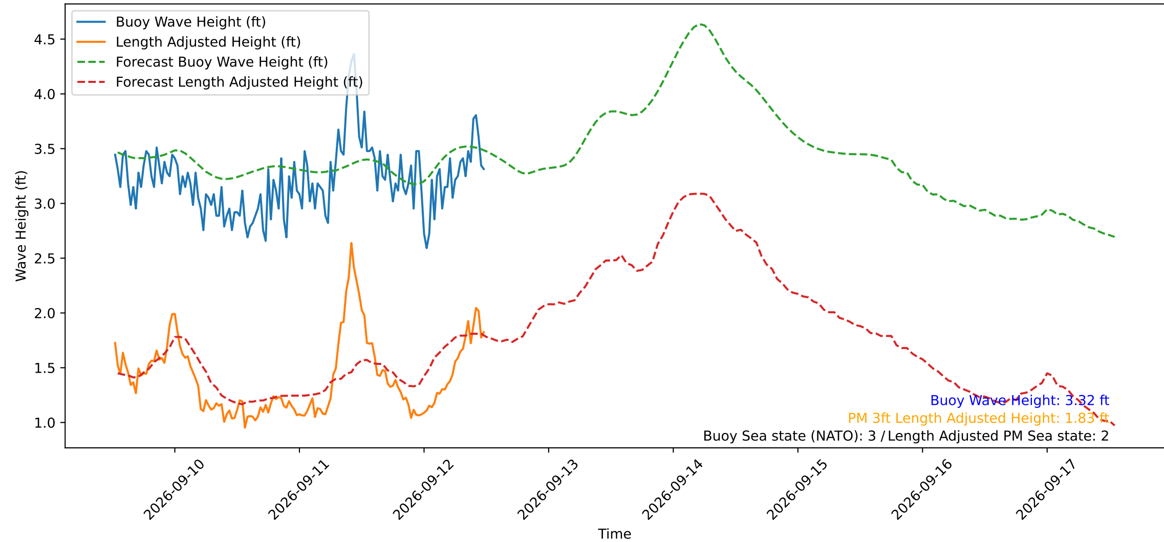
Wave Heights over Time for Oceanside Harbor at 2026-09-12 12:30:29
