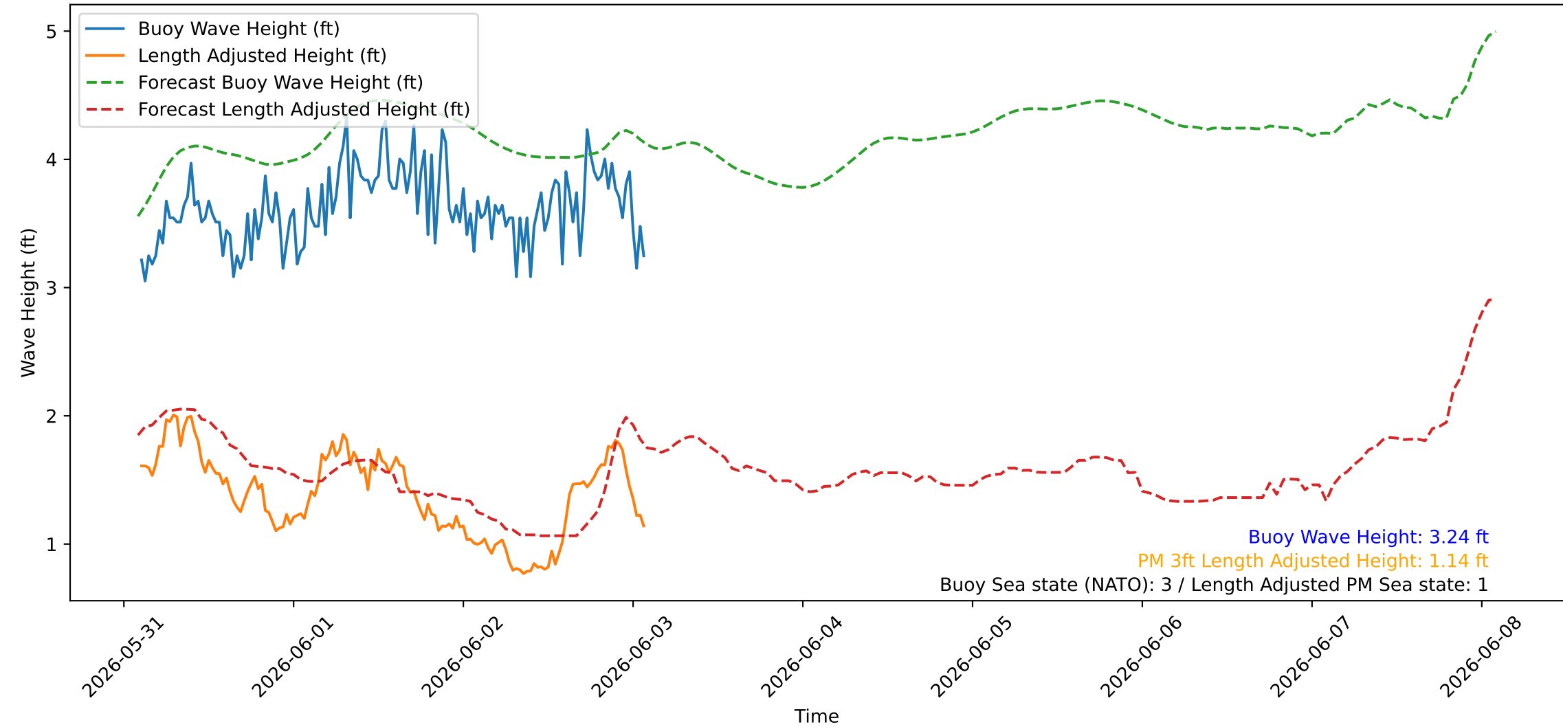
Wave Heights over Time for Green Beach at 2026-06-03 02:21:09
