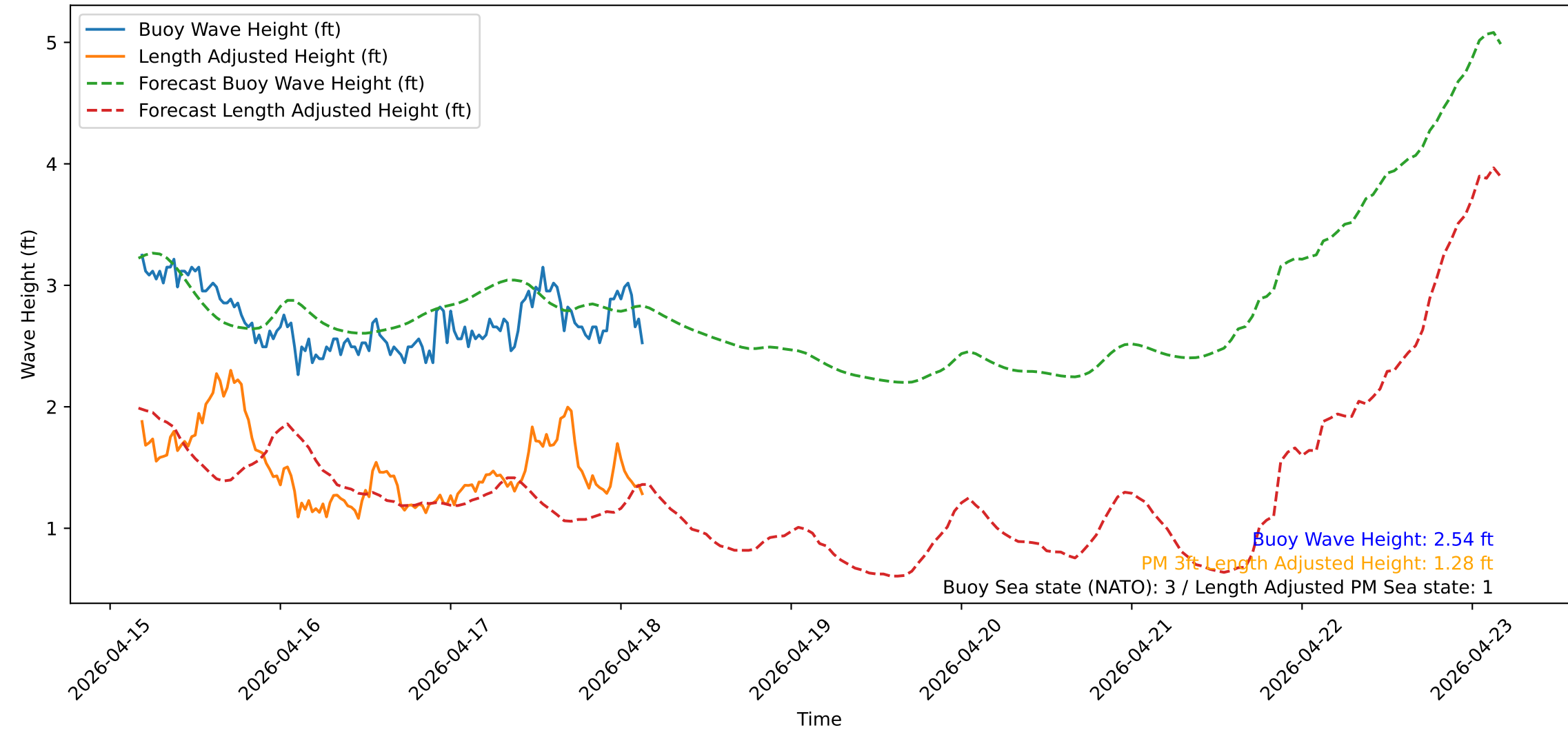
Wave Heights over Time for Red Beach at 2026-04-18 04:00:50
