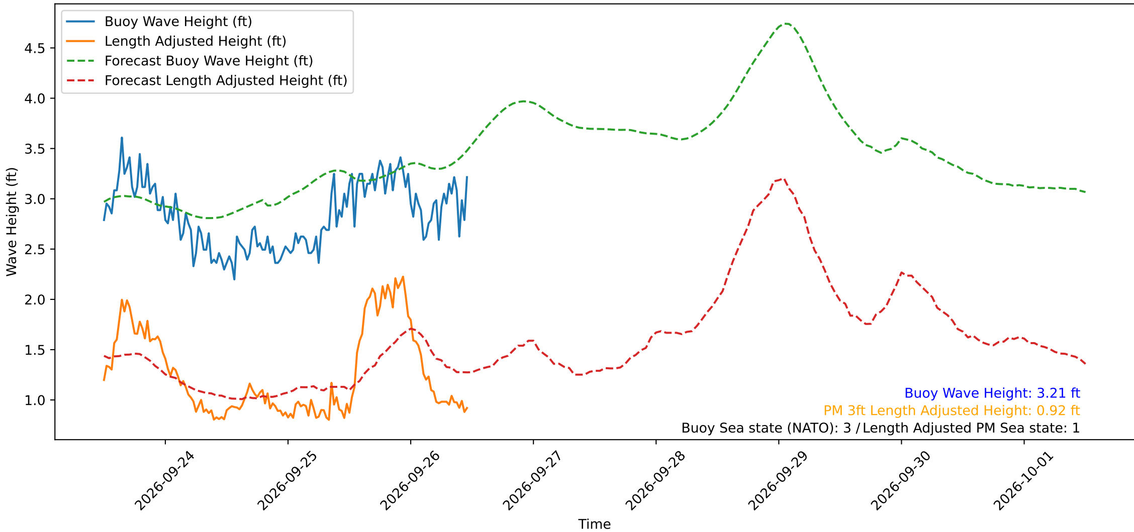
Wave Heights over Time for Oceanside Harbor at 2026-09-26 11:50:29
