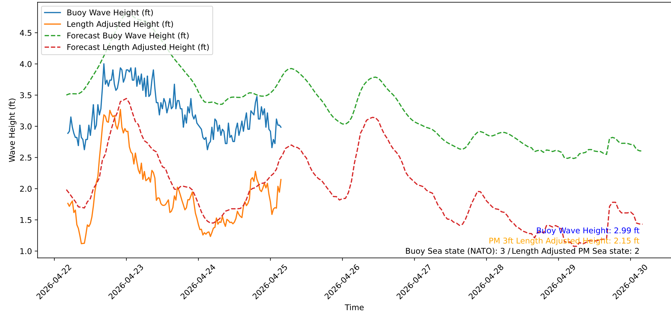
Wave Heights over Time for Green Beach at 2026-04-25 04:21:14
