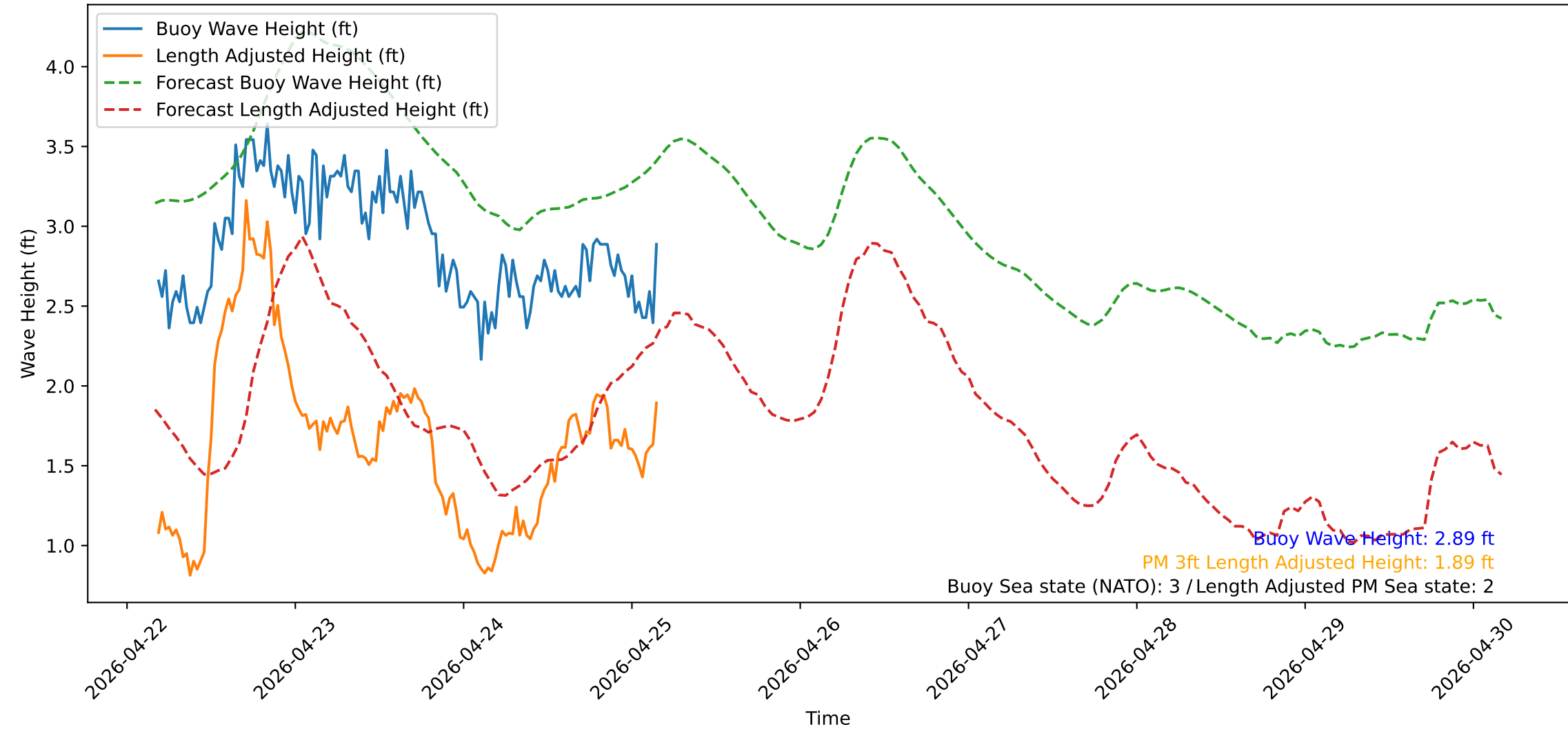
Wave Heights over Time for Red Beach at 2026-04-25 04:20:52
