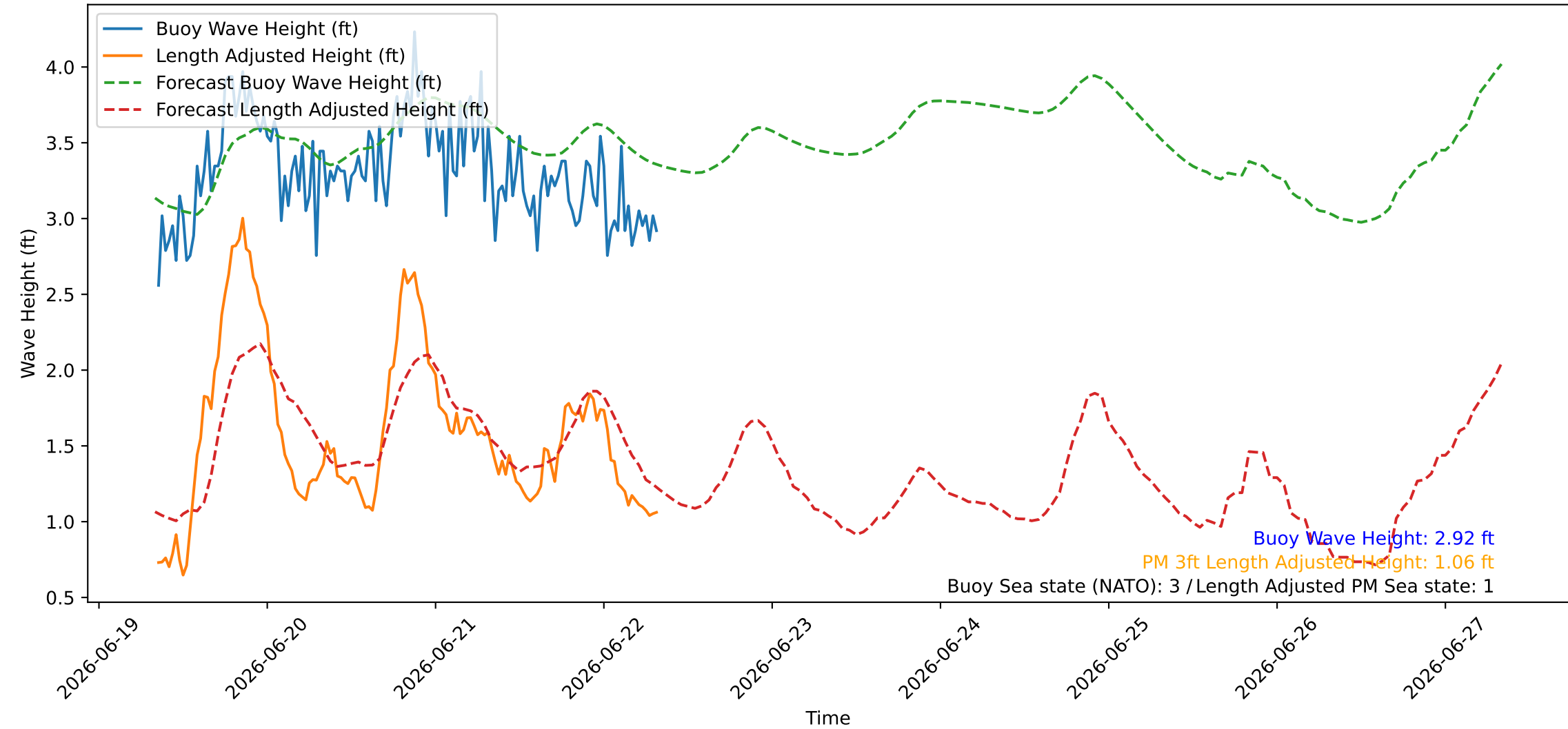
Wave Heights over Time for Green Beach at 2026-06-22 08:21:09
