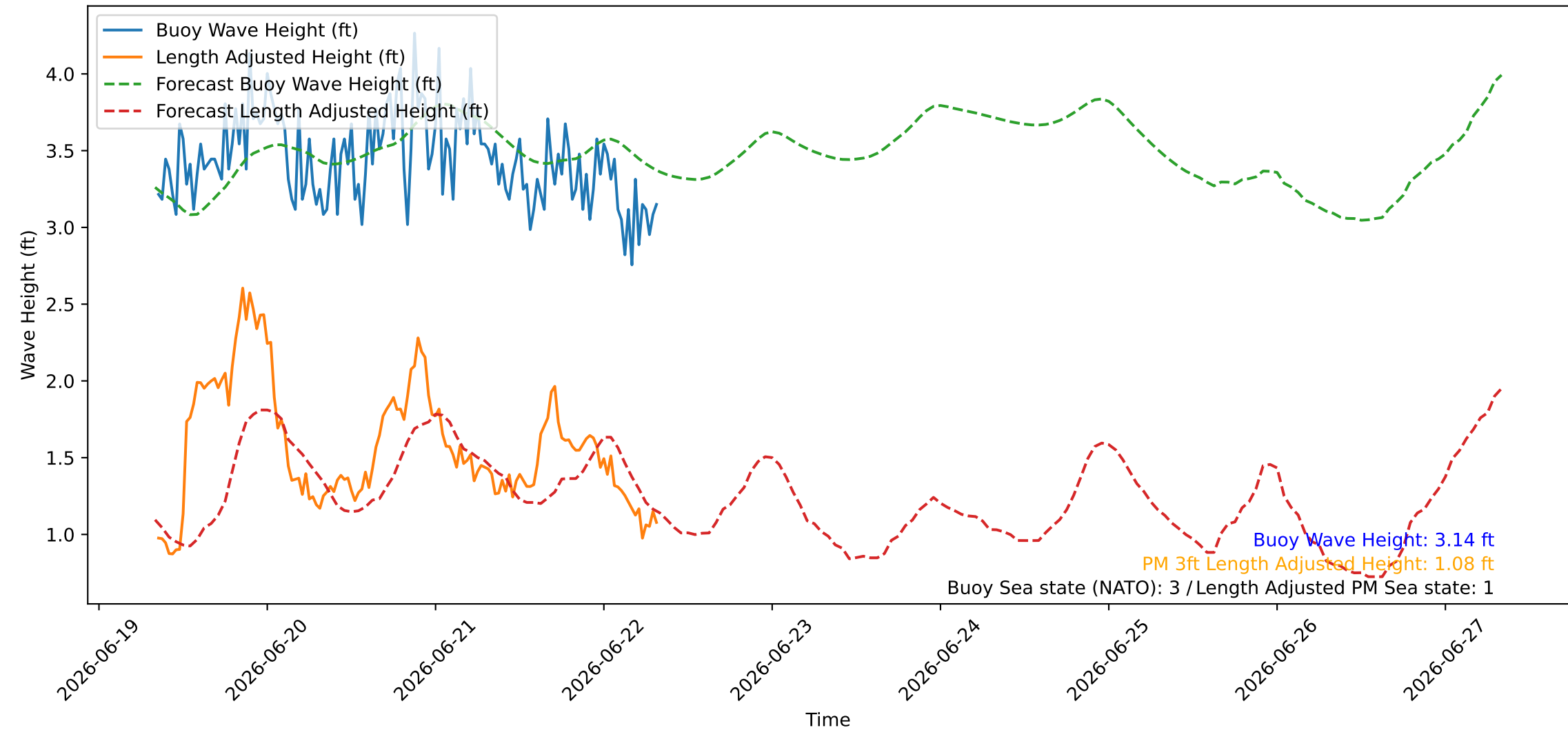
Wave Heights over Time for Oceanside Harbor at 2026-06-22 08:20:26
