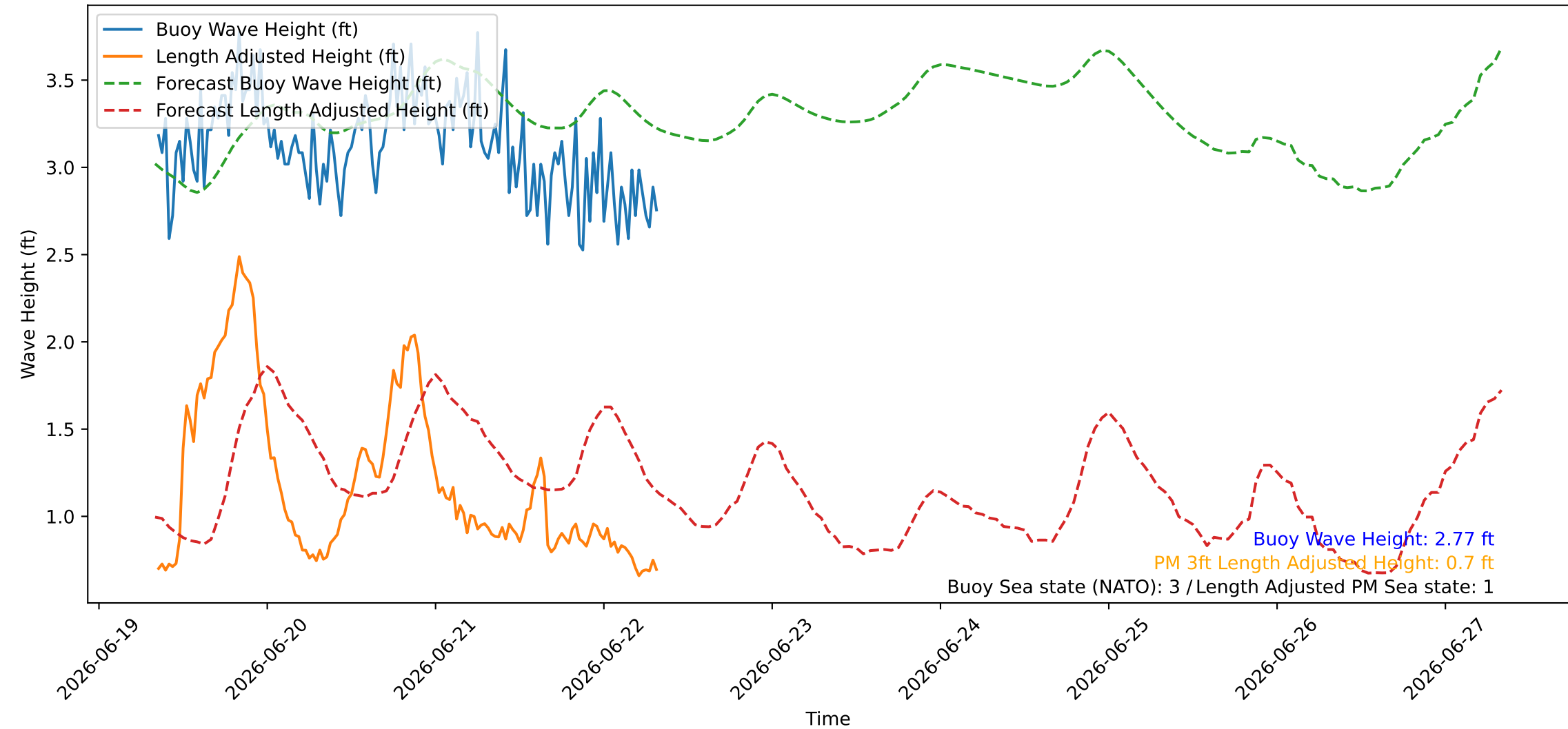
Wave Heights over Time for Red Beach at 2026-06-22 08:20:47
