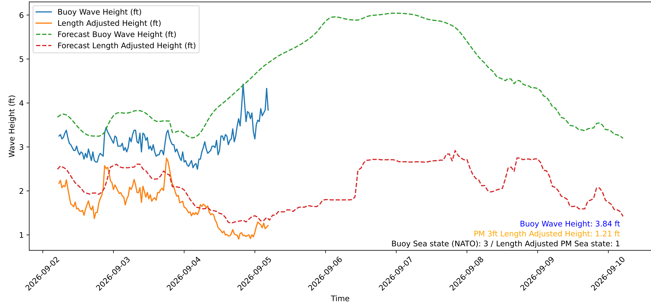
Wave Heights over Time for Green Beach at 2026-09-05 05:11:13
