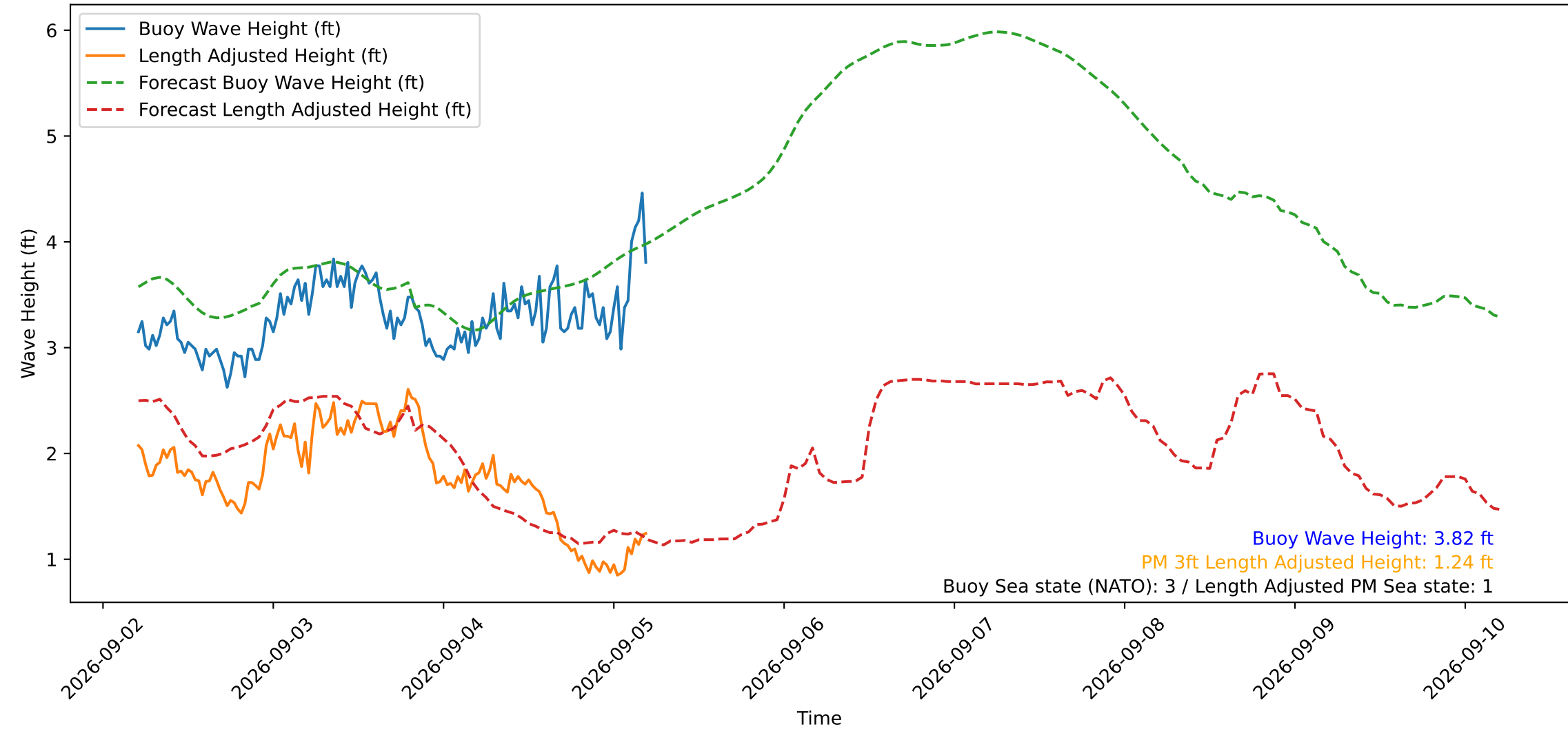
Wave Heights over Time for Oceanside Harbor at 2026-09-05 05:10:30
