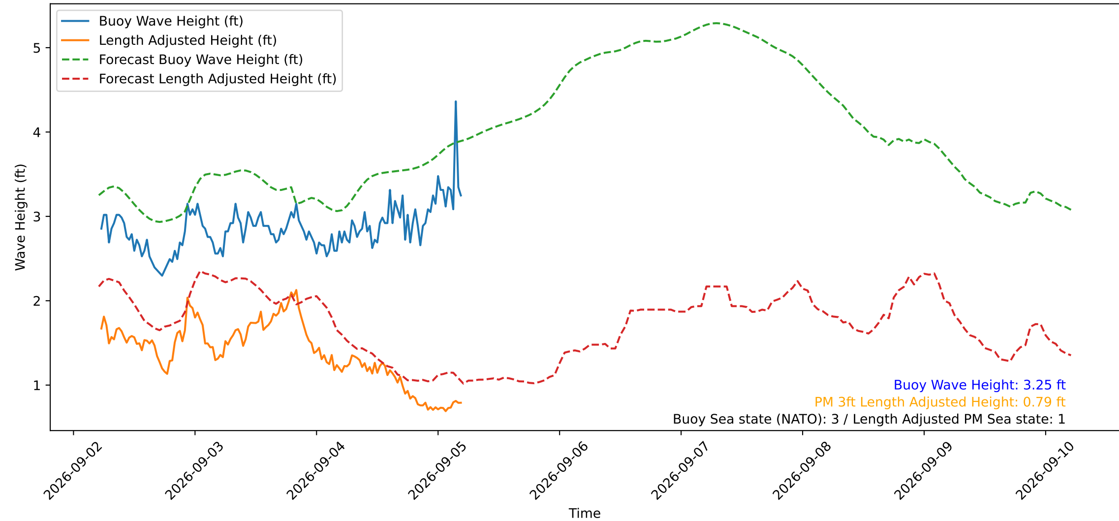
Wave Heights over Time for Red Beach at 2026-09-05 05:10:50
