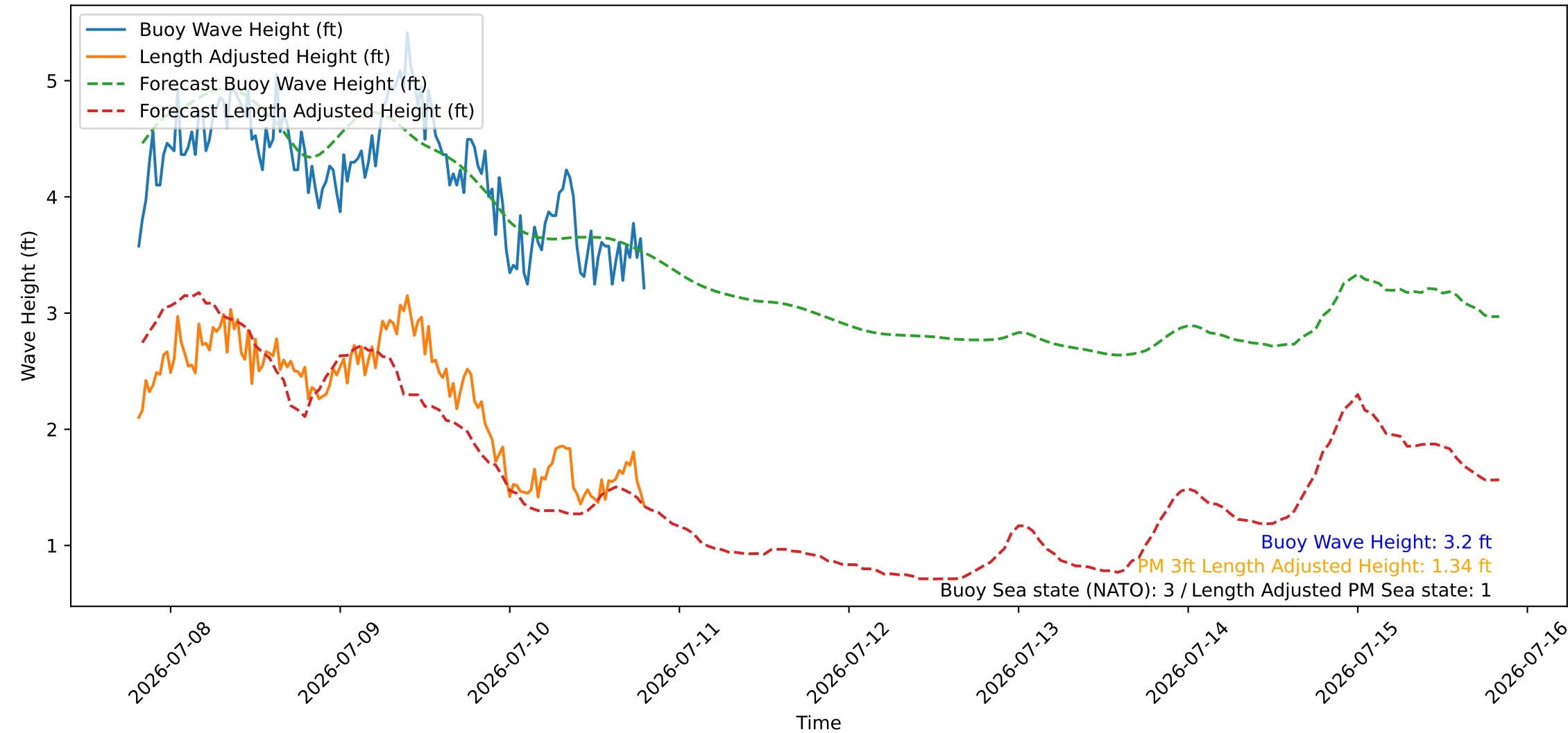
Wave Heights over Time for Oceanside Harbor at 2026-07-10 19:30:27
