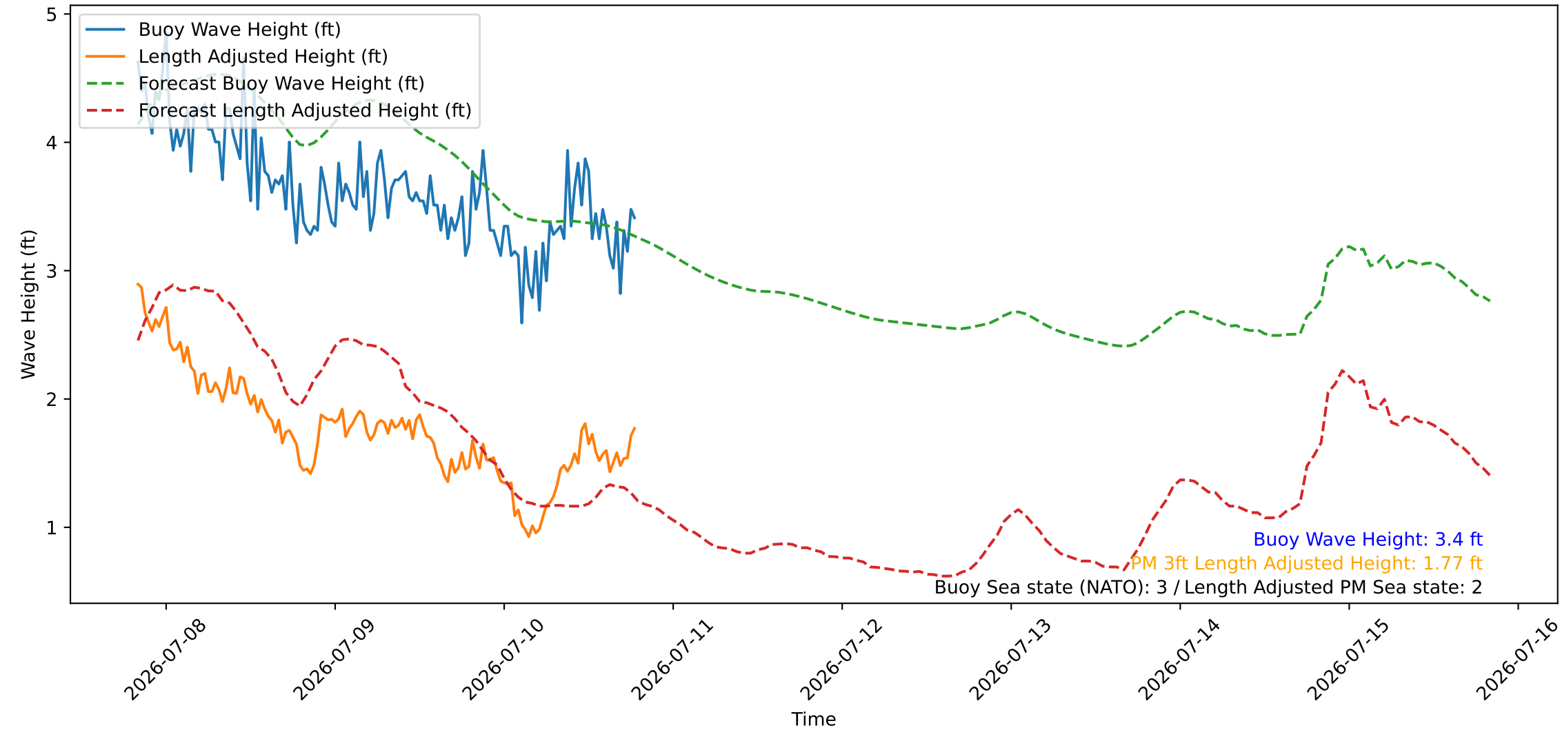
Wave Heights over Time for Red Beach at 2026-07-10 19:30:47
