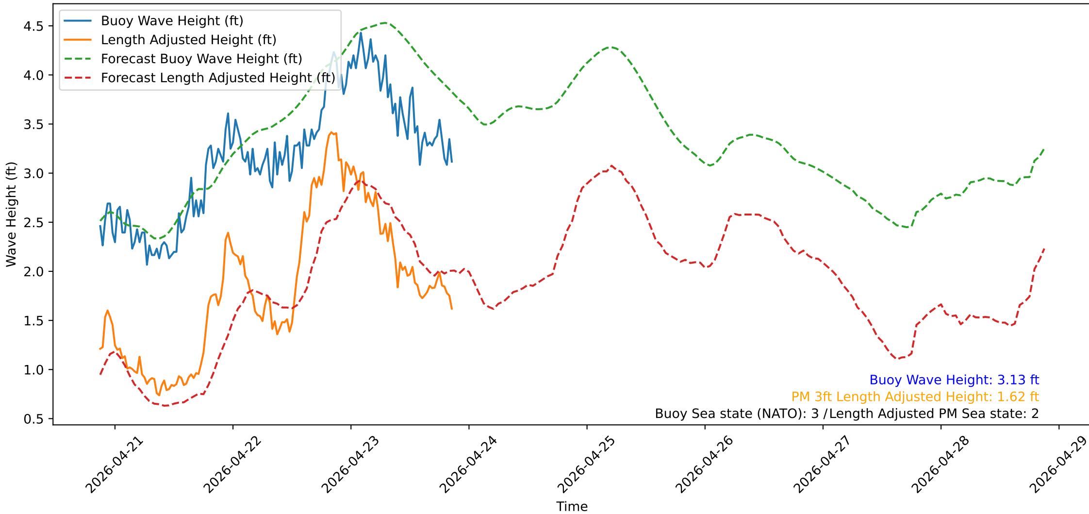
Wave Heights over Time for Oceanside Harbor at 2026-04-23 21:00:31
