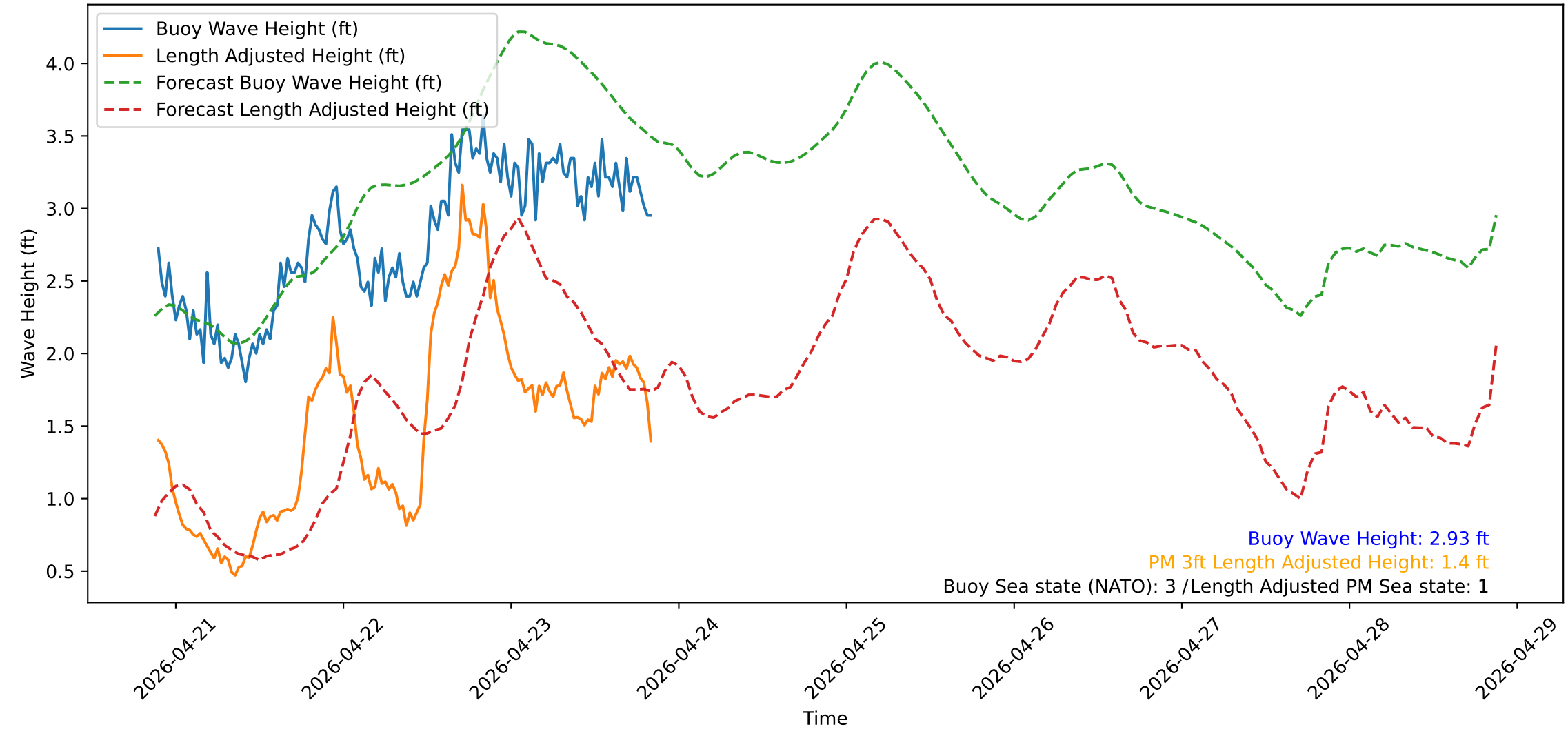
Wave Heights over Time for Red Beach at 2026-04-23 21:00:50
