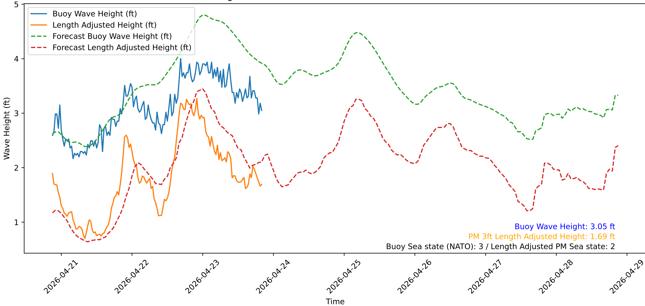
Wave Heights over Time for Green Beach at 2026-04-23 21:01:12
