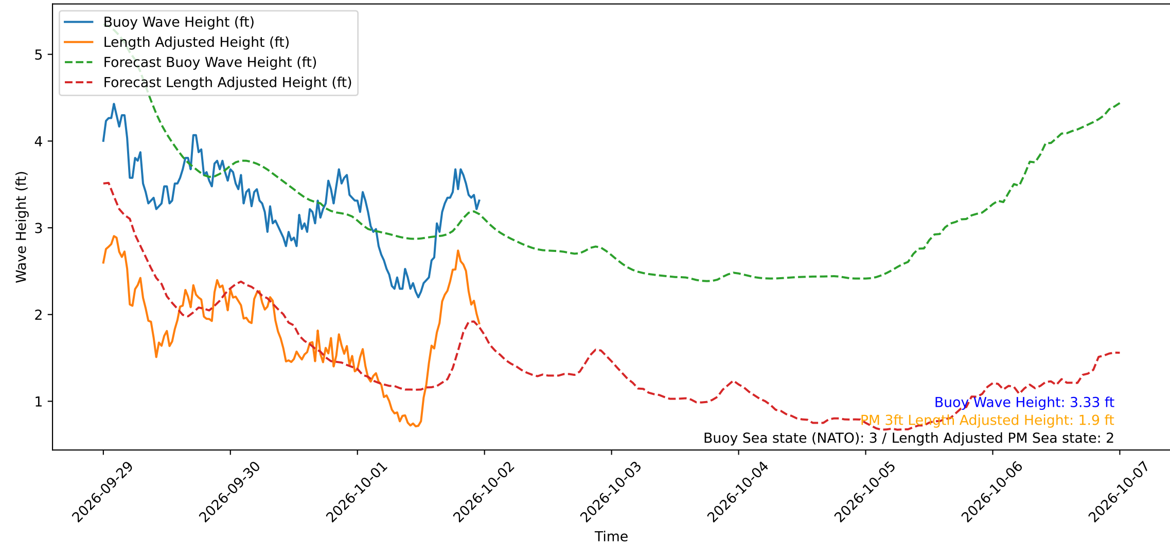
Wave Heights over Time for Green Beach at 2026-10-01 23:41:12
