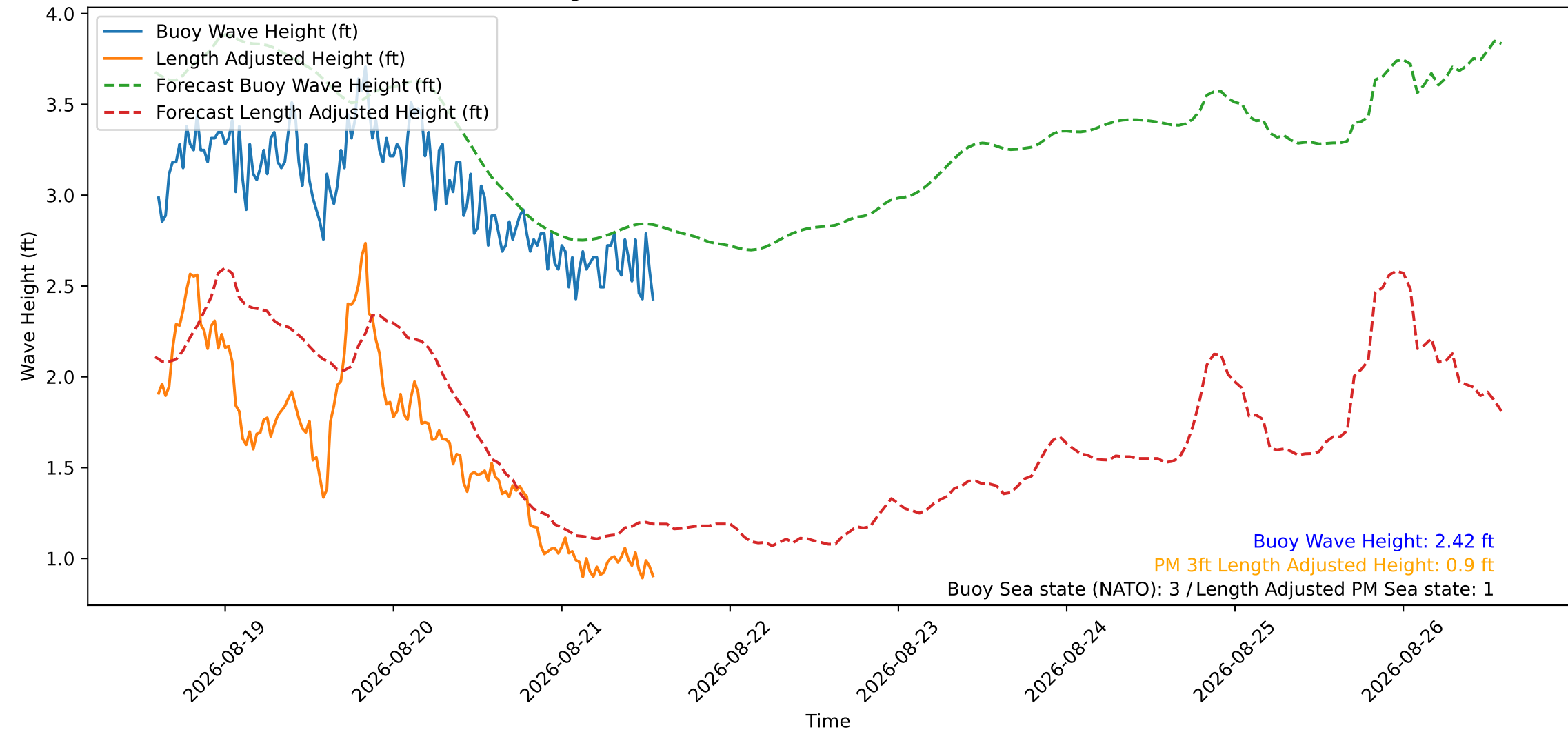
Wave Heights over Time for Green Beach at 2026-08-21 14:01:09
