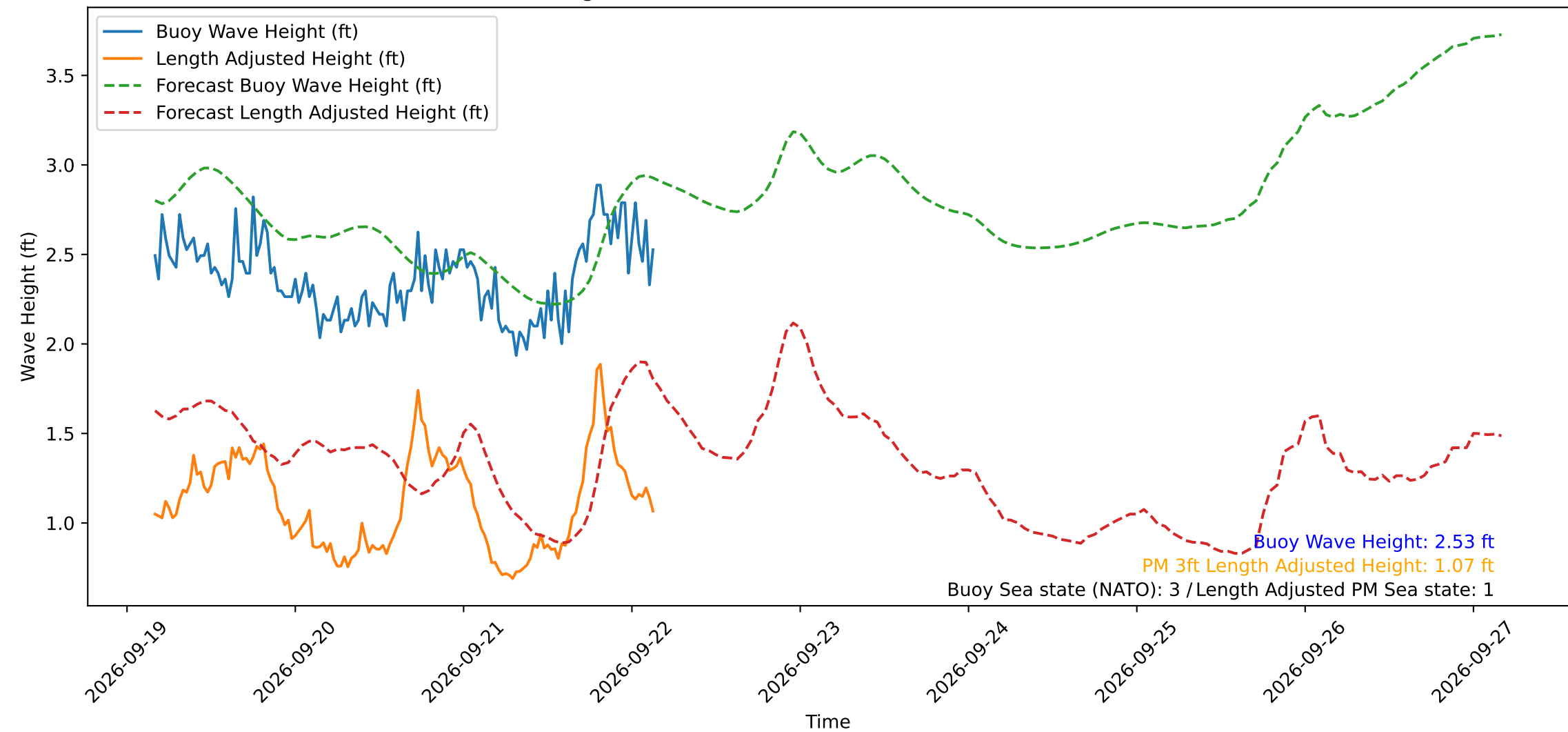
Wave Heights over Time for Red Beach at 2026-09-22 03:50:51
