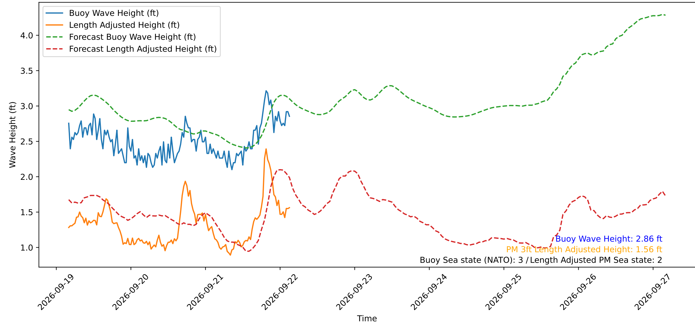
Wave Heights over Time for Oceanside Harbor at 2026-09-22 03:50:30
