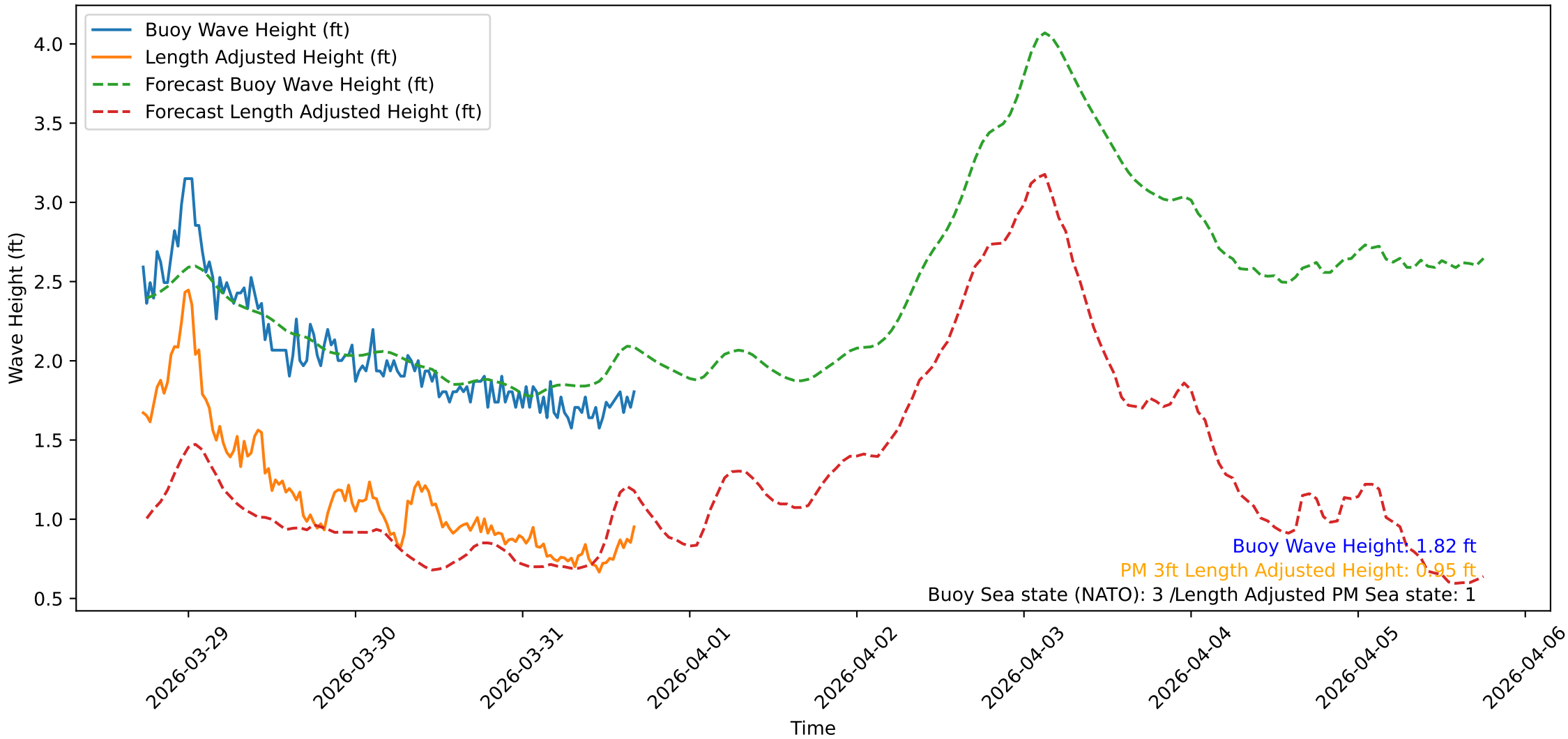
Wave Heights over Time for Oceanside Harbor at 2026-03-31 17:40:31
