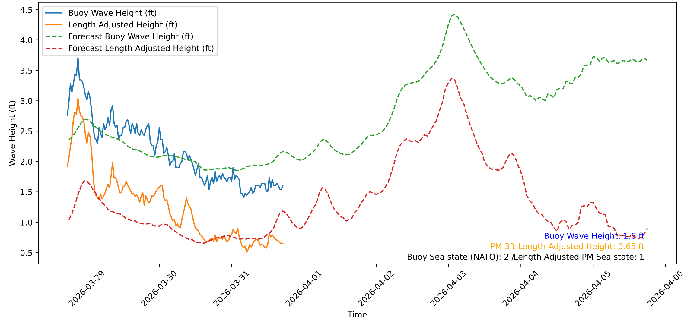
Wave Heights over Time for Green Beach at 2026-03-31 17:41:09
