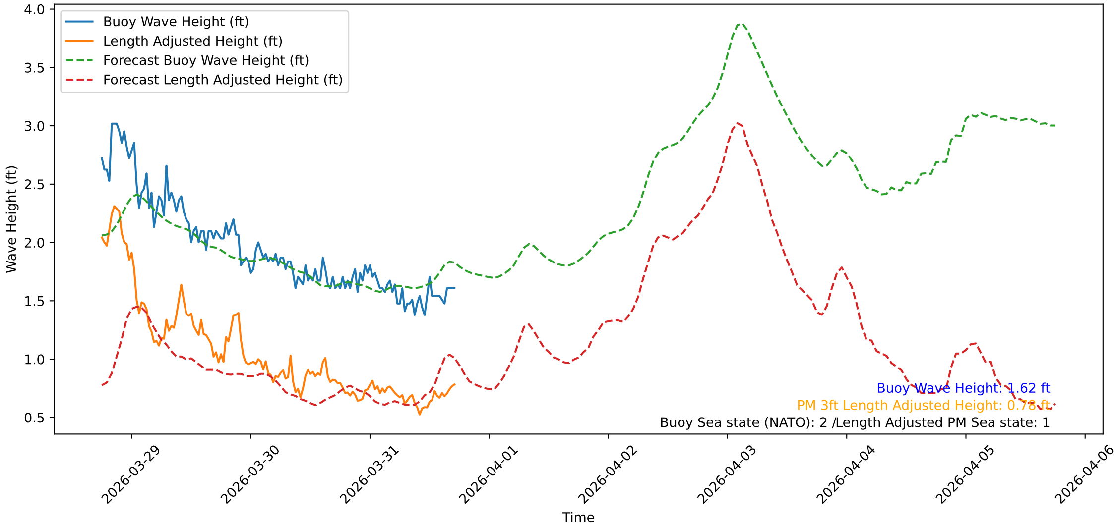
Wave Heights over Time for Red Beach at 2026-03-31 17:40:47
