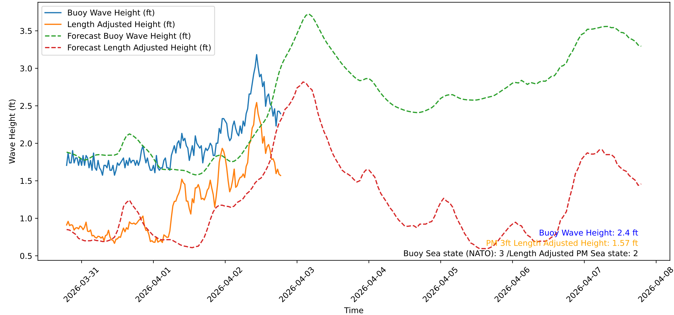
Wave Heights over Time for Oceanside Harbor at 2026-04-02 19:00:31
