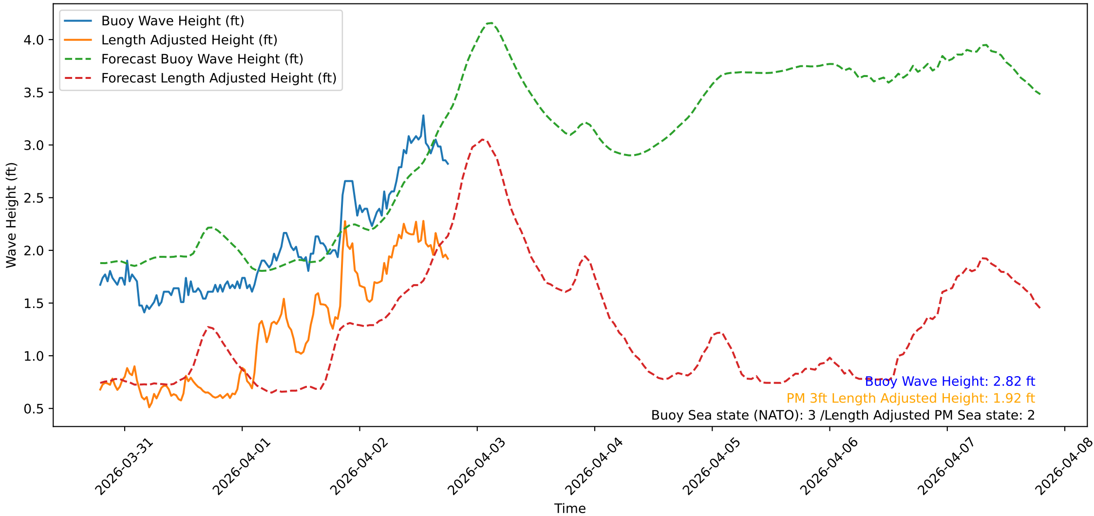
Wave Heights over Time for Green Beach at 2026-04-02 19:01:09
